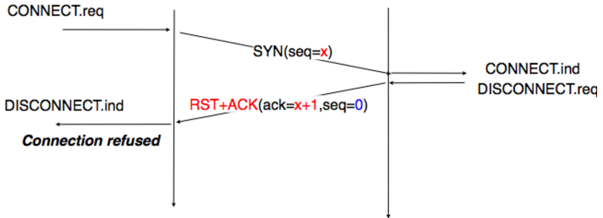
Fig. 23: TCP connection establishment rejected by peer
