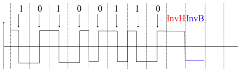
Fig. 2: Manchester encoding
