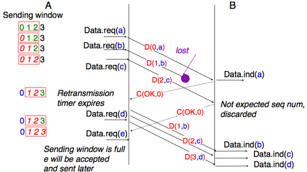
Fig. 13: Go-back-n : example
