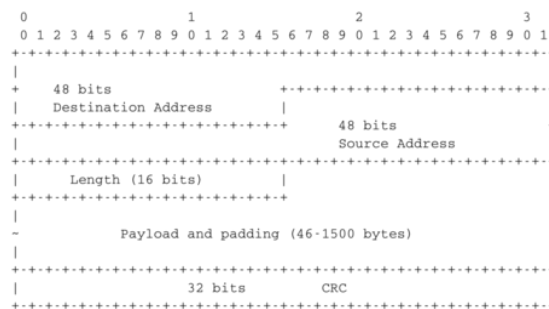
Fig. 83: Ethernet 802.3 frame format
