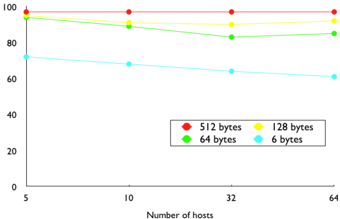
Fig. 81: Impact of the frame length on the maximum channel utilisation [SH1980]
