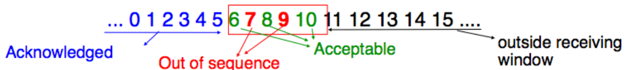
Fig. 14: The receiving window with selective repeat
