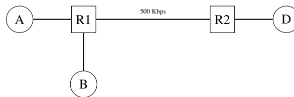
Fig. 83: A simple network with hosts sharing a bottleneck link
