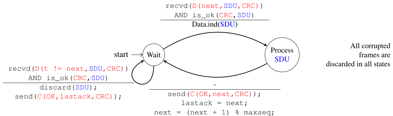
Fig. 11: Go-back-n: receiver FSM
