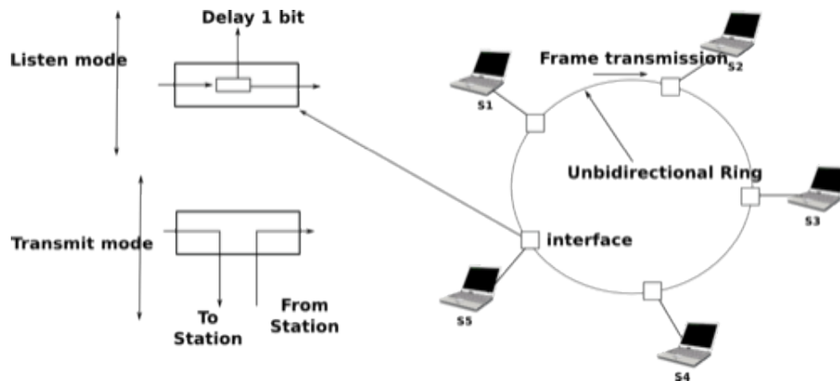
Fig. 74: A Token Ring network
