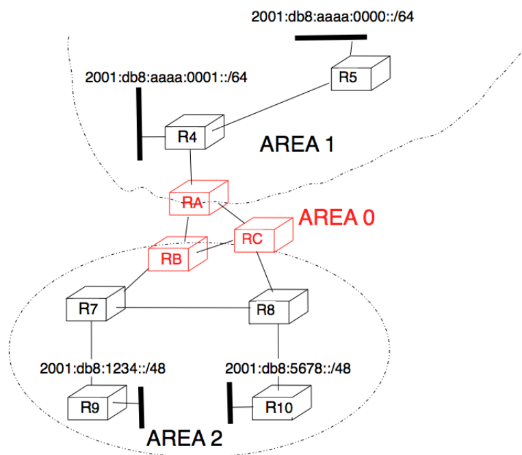
Fig. 62: Hierarchical routing with OSPF
