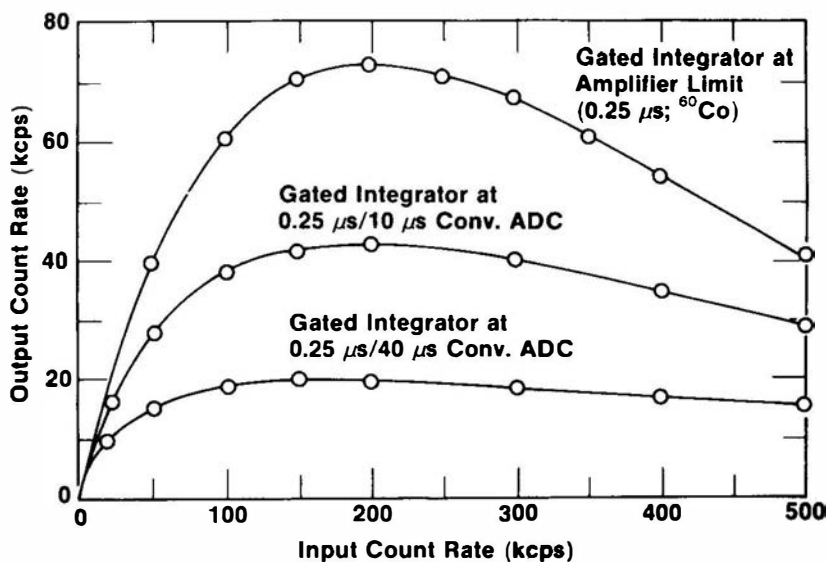
Figure 17.37 An example of the throughput of a pulse-processing system at high input rates. In this case, a gated integrator allows the use of a short (0.25 \mu\text{s} ) Gaussian shaping time. The top curve is for the amplifier alone. The remaining plots show the additional losses due to the conversion time of the ADC of the multichannel analyzer used to record the pulses. (From Britton et al., IEEE Trans. Nucl. Sci. NS-31(1) , 455 (1984).)
