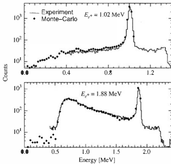
Figure 13.20 Response of a silicon detector with 2-mm depletion depth to monoenergetic positrons with the indicated energies. (From Frommhold et al. 46 )
