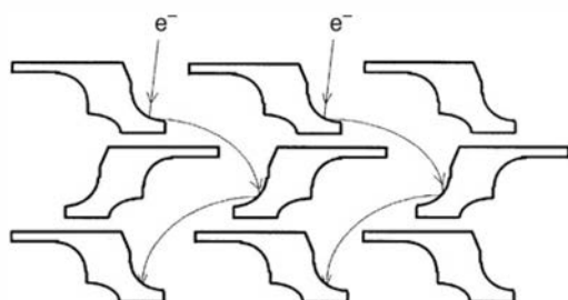
Figure 9.26 Cross section of a metal channel dynode structure. (From Yoshizawa and Takeuchi. 117 )
