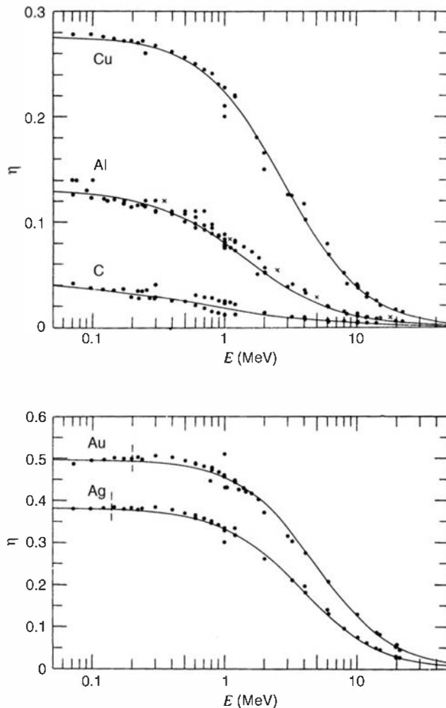
Figure 2.17 Fraction \eta of normally incident electrons that are backscattered from thick slabs of various materials, as a function of incident energy E . (From Tabata et al. 28 )
