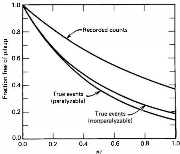
Figure 17.33 The fraction of recorded counts (upper curve) and true events (lower two curves) that escape pile-up as a function of true event rate n .
