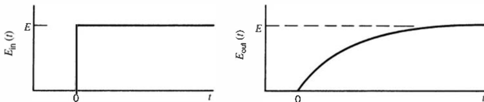
Figure 17.3 A low-pass RC filter or integrator network. The response to a step function input is illustrated.
