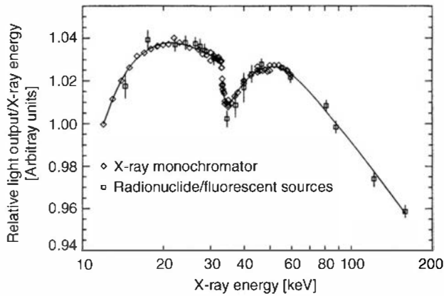
Figure 10.24 Measured light output per unit deposited energy for NaI(Tl), normalized to unity at 88 keV. (From Wayne et al. 34 )
