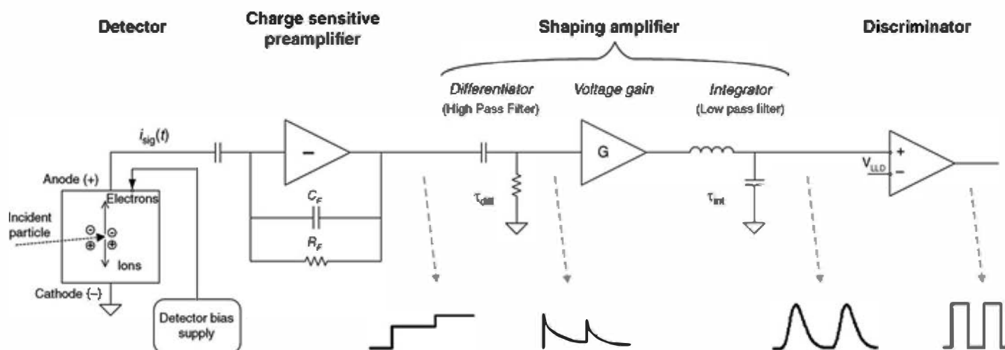
Figure 16.2 Schematic of simple signal processing electronics. This circuit is suitable for use, as shown, in many applications and is conceptually similar to more complex circuits. These elements are discussed in greater detail in Chapter 17. (Courtesy of R. Redus, Amptek, Inc.)
