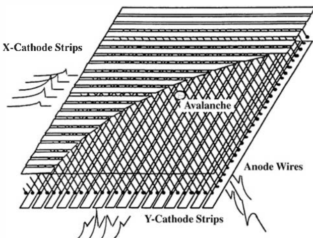
Figure 6.22 Sketch of a two-dimensional position-sensing multiwire proportional counter. (From Sauli. 108 )
