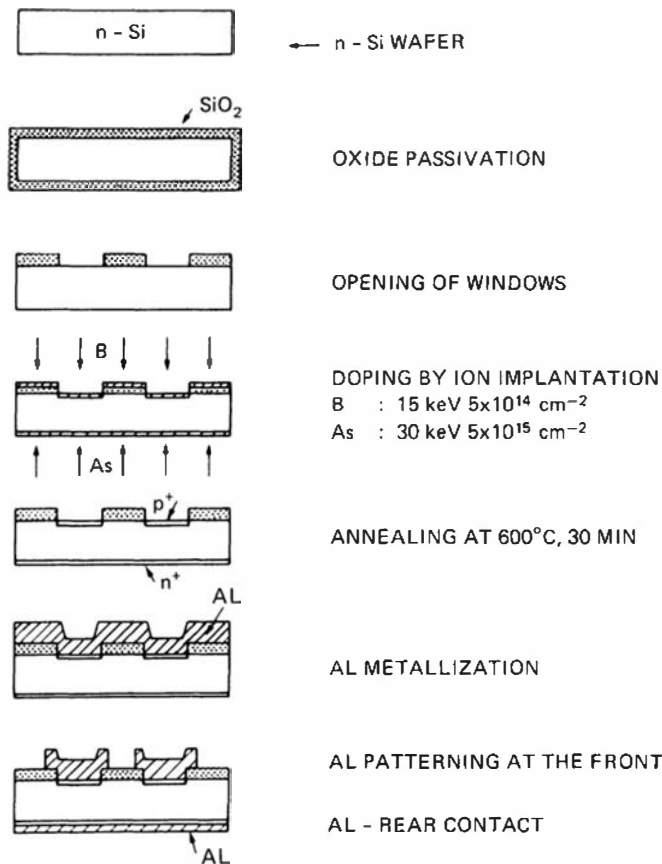
Figure 11.14 Steps in the fabrication of passivated planar silicon diode detectors. (From Kemmer. 38 )
