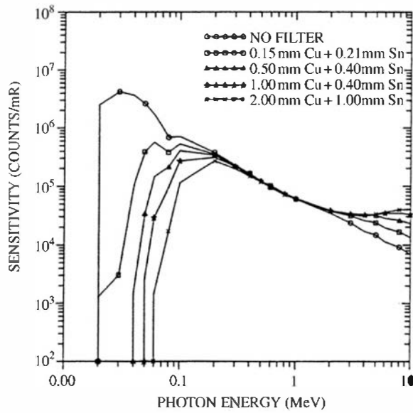
Figure 11.20 Calculated sensitivities (in counts/mR) of a typical photodiode to X- or gamma-ray photons as a function of their energy. Plots are shown for the bare photodiode as well as for the cases in which filters of the composition and thicknesses shown were included. (From Chen et al. 125 )
