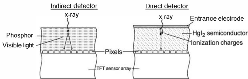
Figure 13.42 Schematic cross section of TFT imaging detectors, showing indirect detection via optical photons and direct charge detection using a semiconductor layer. (Adapted from Hartsough et al. 207 )
