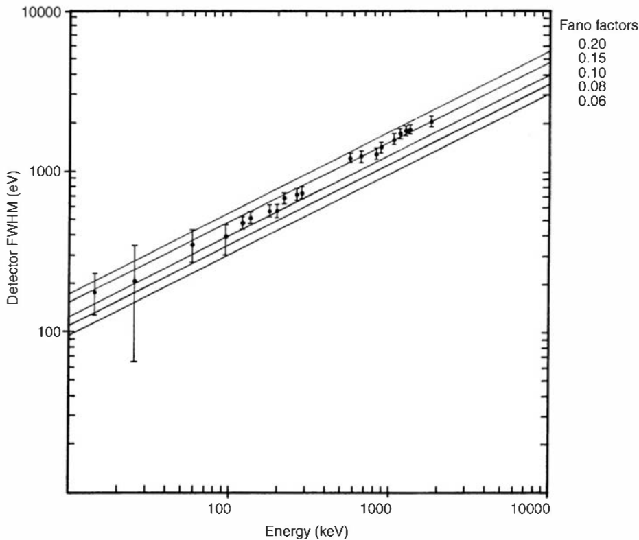
Figure 12.9 The measured statistical contribution W_D for an 8 mm diameter \times 4 mm planar Ge(Li) detector. Lines are shown corresponding to various assumed values for the Fano factor. (From Palms et al. 14 )
