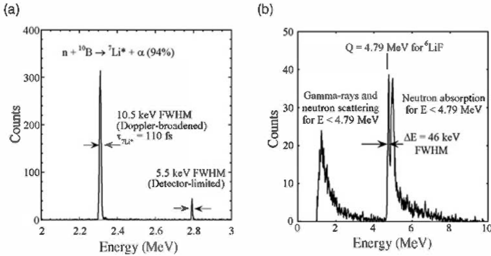
Figure 19.10 (a) Thermal neutron detection 78 in a \text{TiB}_2 absorber using a Mo/Cu TES on a SiN membrane. The two peaks correspond to the different Q values for the ground state and first excited state of {}^7\text{Li} . (b) Fast-neutron spectrum of a {}^{252}\text{Cf} source from a TES detector with an enriched {}^6\text{LiF} absorber. 80
