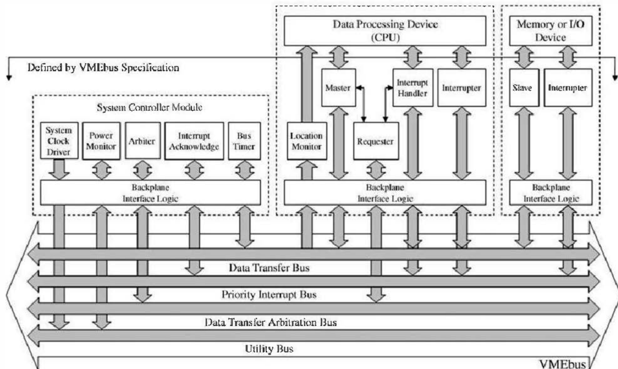
Figure A.3 Functional modules and busses defined by the VMEbus standard. (Adapted from IEEE Standard 1014-1987 for A Versatile Backplane Bus: VMEbus , New York, NY.)
