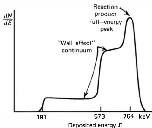
Figure 14.6 Expected pulse height spectrum from a {}^3\text{He} tube in which the wall effect is significant.
