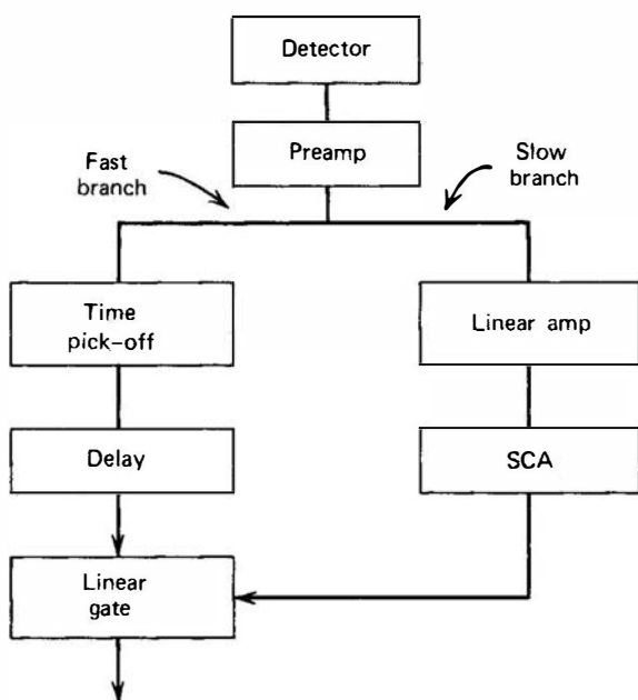
Figure 17.63 A simple fast-slow pulse-processing system in which a slow amplitude branch is used to select only those fast timing pulses that correspond to events of a predetermined amplitude set by the SCA window.
