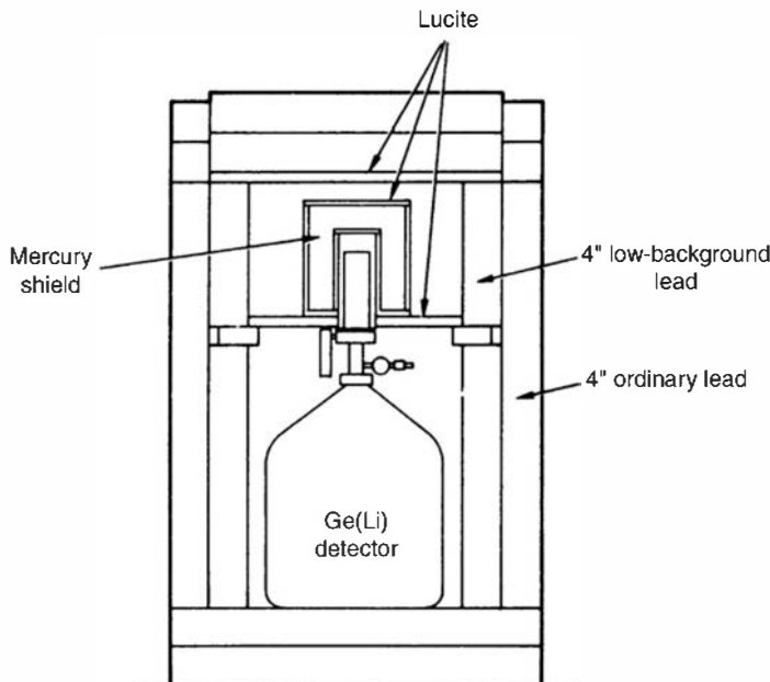
Figure 20.4 A low-background shield configuration for a germanium detector. (From Kaye et al. 16 )
