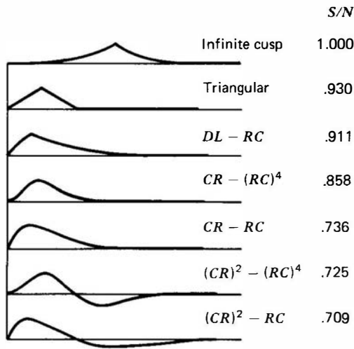
Figure 17.24 Various pulse shapes and their signal-to-noise ratio (S/N) relative to the infinite cusp. Various time constants are chosen to yield minimum noise, and pulse shapes are normalized to constant height. (Reproduced with permission from Nuclear Electronics , by P. W. Nicholson. Copyright 1974, by John Wiley & Sons Ltd.)
