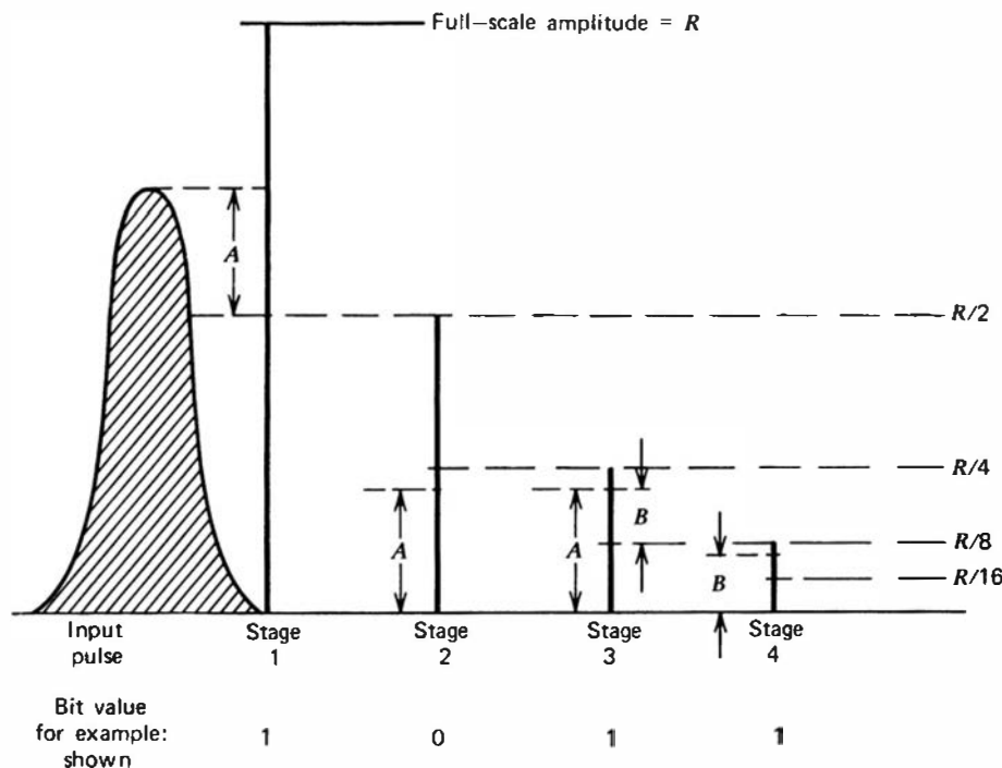
Figure 18.9 Illustration of the operational sequence for a successive approximation ADC. Four stages are shown that generate the four-bit word shown at the bottom as the digital output.
