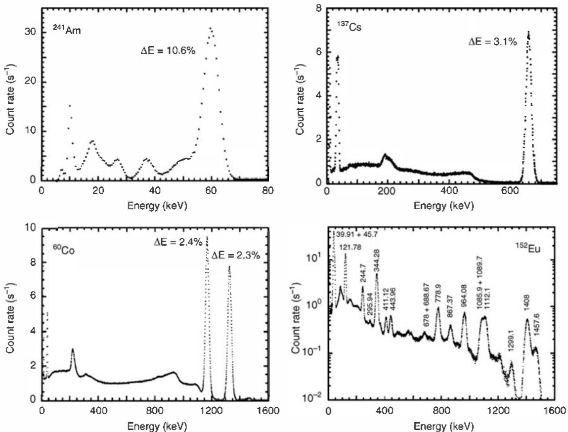
Figure 10.12 Pulse height spectra from a 2 in. × 2 in. LaBr 3 (Ce) scintillator. The better energy resolution is evident in comparison with the NaI(Tl) example for 60 Co in Fig. 10.13b. (From Quarati et al. 16 )
