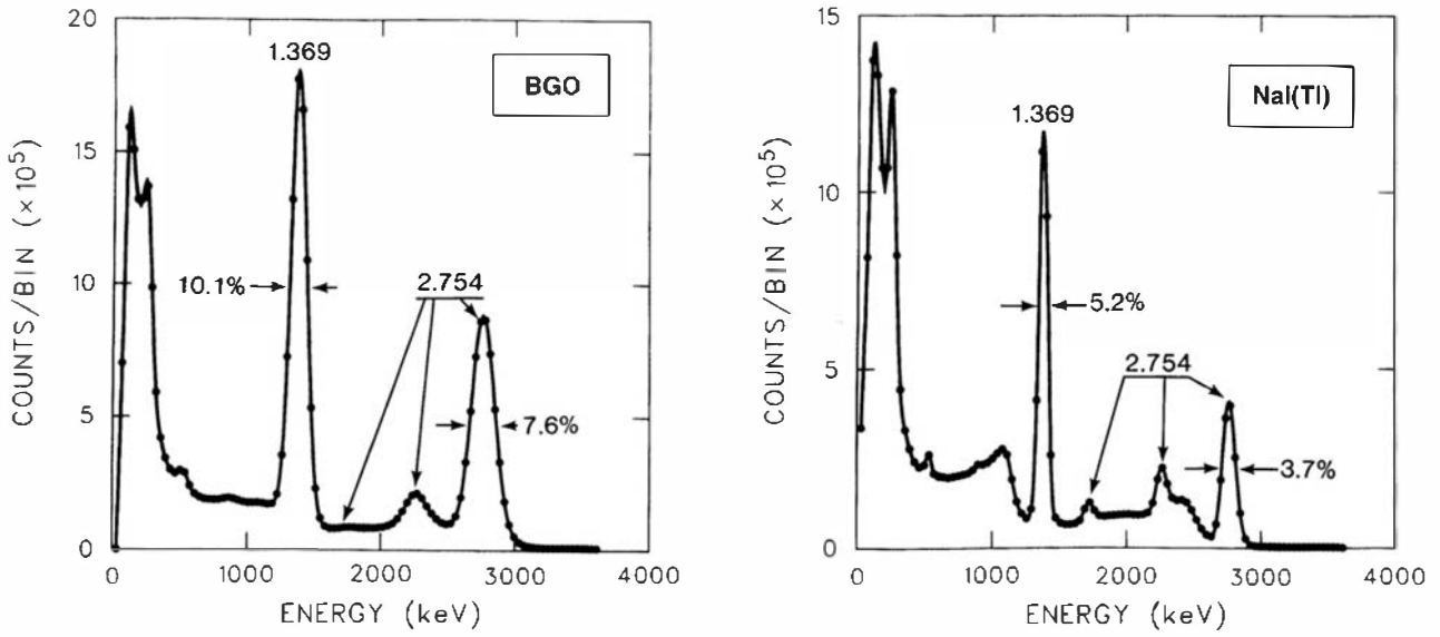
Figure 10.15 Comparative pulse height spectra measured for BGO (left) and NaI(Tl) (right) scintillators of equal 7.62 cm × 7.62 cm size for gamma rays from 24 Na. (From Moss et al. 14 )
