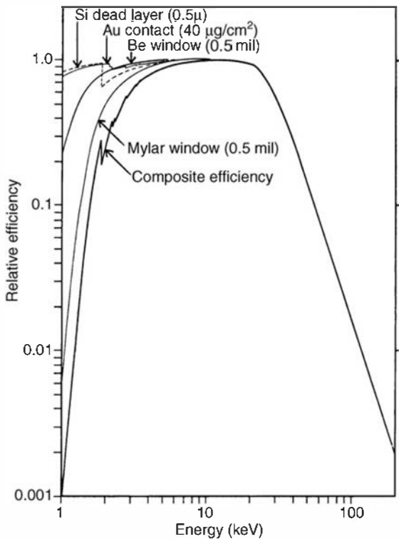
Figure 13.14 Calculated full-energy peak efficiency for a 3-mm-thick Si(Li) detector. (From Gallagher and Cipolla. 34 )
