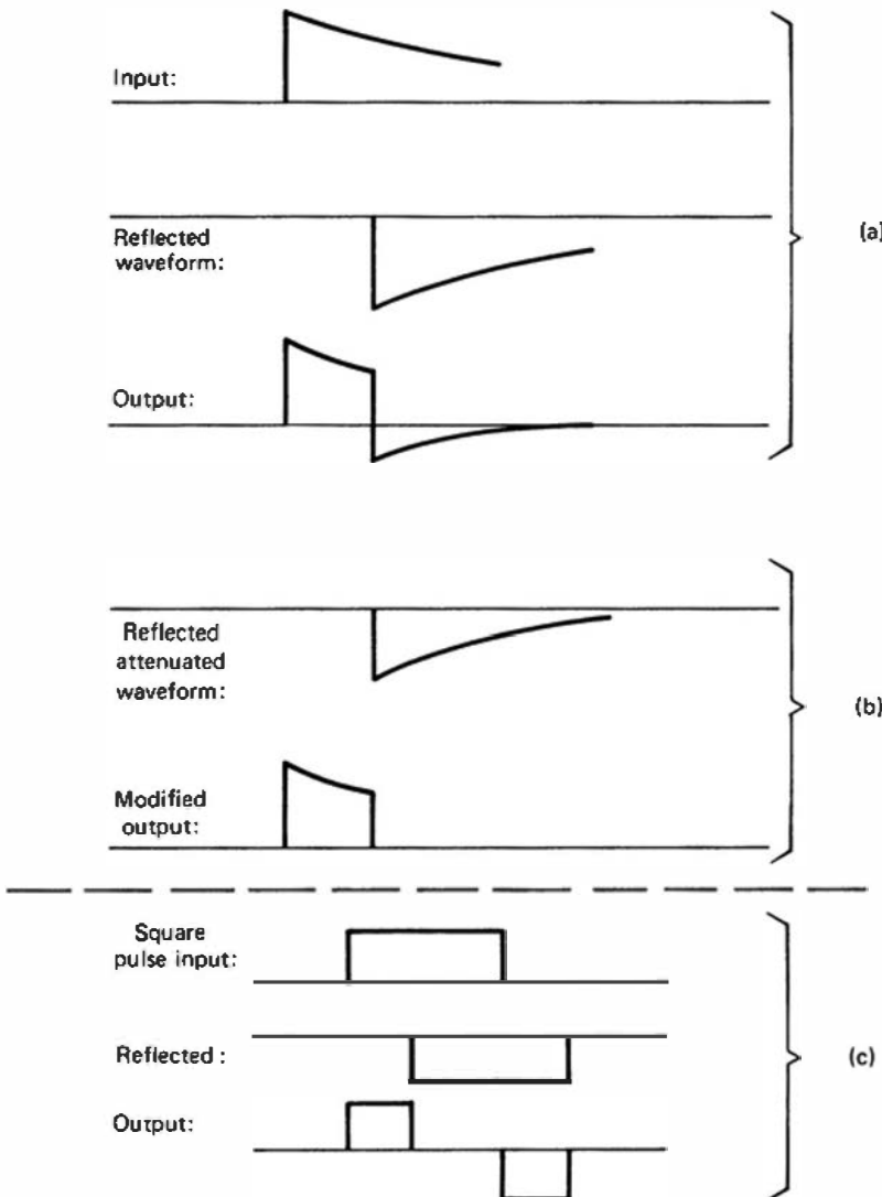
Figure 17.14 (a) Effect of applying simple SDL shaping to an input tail pulse with decay time comparable with the propagation time of a delay line. (b) Remedy to the undershoot of part (a) accomplished by partially attenuating the reflected waveform. (c) Effect of SDL shaping on a rectangular-shaped input pulse whose length exceeds the delay line down-and-back time.
