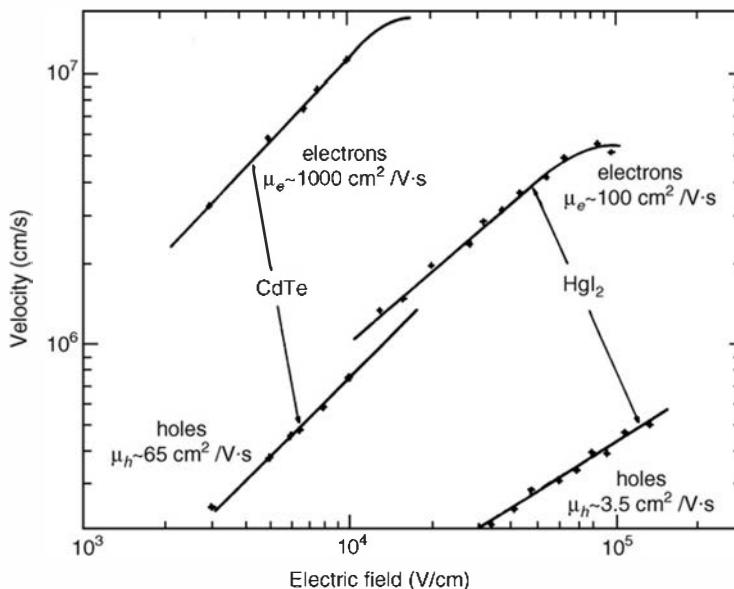
Figure 13.25 Drift velocity as a function of electric field strength for charge carriers in CdTe and HgI 2 . In both materials, holes are much less mobile than electrons. (From Scharager et al. 59 )
