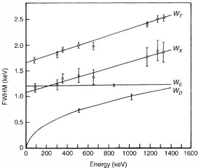
Figure 12.11 Example of the variation of the FWHM of the full-energy peak of an 86 cm 3 HPGe detector with gamma-ray energy. Each of the three terms in Eq. (12.12) is shown separately, together with the total FWHM. (From Owens. 16 )
