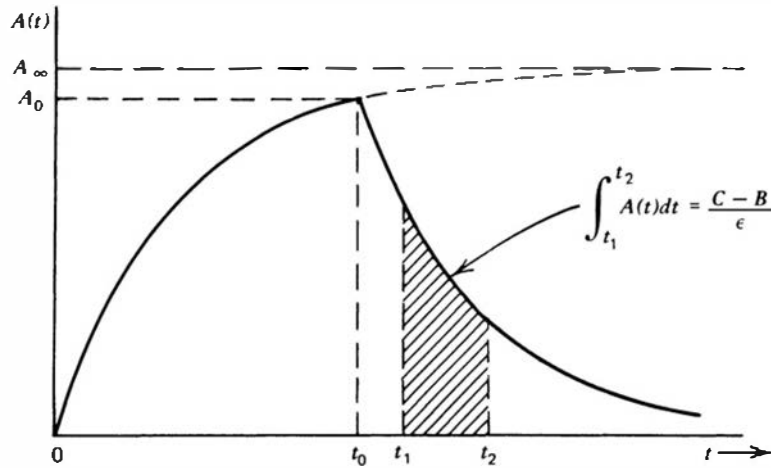
Figure 19.23 The activity of an activation detector after insertion in a constant neutron flux at time = 0 and removal at time = t_0 . The measured number of counts is proportional to the area under the decay curve between t_1 and t_2 . All times are measured from the start of irradiation at t = 0 .
