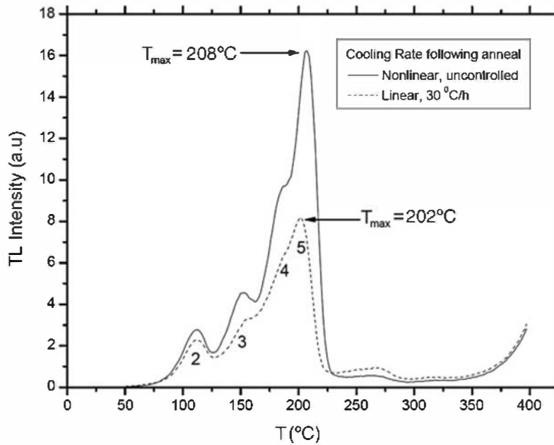
Figure 19.15 Glow curve of LiF:Mg,Ti (TLD-100). The main dosimetric peak 5 occurs at between 200 and 210°C if a linear heating rate of 2°C/s is employed. (Courtesy of Y. S. Horowitz, Ben Gurion Univ.)
