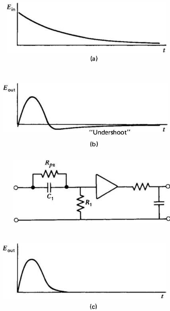
Figure 17.8 Application of pole-zero cancellation to eliminate the undershoot (b) normally generated by a CR - RC shaping network for an input step with finite decay time. By adding an appropriate resistance R_{pz} to the differentiator stage, a waveform without undershoot (c) can be obtained.
