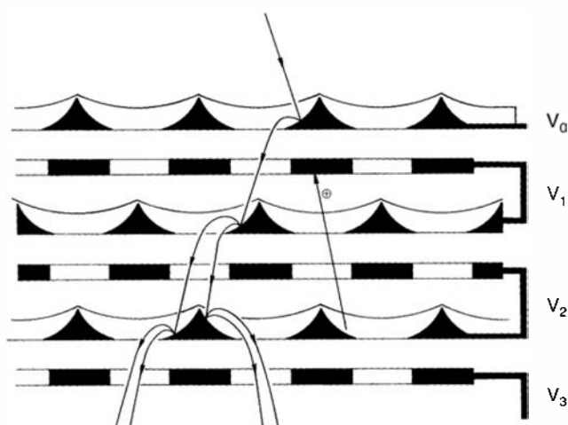
Figure 9.25 Cross section of a focused mesh electron multiplier. Each cusp-shaped dynode layer has an associated guard plate with its holes aligned over the points of the cusps. The guard plate helps focus the emitted secondary electrons onto the next dynode layer and also stops any secondary ions (the upward arrow shown) from causing ion feedback. (From Vallerga et al. 114 )
