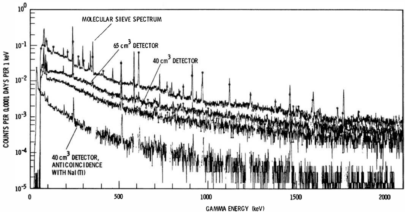
Figure 20.11 The bottom spectrum shows the degree to which background in a 40-cm 3 germanium detector may be suppressed through the use of an annular NaI(Tl) scintillator in anticoincidence. A comparison of the two middle spectra illustrates the increase in background with detector active volume. The top curve shows the recorded spectrum using a sample of molecular sieve (formerly a part of some germanium vacuum systems) as a source of natural background radiation. (From Kaye et al. 16 )
