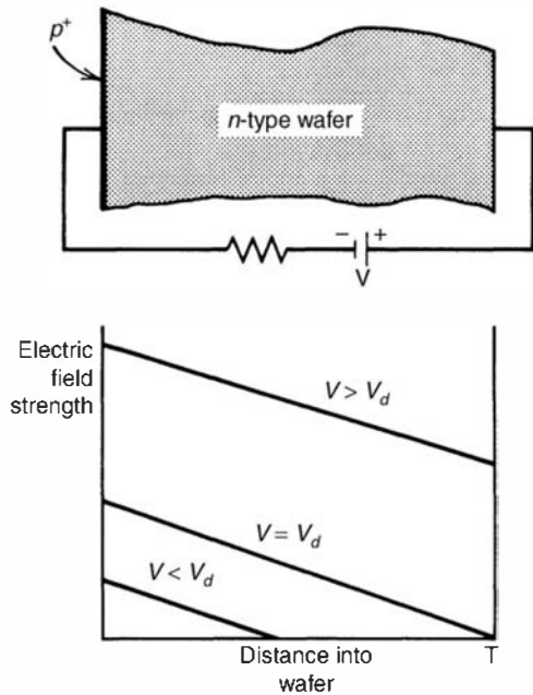
Figure 11.12 The electric field shape in a reverse bias semiconductor detector. Three plots are shown for bias voltages that are below, equal to, and above the depletion voltage V_d .
