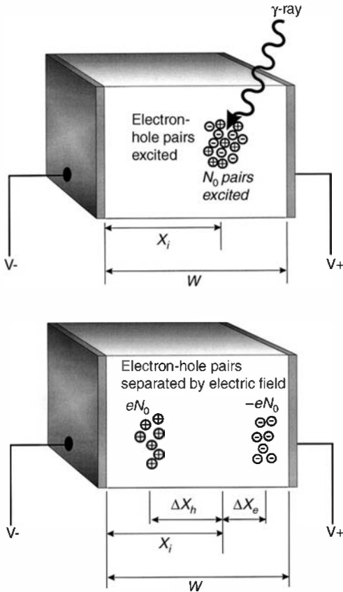
Figure 13.23 Basic operating configuration for a planar semiconductor detector. Electrons and holes are swept to their respective electrodes by an externally applied voltage. (From McGregor and Hermon. 50 )
