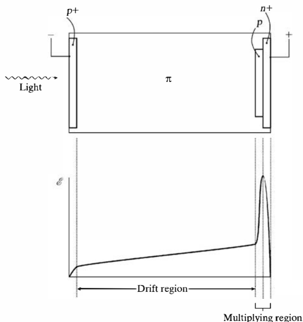
Figure 9.18 The reach-through configuration for an avalanche photodiode is sketched at the top of the figure. Below is a plot of the resulting electric field when a bias voltage is applied.
