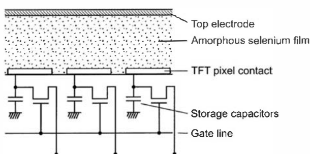
Figure 13.43 Amorphous silicon photoconductor layer coupled to a thin film transistor (TFT) readout array.
