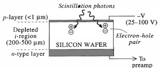
Figure 9.15 Basic configuration of a conventional photodiode.
