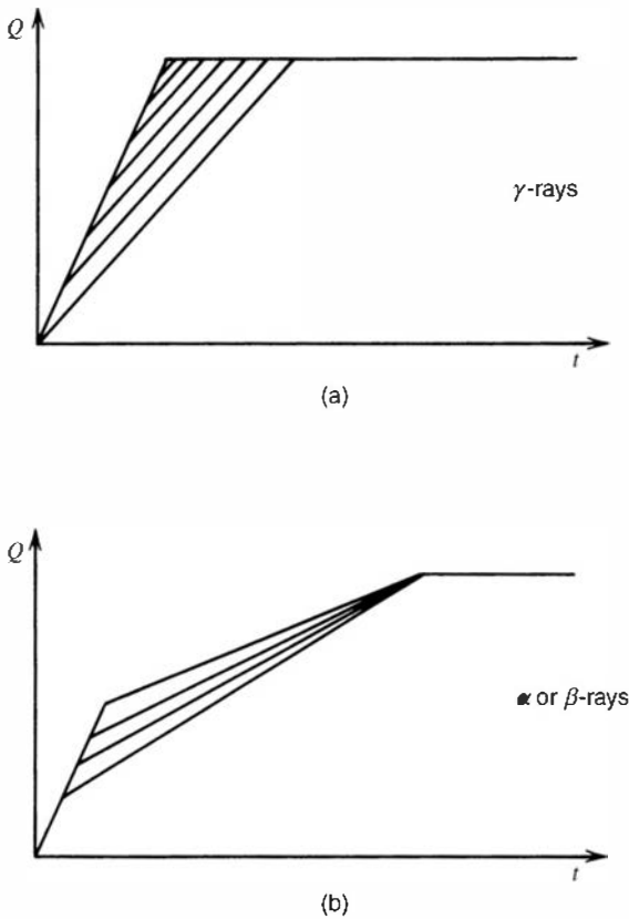
Figure 13.2 Simplified representation of the signal pulse leading edge for a Si(Li) detector. Variations arise from differences in the position of interaction within the detector active volume. (From Moszynski et al. 8 )
