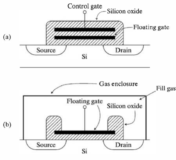
Figure 19.25 (a) Configuration of a nonvolatile memory cell (EEPROM). (b) The direct ion storage dosimeter (DIS) consisting of the combination of a gas-filled ion chamber and an EEPROM.
