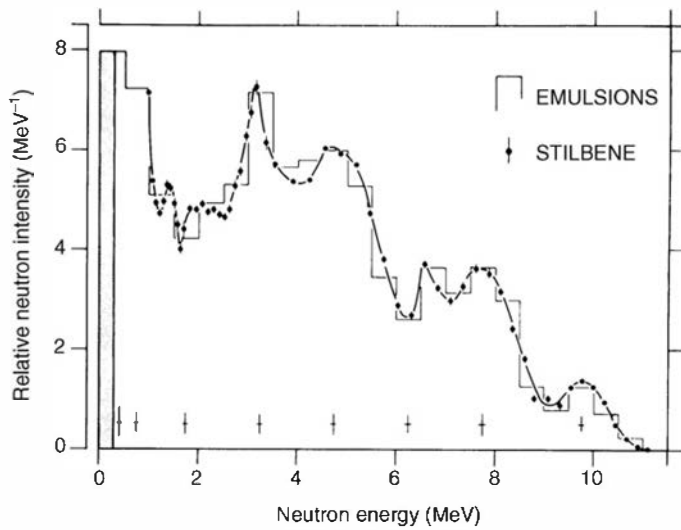
Figure 1.12 Measured energy spectra for neutrons from a ^{239}\text{Pu}/\text{Be} source containing 80 g of the isotope. (From Anderson and Neff. 26 )
