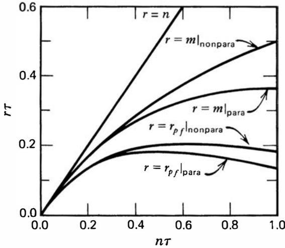
Figure 17.34 Variation of the recorded count rate ( m ) and the rate at which true events are recorded free of pile-up ( r_{pf} ) for both paralyzable and nonparalyzable systems. The true event rate is n and the pile-up resolution time is \tau .
