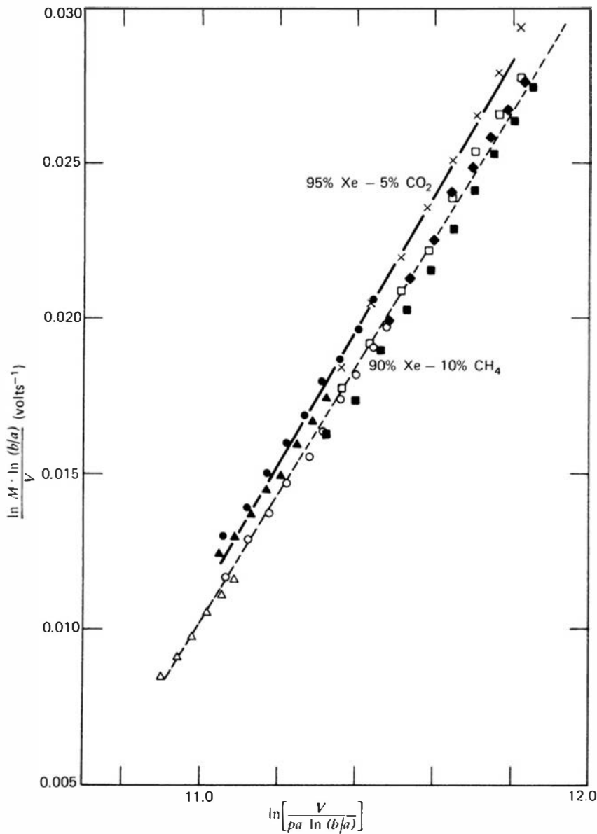
Figure 6.12 A Diethorn plot of the same data shown in Fig. 6.11. As predicted by Eq. (6.10), a graph of [\ln M \cdot \ln(b/a)/V] versus \ln [V/pa \ln(b/a)] for all counters using the same gas closely matches a straight line with slope of (\ln 2/\Delta V) and intercept (-\ln 2)(\ln K)/\Delta V . (From Hendricks. 51 )
