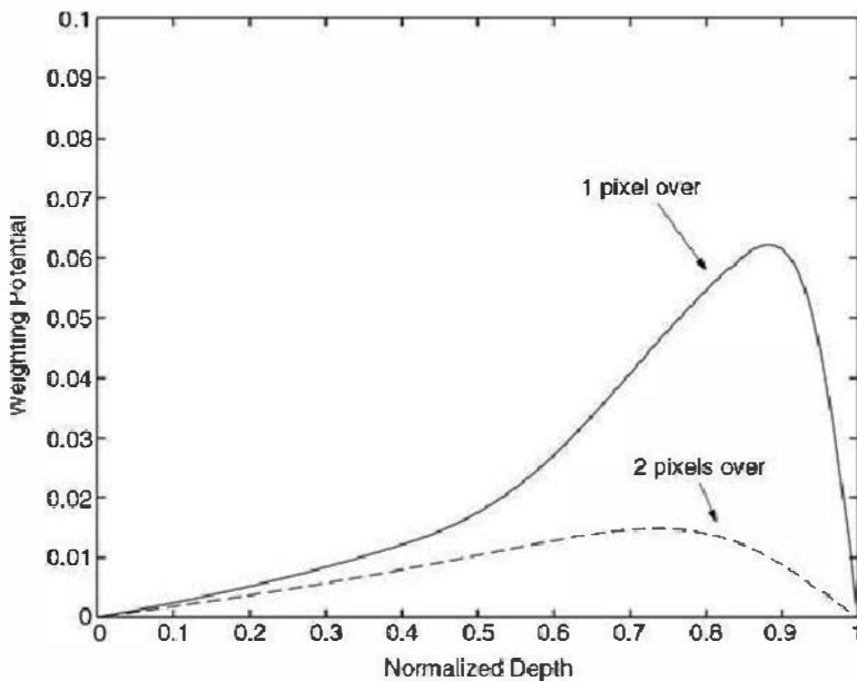
Figure D.3 The solid curve shows the weighting potential for Pixel #1 of Fig. D-1a along an axis that is perpendicular to the center of an adjacent pixel. The dashed line shows the same variation along the axis of a pixel that is located two pixels away. Both plots are for the case in which the pixel size is 20% of the detector thickness T . Note that the vertical scale is expanded by a factor of 10 compared with the previous two figures.
