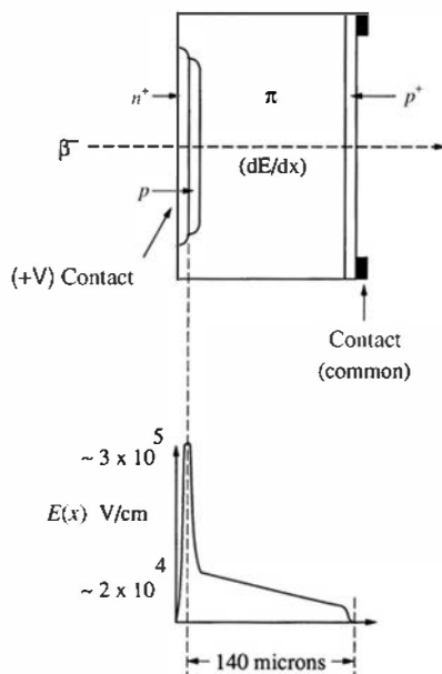
Figure 13.32 The “reach-through” configuration for an avalanche diode. (From Hauger et al. 148 )
