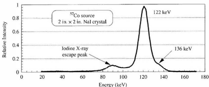
Figure 10.10 Pulse height spectrum from a \text{NaI}(\text{Tl}) scintillator for gamma rays emitted by ^{57}\text{Co} at 122 and 136 keV. The iodine X-ray escape peak lies 28 keV below the corresponding full energy peak and is evident only for the more intense 122 keV gamma ray.
