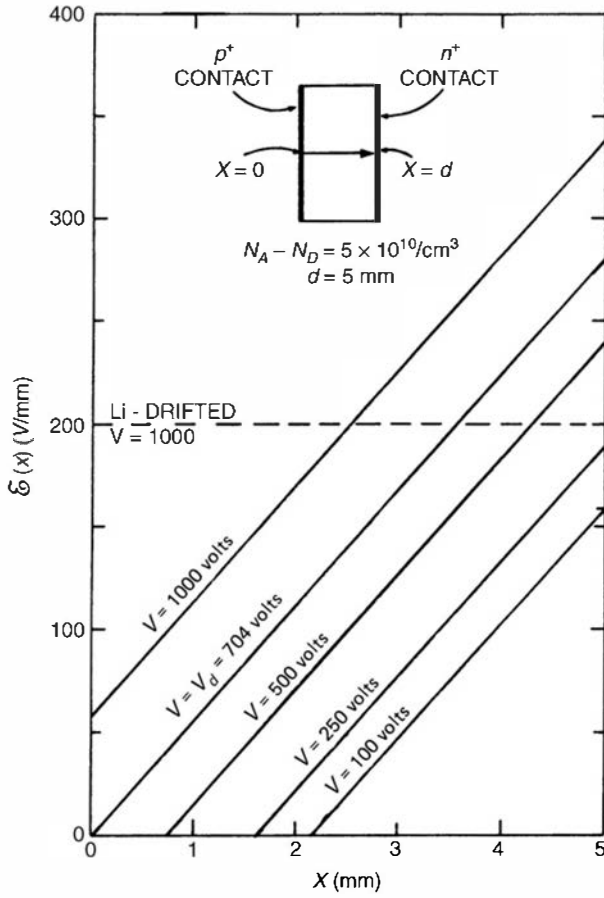
Figure 12.5 The variation of the electric field strength throughout the active volume of a planar HPGe detector for different values of the reverse bias V . The bias value at which full depletion is achieved is labeled V_d . The uniform field present in a Ge(Li) detector of the same dimension is shown for comparison. (From Llacer. 3 )
