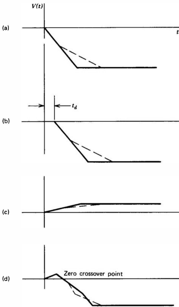
Figure 17.53 Waveforms in the ARC time pick-off method. The original waveform (a) is delayed (b), inverted, and attenuated (c). The sum of (b) and (c) gives waveform (d) with a zero crossover point used to generate the timing signal. The dashed waveform has a slower rise time than the solid, but both give the same timing signal.
