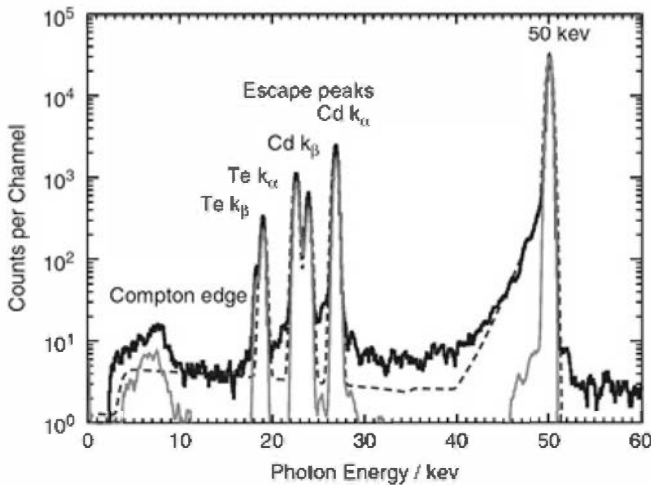
Figure 13.27 Pulse height spectrum recorded from a CdTe detector for incident 50 keV photons (grey curve). Fitted curves (solid and dashed) from several models of detector response are also shown. The four peaks that are located in the 19–27 keV range are due to escape of the K_\beta and K_\alpha X-rays from tellurium, and the K_\beta and K_\alpha X-rays from cadmium. These energies are about 31.0, 27.5, 26.1, and 23.2 keV, respectively, so these values correspond to the spacing of each escape peak below the 50 keV incident energy. (From Krumrey et al. 65 )
