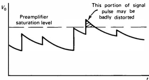
Figure 16.14 The pile-up of pulses within the preamplifier at high rates. If the saturation level of the preamplifier is exceeded, some pulses can be seriously distorted.
