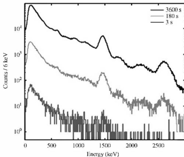
Figure 18.15 Background spectra recorded from a NaI(Tl) scintillator using different measurement times. (From Runkle et al. 52 )
