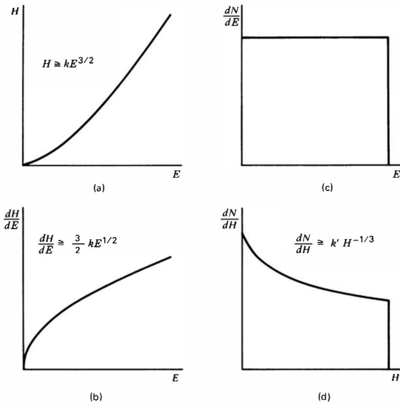
Figure 15.18 Part (a) shows a plot of pulse height versus energy for a typical organic scintillator. This nonlinear response leads to a distortion of the rectangular proton recoil spectrum of part (c) into the spectrum shown in part (d).
