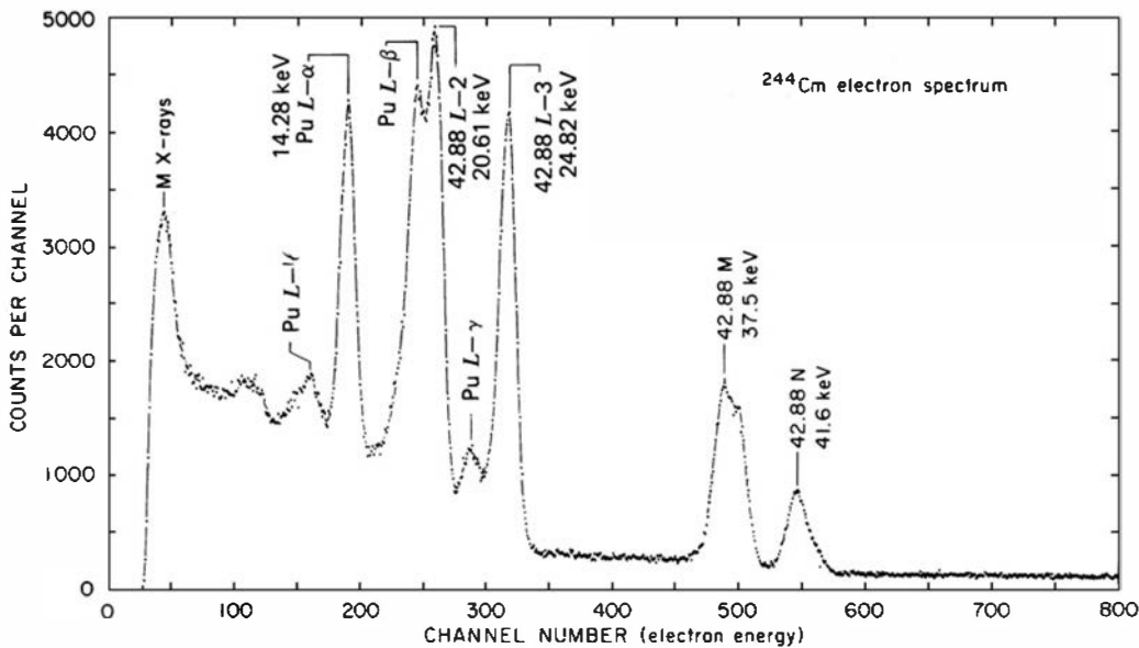
Figure 13.19 Conversion electron spectrum of a ^{244}\text{Cm} sample determined using an 80\text{ mm}^2 \times 3\text{ mm} Si(Li) detector. (From Ahmad and Wagner. 41 )
