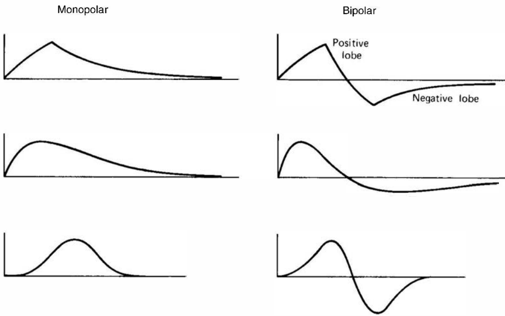
Figure 17.10 Illustration of the distinction between monopolar and bipolar signal pulses of various shapes.
