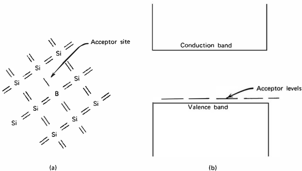
Figure 11.4 (a) Representation of an acceptor impurity (boron) occupying a substitutional site in a silicon crystal. (b) Corresponding acceptor levels created in the silicon bandgap.
