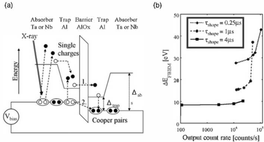
Figure 19.11 (a) Energy band diagram and charge flow in a superconducting tunnel junction detector. Photon or particle absorption produces excess single charges in the absorber, which are trapped by inelastic scattering and produce a current pulse signal as they tunnel across the insulating barrier. (b) Energy resolution versus count rate at a photon energy of 277 eV. STJ detectors can be operated at rates up to 10^4 counts/s at highest energy resolution, and up to 10^5 counts/s with shorter shaping times and thus lower resolution. 86
