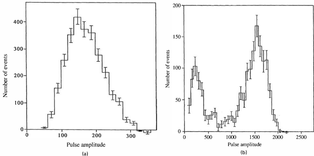
Figure 15.28 Measured spectra from a capture-gated neutron spectrometer for incident neutrons with energies of 1.2 MeV (part a ) and 6.7 MeV (part b ). (From Czirr and Jensen. 181 )
