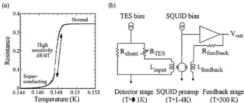
Figure 19.8 (a) Resistive transition of a superconducting molybdenum–copper transition edge sensor. For radiation detection, the TES is operated R(T) at transition. (b) Schematic TES read-out circuit. The TES is biased in the transition in parallel with a shunt resistor R_S \ll R_{\text{TES}} to maintain a constant voltage bias for electrothermal feedback, and read out with a SQUID preamplifier in feedback mode. (Courtesy of S. Friedrich, Lawrence Livermore National Laboratory.)
