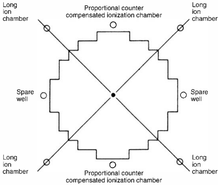
Figure 14.11 Geometric arrangement of out-of-core neutron detectors relative to the core of a PWR. (From Harter and Beckerley. 83 )
