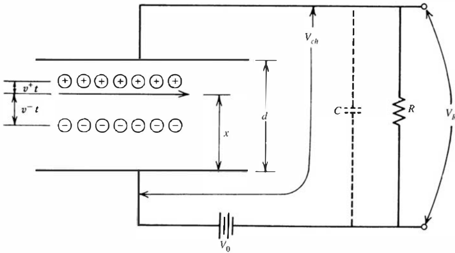
Figure 5.15 Diagram for the derivation of the pulse shape V_R(t) for the signal from an ion chamber. See the text for identification.
