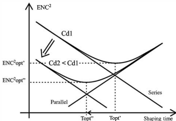
Figure 17.27 Series and parallel noise behavior of two detectors that are identical except for their capacitance values. The higher-capacitance detector (labeled as Cd1) reaches its minimum noise performance at an optimum shaping time labeled T_{\text{opt}'} . The detector with lower capacitance reaches a lower noise level at a shorter optimum shaping time. (From Fiorini. 25 )
