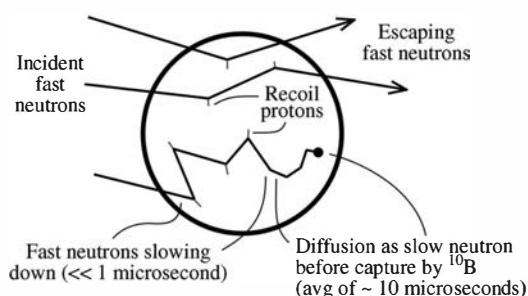
Figure 15.26 Principle of the capture-gated neutron spectrometer using a plastic scintillator loaded with ^{10}\text{B} .
