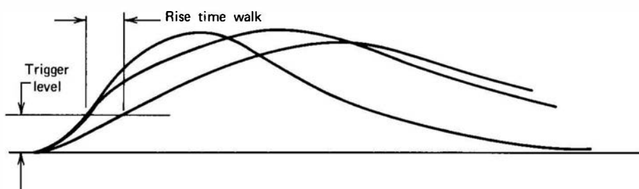
Figure 17.50 Time walk in leading edge triggering due to variations in pulse shape or rise time. Changes in either the overall pulse rise time or the shape of the leading edge for pulses with the same rise time can be responsible for time walk.
