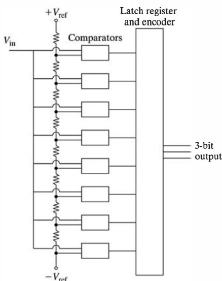
Figure 17.42 Block diagram of a 3-bit flash ADC. Each additional one bit of resolution doubles the required number of comparators.
