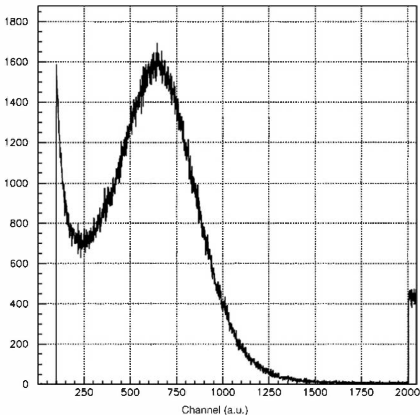
Figure 9.13 Pulse height spectrum measured from a Hamamatsu R5912 PMT due to single electrons emitted spontaneously under dark conditions from the photocathode. (From Bauleo et al. 39 )
