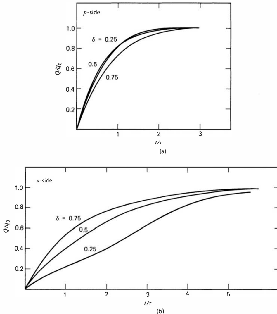
Figure 13.4 Calculated shape of the signal pulse leading edge for electrons incident on a Si(Li) detector. Various assumed electron ranges are shown, defined as \delta \equiv electron range/detector thickness. The time scale is in units of \tau \equiv d/\mu_e \mathcal{E}_0 , where d = detector thickness, \mu_e is the electron mobility, and \mathcal{E}_0 is the maximum electric field whose shape is assumed to be given by Eq. (13.2). (a) Electrons incident on the p side (high-field side) of the detector. (b) Electrons incident on the n side (low-field side) of the detector. (From Moroz and Moszynski. 10 )
