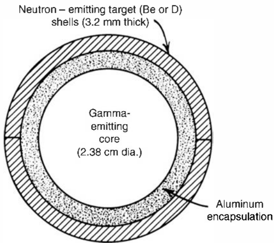
Figure 1.15 Construction of a simple spherical photoneutron source.
