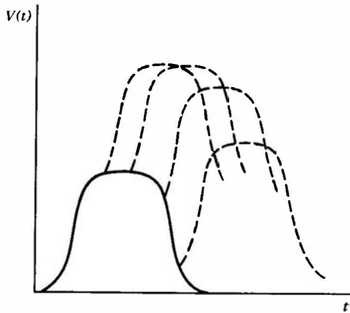
Figure 17.29 Peak pile-up, in which two closely spaced signal pulses combine to form one distorted pulse. Several different cases are sketched with increasing overlap between the first and second pulse.
