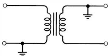
Figure 16.10 The basic configuration of an inverting pulse transformer.
