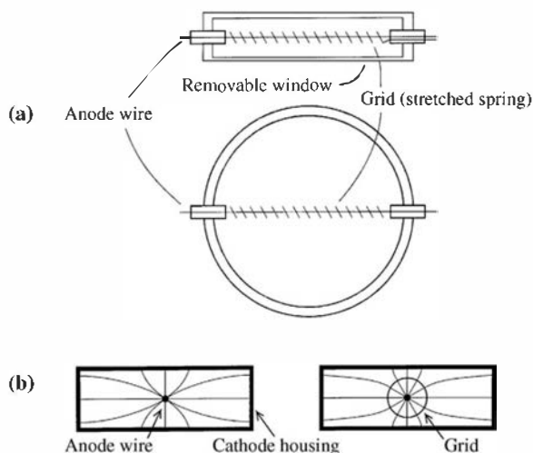
Figure 6.9 In part (a), the shape of the “pancake” proportional tube is shown. The effect of the grid on improving the uniformity of the electric field around the anode wire is illustrated in part (b).
