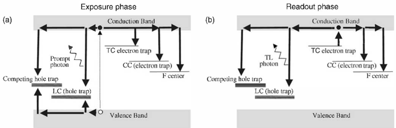
Figure 19.14 (a) Conduction band-valence band model for the exposure phase of the TL mechanism. Electrons and holes formed by the incident radiation can migrate in the conduction and valence bands and be captured at various electron and hole trapping centers. The capture of electrons at appropriate trapping centers (TC) created by dopants in the crystal builds up a population that will serve as the basis for the signal during readout. Other traps can exist (shown here as competing centers (CC) or color centers (F center)) that do not easily depopulate and so will not contribute to the signal. Also shown is capture at a luminescence center (LC) that can yield prompt light during the exposure period, as in the scintillators described in Chapter 8. Holes migrating in the valence band also are subject to capture, either forming luminescence centers or competing hole traps. (b) The heating phase for TLD readout during which electrons are thermally liberated from the TC. The electrons then randomly migrate in the conduction band, and are subject to capture at a number of different types of trapping centers. The readout signal is based on the light that is liberated when that capture occurs at an LC. Several other competing capture processes that do not lead to a useful signal are also shown. Although the F center and the CCs do not directly contribute to light emission, they can strongly influence the emptying and filling rates of the TCs. Analogous mechanisms involving thermal release, migration, and recombination can occur for the holes. (Courtesy of Y. S. Horowitz, Ben Gurion Univ.)
