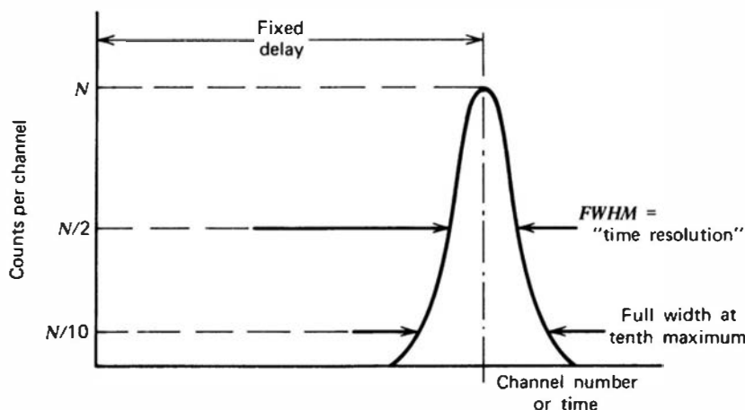
Figure 17.55 The multichannel time spectrum for the system of Fig. 17.54.
