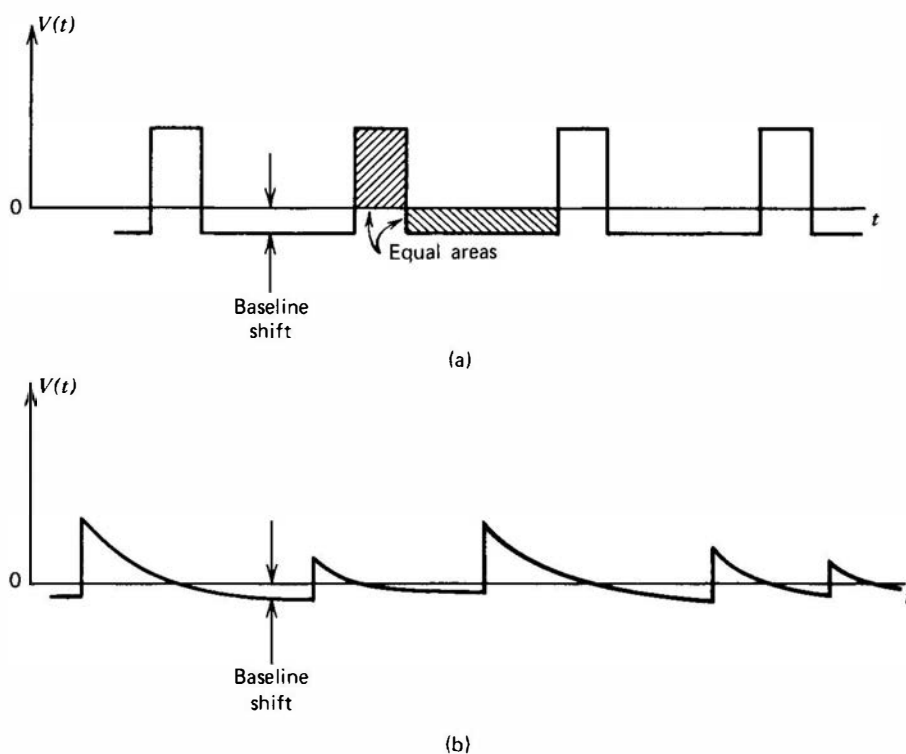
Figure 17.9 Illustrating baseline shift that must take place in ac-coupled circuits. In part (a) uniform and regular pulses lead to fixed baseline shift, but the random pulses of part (b) give rise to variable shift.
