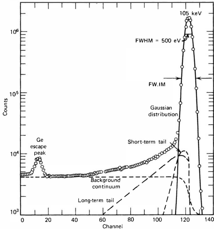
Figure 12.25 Detailed shape of an observed peak from a Ge(Li) detector. (From Meyer et al. 67 )
