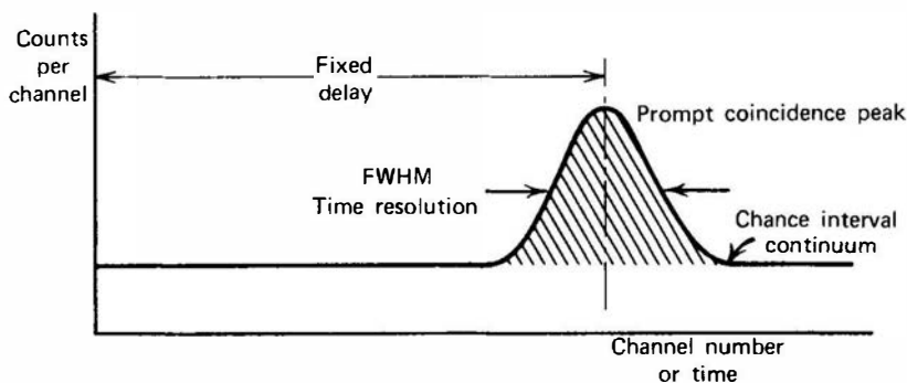
Figure 17.57 The multichannel time spectrum for a radioisotope source emitting some radiation in prompt coincidence. The cross-hatched area gives the total number of recorded coincident events. The time resolution of the system is conventionally defined as the FWHM of the prompt coincidence peak.
