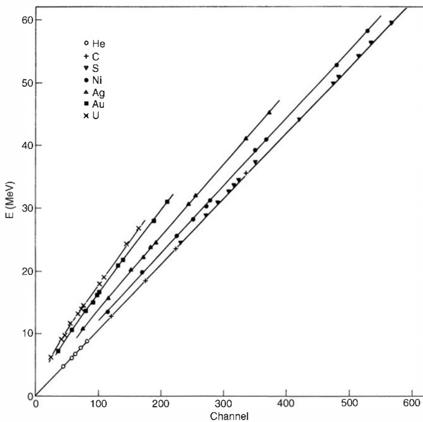
Figure 11.16 The true energy of various ions versus the pulse height channel number from a silicon surface barrier detector. (From Wilkins et al. 81 )
