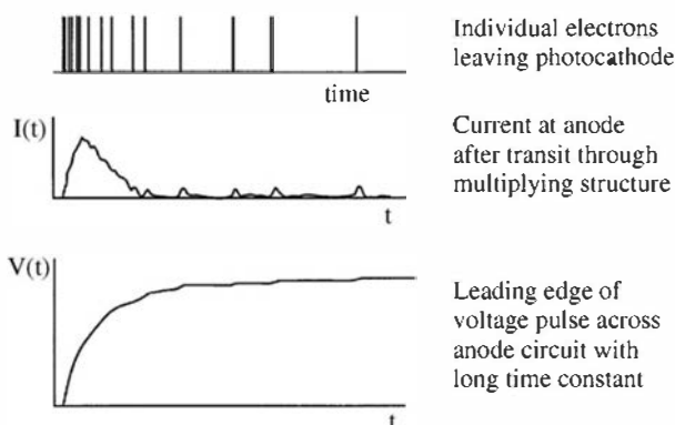
Figure 9.22 The sketch at the top represents the emission of electrons from the photocathode as a function of time following a scintillation event. The resulting current arriving at the anode is shown in the middle plot, and the bottom curve is the leading edge of the voltage pulse produced by integrating this current on an anode circuit with a long time constant.
