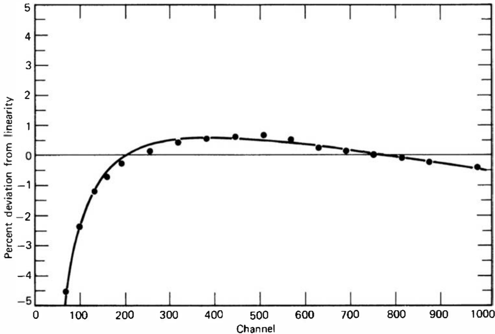
Figure 12.30 A typical differential linearity plot for a germanium detector system. (From Zulliger et al. 91 )
