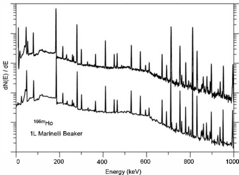
Figure 12.23 Comparison of simulated (upper plot) and measured (lower plot) of the complex gamma-ray spectra produced by a sample of ^{166\text{m}}\text{Ho} by a HPGe detector with 40% relative efficiency (From García-Toraño et al. 63 )
