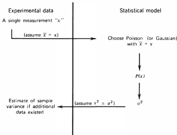
Figure 3.12 An illustration of Application B of counting statistics—prediction of the precision to be associated with a single measurement.
