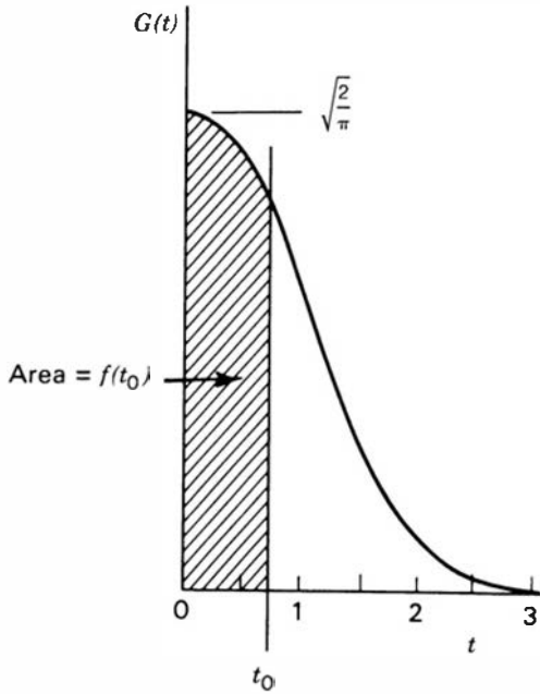
Figure 3.8 A plot of the general Gaussian curve.
