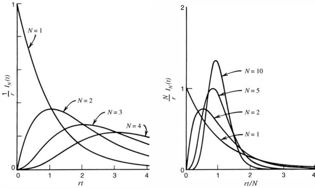
Figure 3.16 Graphical representation of the scaled interval distribution I_N(t) . (a) Four distributions for scaling factors of 1, 2, 3 and 4. (b) Interval distributions for N = 1 through N = 10 normalized to the same average interval N/r .
