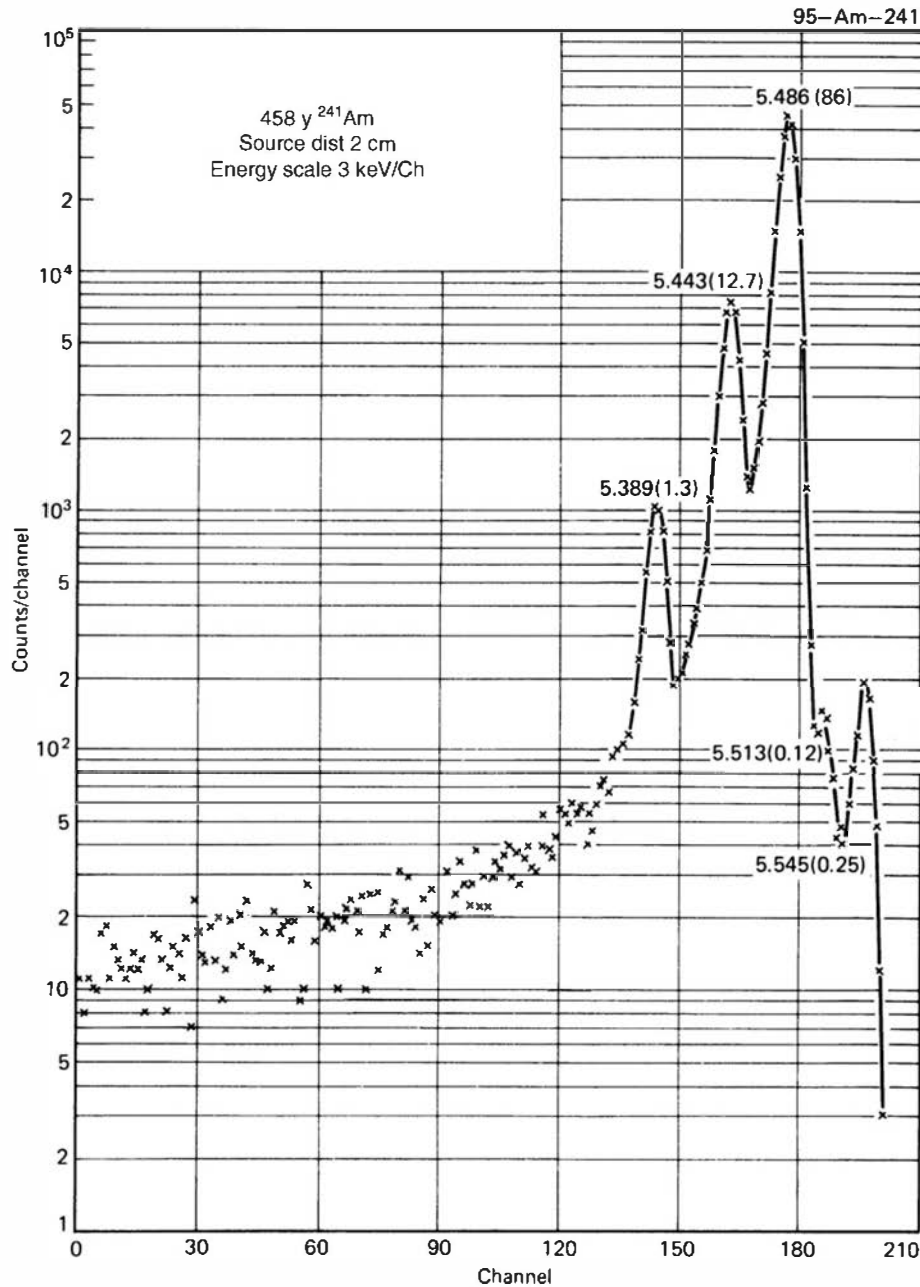
Figure 11.15 Upper portion of the 241 Am alpha spectrum as recorded by a high-resolution surface barrier detector. (From Chanda and Deal. 80 )
