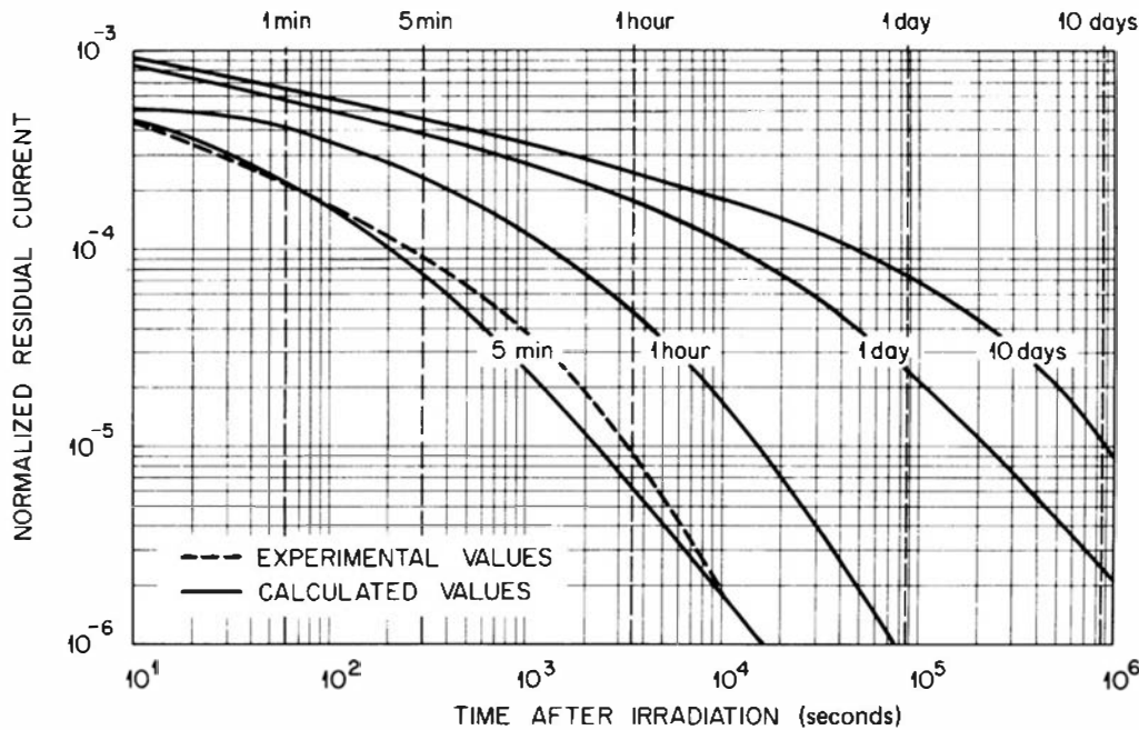
Figure 14.14 Memory effect in fission chambers corresponding to various steady-state irradiation times. (From Roux. 86 )
