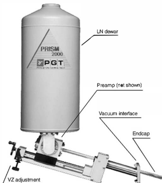
Figure 13.16 An example of a typical low-energy photon spectrometer system consisting of a Si(Li) detector within a cryostat fitted with a thin endcap window. The first stage of preamplification is also located near the detector and cooled through a thermal conductor in contact with the liquid nitrogen in the dewar, while the rest of the preamp is external. The “VZ Adjustment” allows adjustment of the position of the detector, which is normally inside a vacuum chamber needed to eliminate any air between the source and detector to prevent attenuation of soft X-rays. (Courtesy of Princeton Gamma Tech, Princeton, NJ)
