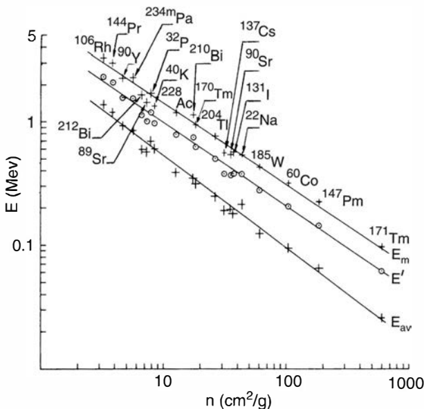
Figure 2.16 Beta particle absorption coefficient n in aluminum as a function of the endpoint energy E_m , average energy E_{av} , and E' \equiv 0.5(E_m + E_{av}) of different beta emitters. (From Baltakmens. 27 )
