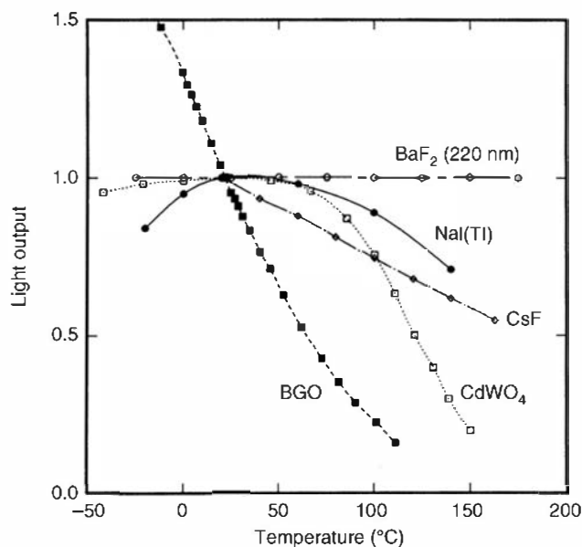
Figure 8.12 The dependence of the light output of some common scintillators as a function of temperature. Only the fast (220 nm) component from \text{BaF}_2 is included. (From Melcher. 118 )
