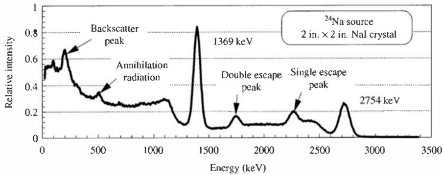
Figure 10.14 Pulse height spectrum from a NaI(Tl) scintillator for gamma rays emitted by ^{24}\text{Na} at 1369 and 2754 keV. The single and double escape peaks corresponding to pair production interactions of the higher energy gamma rays are very apparent, as is the annihilation radiation peak at 511 keV due to pair production interactions in surrounding materials.
