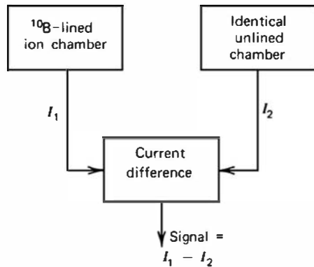
Figure 14.9 Operating principle of a compensated ion chamber (CIC).
