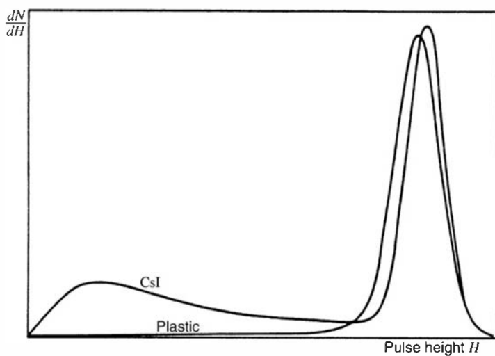
Figure 10.33 Experimental pulse height spectra from CsI(Tl) and plastic scintillators for 1.0 MeV electrons at normal incidence. The spectra are normalized to the same maximum pulse height. (From Titus. 57 )
