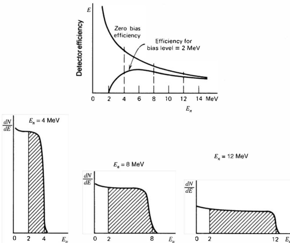
Figure 15.22 The effect of discrimination level on proton recoil detector efficiency. The upper graph gives both the zero bias efficiency and the reduced efficiency when a discrimination level corresponding to a proton energy of 2 MeV is used. See text for further elaboration.
