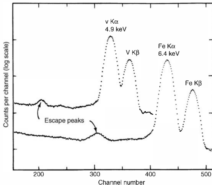
Figure 13.7 Upper portion of pulse height spectra of K X-rays from the decay of 51 Cr and 57 Co. Peaks caused by the escape of the Si X-ray from the detector are evident in both spectra. (From Wood et al. 14 )
