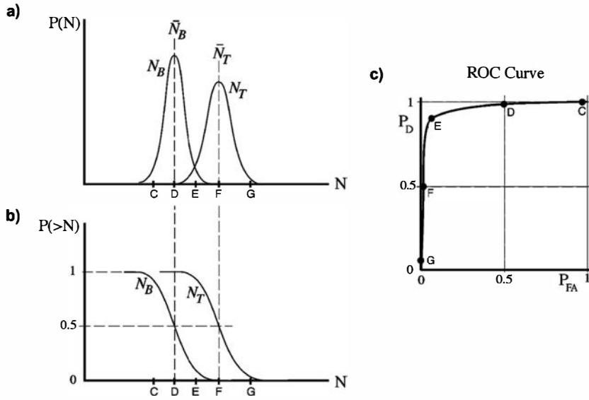
Figure 3.14 (a) Example plots of the probability distributions of observing a specific count N for background ( N_B ) and for the total count ( N_T ) when a true source is present. (b) Plots of the probability of observing a greater number of counts than N for the two example distributions shown in part (a). These plots represent the area under the curves of part (a) that are to the right of any point along the horizontal N scale. (c) The corresponding Receiver Operating Characteristic (ROC) curve for the distributions shown in part (a). The horizontal axis is P_{FA} , the probability of a false positive, and the vertical scale is P_D , the probability of detecting a true source. The five points designate the results when different choices are made for L_C , the minimum number of counts required to declare positive detection of a source. These choices (C through G) are shown along the horizontal axis in parts (a) and (b).
