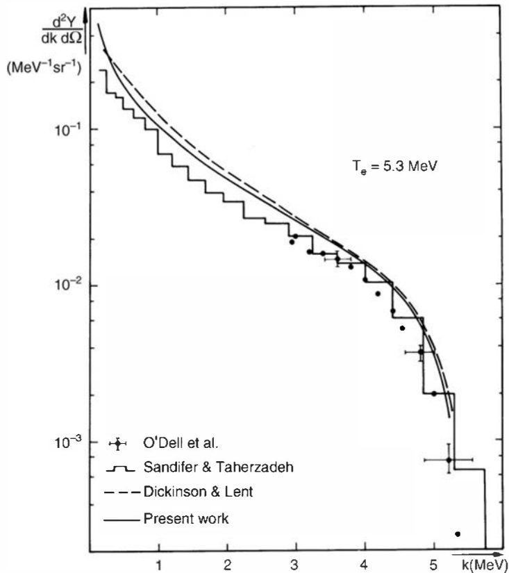
Figure 1.6 The bremsstrahlung energy spectrum emitted in the forward direction by 5.3 MeV electrons incident on a Au-W target. A 7.72 g/cm 2 aluminum filter also was present. (From Ferdinande et al. 14 )
