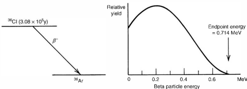
Figure 1.1 The decay scheme of 36 Cl and the resulting beta particle energy distribution.
