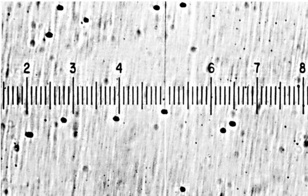
Figure 19.19 Photograph of etched fission fragment tracks in polycarbonate film. The smallest scale division represents 10\ \mu\text{m} . (Photo courtesy of D. M. Gilliam, National Bureau of Standards.)
