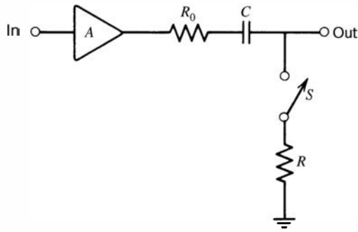
Figure 17.11 Equivalent circuit of a baseline restorer. R_0 is the output impedance of the operational amplifier, normally with gain A = 1 . The time constant is given by the product (R + R_0)C .
