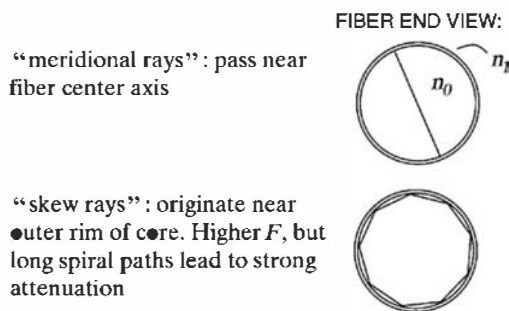
Figure 8.22 Sketch showing the distinction between “meridional rays” that originate near the axis of the fiber, and “skew rays” that represent a much longer transmission path through the fiber.
