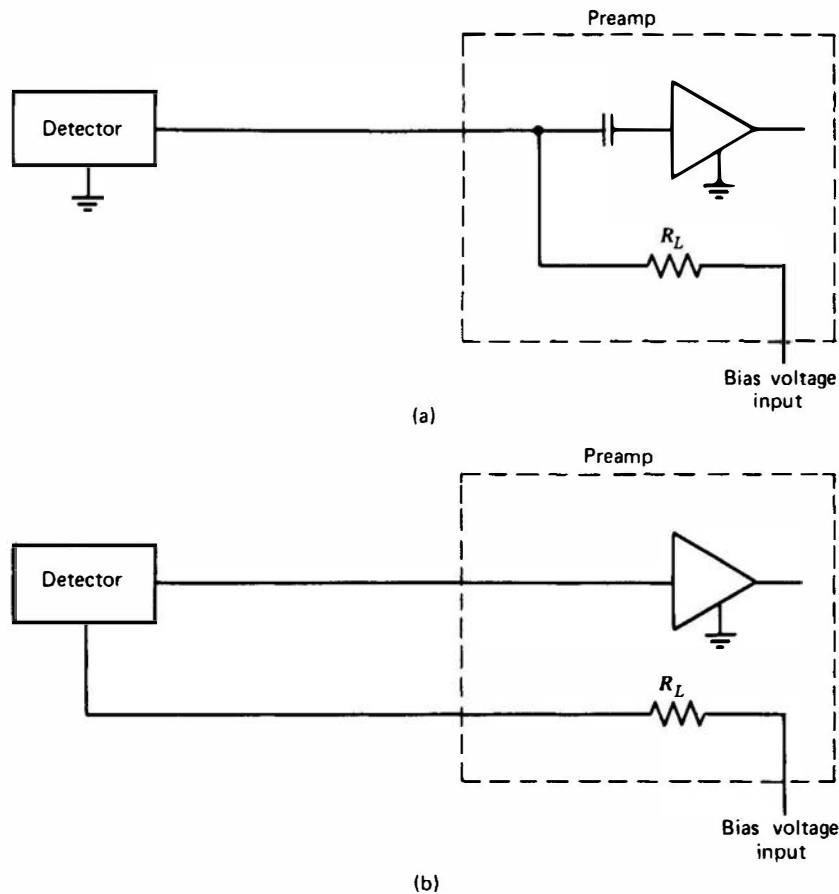
Figure 16.16 Two configurations for supplying detector bias through a preamplifier. (a) An ac-coupled arrangement, in which a coupling capacitor is provided between the detector and preamplifier circuits. This allows interchanging different values of R_L without affecting the preamplifier input. (b) A dc-coupled configuration that eliminates the coupling capacitor and generally leads to better noise performance for critical applications. Now the detector must be isolated from ground, and changing the bias resistor R_L may affect the input stage characteristics.
