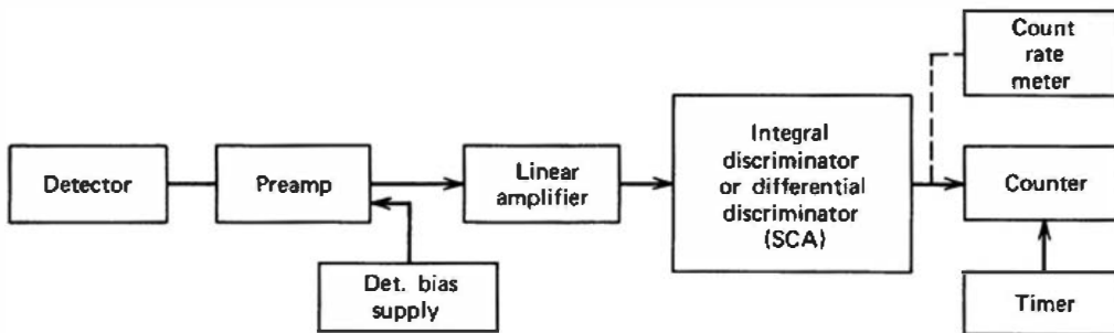
Figure 17.16 Elements of a typical signal chain for pulse counting.
