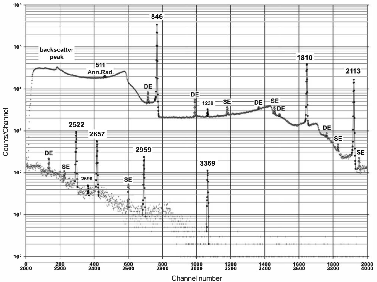
Figure 12.21 Spectrum from a 35 cm 3 Ge(Li) coaxial detector exposed to a source of 56 Mn emitting multiple gamma rays with the energies (in keV) indicated on the plot. Since many of these are relatively high energy, a large number of single escape (SE) and double escape (DE) peaks are evident. (From Helmer et al. 62 )
