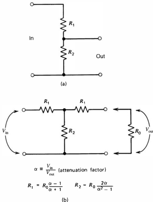
Figure 16.8 (a) A simple voltage-divider attenuation network. (b) A T-attenuator network. The attenuation factor holds provided the network is loaded with the value of R_0 shown. The input and output impedances are then also equal to R_0 .
