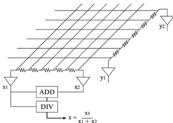
Figure 9.27 Illustration of the crossed-wire scheme for readout of a position-sensing photomultiplier tube. A resistor chain interconnecting all the wires running in one dimension is provided with preamplifiers on each end. Carrying out the operations shown produces a pulse that ideally is proportional only to the event coordinate in that dimension.
