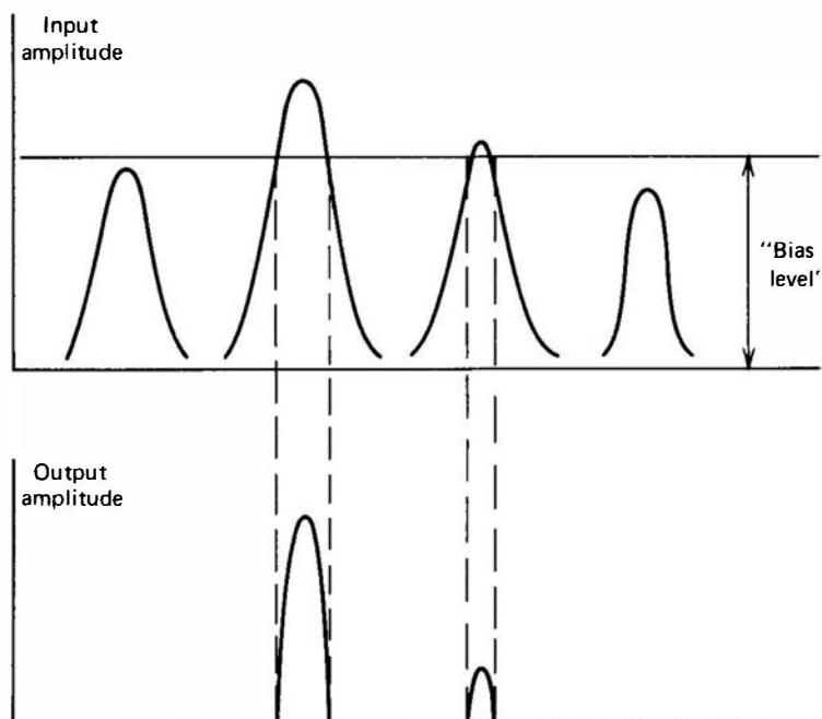
Figure 17.38 The function of a biased amplifier is to provide linear amplification for only that portion of each input pulse that lies above the bias level.
