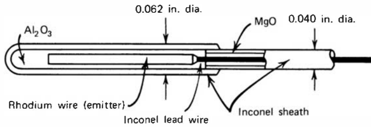
Figure 14.16 Cross-sectional view of a specific self-powered detector design. (From Stevens. 91 )
