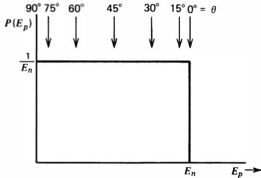
Figure 15.15 Energy distribution of recoil protons E_p produced by monoenergetic neutrons. Recoil energies are indicated for various values of the recoil emission angle \theta as given by Eq. (15.3). For scattering from hydrogen, E_p is equivalent to E_R in Eqs. (15.1) through (15.7).
