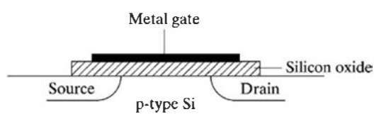
Figure 19.26 Configuration of a metal oxide semiconductor field effect transistor (MOSFET).
