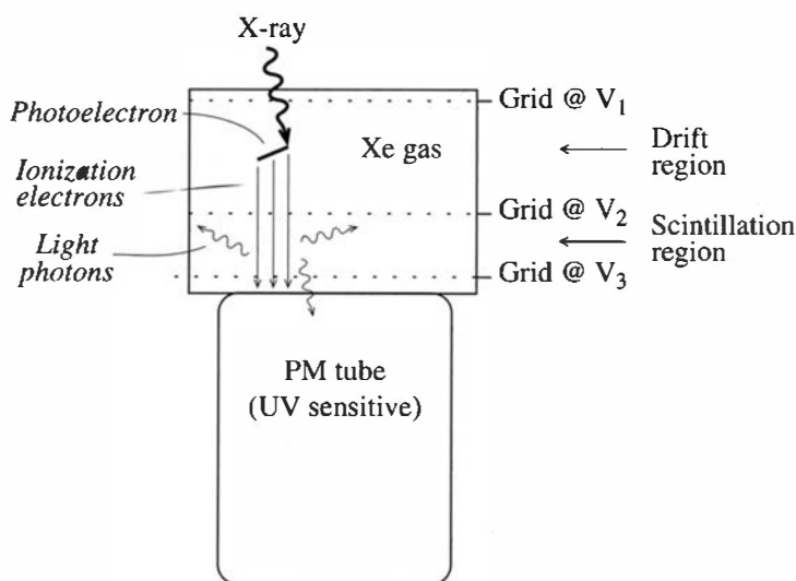
Figure 6.24 Schematic of a gas proportional scintillation counter with a low-field drift region and a higher-field scintillation region. All the light is generated in the scintillation region.
