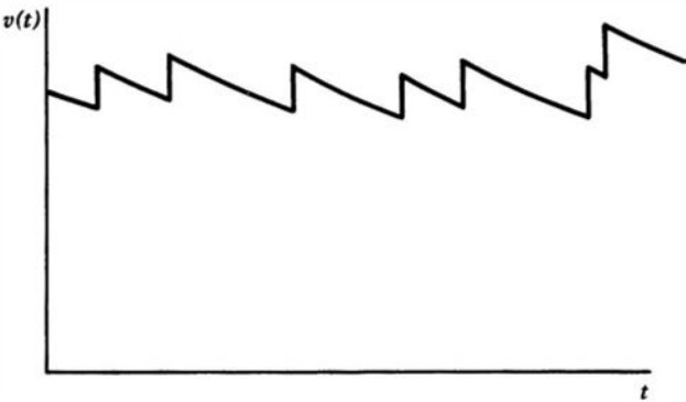
Figure 17.20 Output voltage from the diode-pump rate meter for (a) periodic pulses and (b) random pulses.
