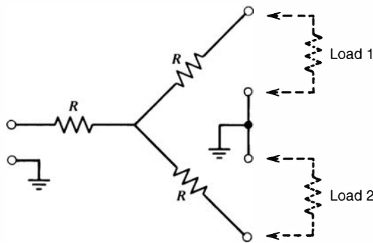
Figure 16.9 A symmetric pulse splitter that can be used to drive two loads while maintaining matched impedance levels.
