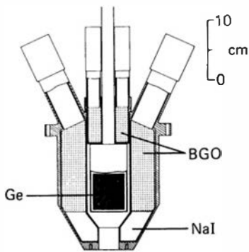
Figure 12.26 An example of a germanium detector surrounded by a Compton suppression system made up of NaI(Tl) and BGO scintillators. (From Nolan et al. 70 )
