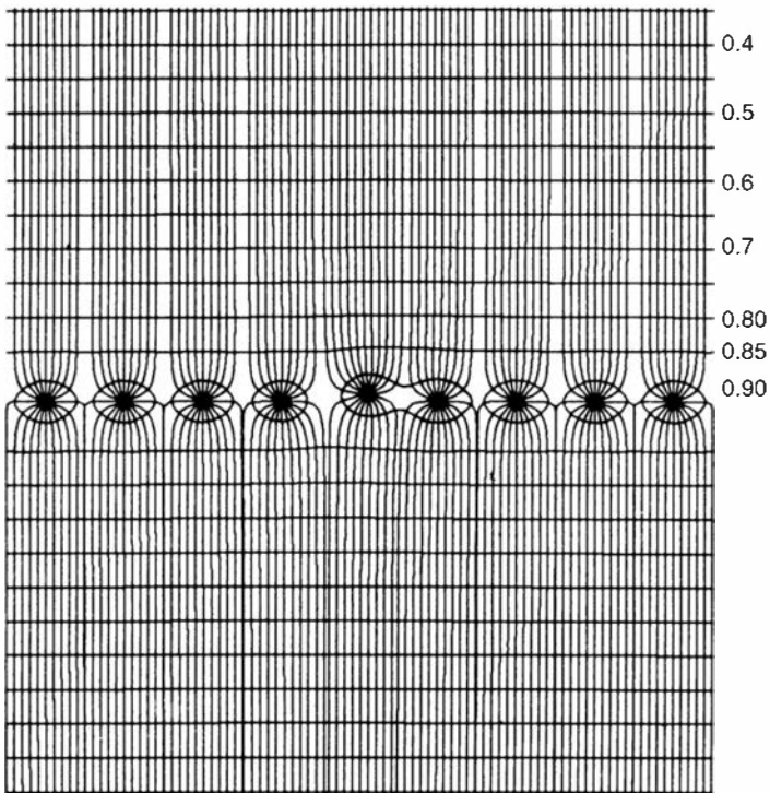
Figure 6.21 A plot of the electric field lines created by a grid of anode wires (running perpendicular to the page) that are placed equidistant between two parallel cathode plates at the top and bottom of the figure. Over much of the volume away from the grid, the field is nearly uniform. A high-field region is created in the immediate vicinity of each grid wire. (From Charpak and Sauli. 107 )
