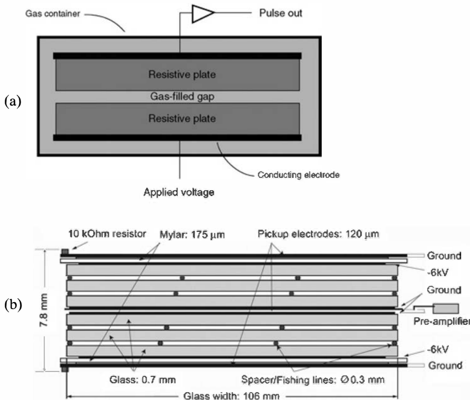
Figure 6.32 (a) Simplified representation of a Resistive Plate Chamber (RPC). A gas-filled gap separates two plates that have an appropriate electrical resistivity. (b) A multigap RPC. The full high voltage is applied to the outer plates, and the inner plates adjust to intermediate voltages. (From G. Belli et al. 164 )
