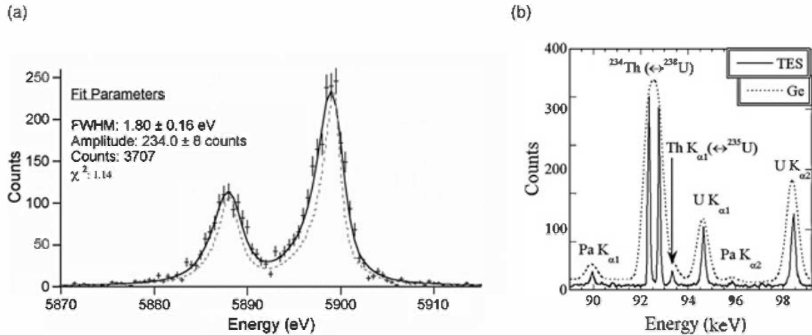
Figure 19.9 (a) ^{55}\text{Fe} X-ray spectrum taken with a Mo/Au TES with a Bi absorber. 72 The dashed line shows the lifetime broadened intrinsic spectral shape of the Mn K_{\alpha_1}/K_{\alpha_2} line complex. (b) 92 keV region of the gamma spectrum from a low-enriched uranium source. 75 The dashed curve shows a spectrum from a typical germanium spectrometer over the same energy range.
