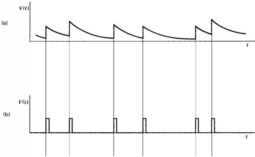
Figure 17.1 The pulses with long tails shown in part (a) illustrate the apparent variation in amplitude due to pulse pile-up. These effects can be greatly reduced by shaping the pulses as in part (b).
