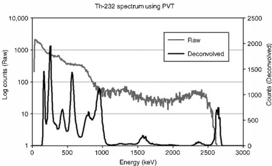
Figure 10.20 Example of the application of deconvolution methods to the direct pulse height spectrum from a plastic scintillator (top curve, log scale) recorded from a source of 232 Th. The deconvolved spectrum at the bottom (linear scale) reveals a number of discrete gamma-ray peaks. (From Burt and Ramsden. 20 )
