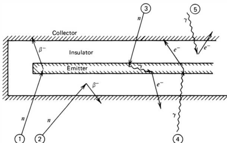
Figure 14.17 Representative events that can take place in an SPN detector. Events ① and ② are neutron capture followed by \beta -decay. Event ③ shows the interaction of a prompt gamma ray emitted upon neutron capture, giving rise to a fast secondary electron. Events ④ and ⑤ show interfering fast electrons arising from interactions of external gamma rays. In standard SPN detectors, event ① is the basis of its neutron response. In those with fast response, event ③ is the preferred mode of interaction.
