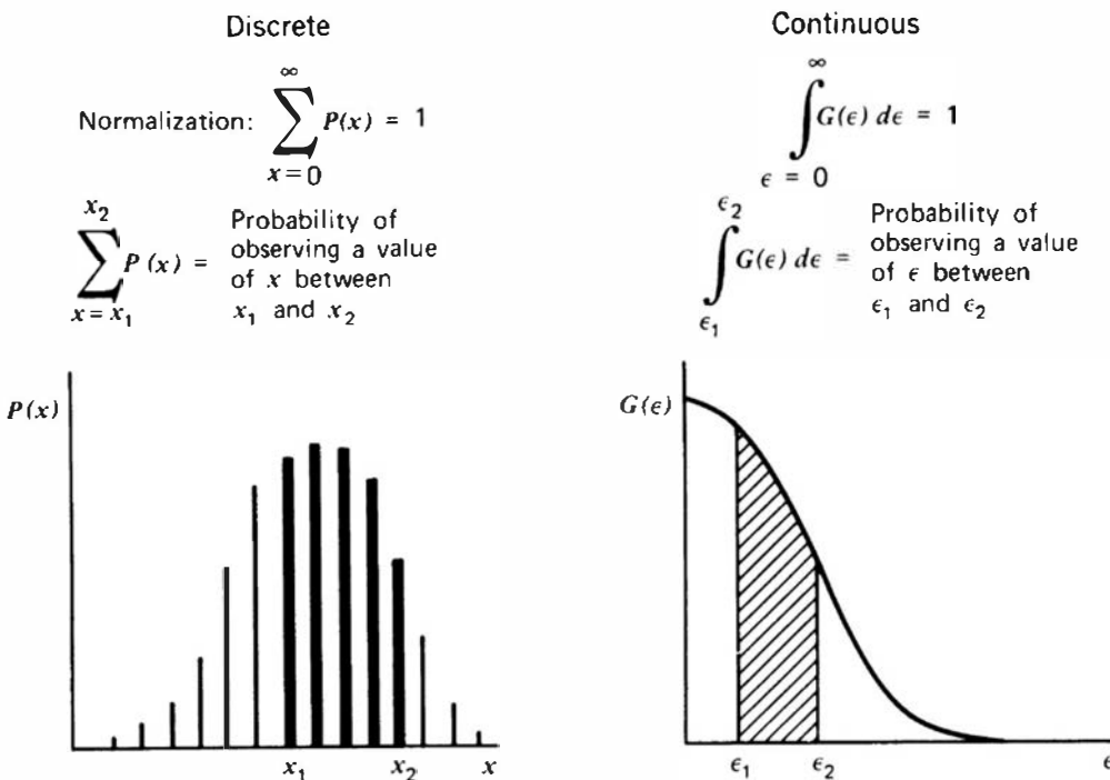
Figure 3.7 Comparison of the discrete and continuous forms of the Gaussian distribution.
