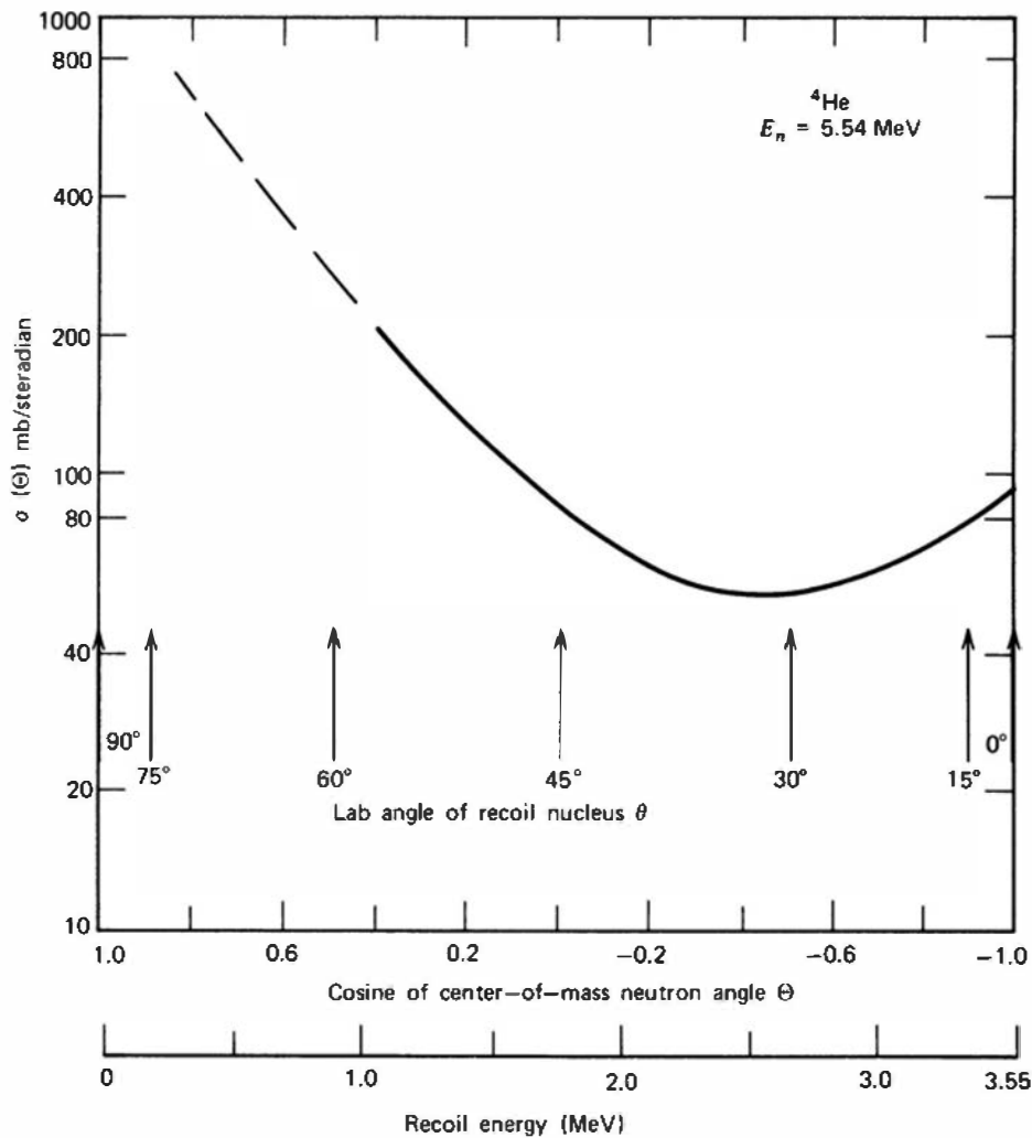
Figure 15.14 The differential scattering cross section of {}^4\text{He} at a neutron energy of 5.54 MeV. Also indicated are the corresponding angle and energy of the helium recoil nucleus in the laboratory system.
