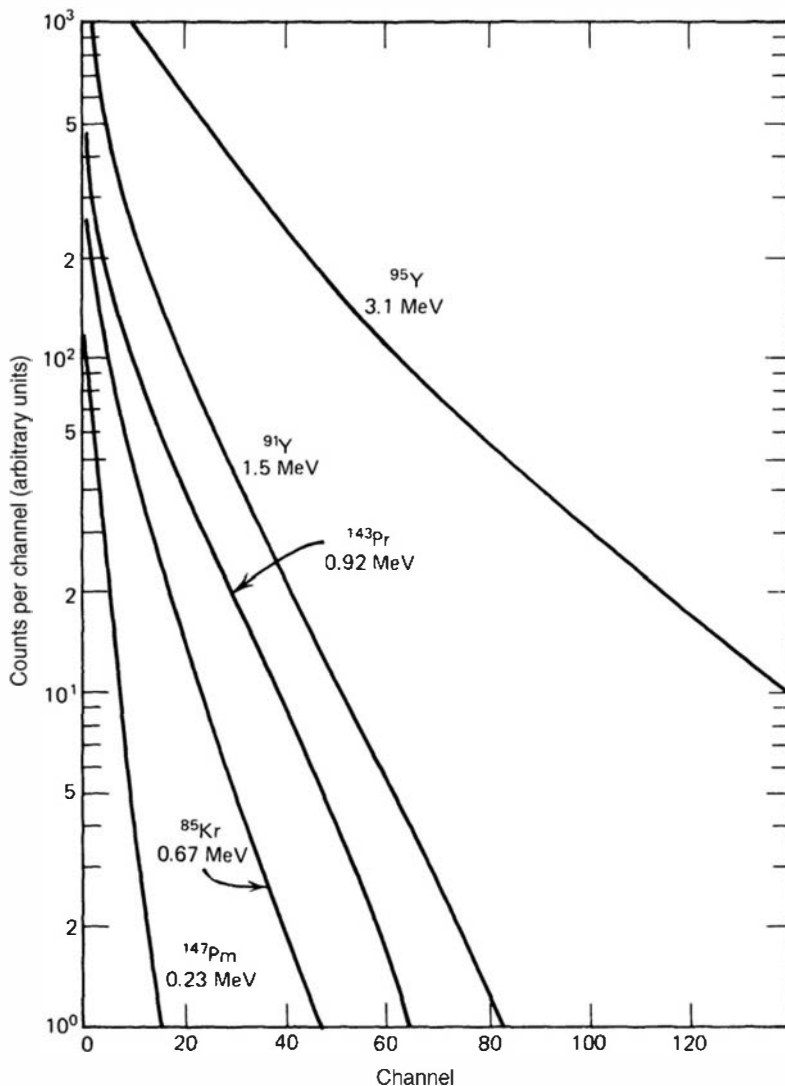
Figure 10.5 Shape of the bremsstrahlung spectra produced by beta particles with the indicated endpoint energies. (From Heath. 5 )
