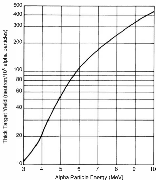
Figure 1.11 Thick target yield of neutrons for alpha particles on beryllium. (From Anderson and Hertz. 23 )
