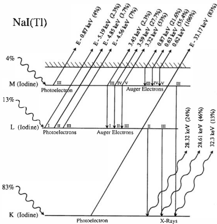
Figure 10.25 Representation of the possible origins of electrons and photons following the photoelectric absorption of an incident X-ray or gamma ray with energy E that is above the K -shell binding energy of 33.17 keV. (From Rooney and Valentine. 35 )
