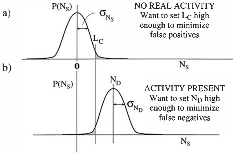
Figure 3.15 The distributions expected for the net counts N_S for the cases of (a) no activity present, and (b) a real activity present. L_C represents the critical level or “trigger point” of the counting system.
