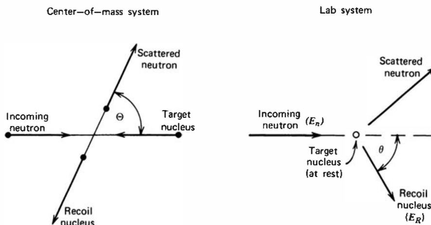
Figure 15.13 Neutron elastic scattering diagrams for the center-of-mass and laboratory coordinate systems.
