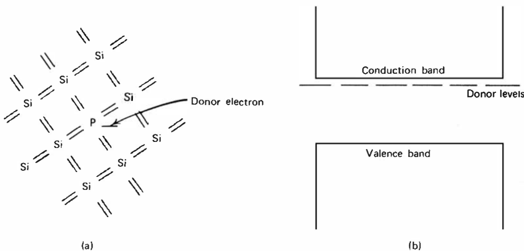
Figure 11.3 (a) Representation of a donor impurity (phosphorus) occupying a substitutional site in a silicon crystal. (b) Corresponding donor levels created in the silicon bandgap.
