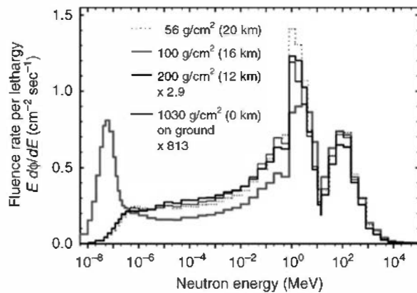
Figure 20.7 Measured energy spectra of background neutrons at ground level and several high altitudes. These spectra typically show peaks at several MeV and around 100 MeV. The ground level spectrum includes a peak at the left from thermalized neutrons. (From Goldhagen et al. 30 )
