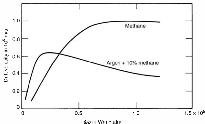
Figure 5.2 Electron drift velocity as a function of electric field \mathcal{E} divided by gas pressure p . (Data from Bortner et al. 8 )
