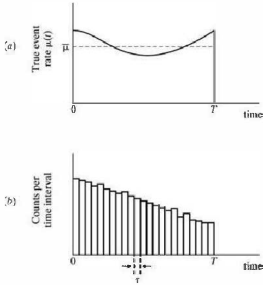
Figure C.1 (a) A measurement in which the true event rate \mu(t) is changing as a function of time. The quantity of interest is the expected distribution of the total number of events (or counts) recorded over the time period from 0 to T . The average true rate over this time period is \bar{\mu} , and the mean number of events is \bar{\mu}T . (b) A series of counts, each taken using a short counting time \tau , extended over a time range from 0 to T when the true rate is changing. The quantity of interest is now the expected distribution in the collection of data consisting of all the recorded counts.
