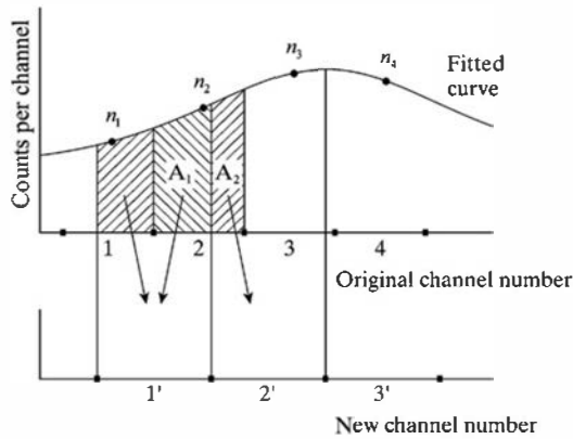
Figure 18.13 Schematic representation of the “rebinning” process to relocate multichannel spectra. The original spectrum is shown at the top as a series of points plotted at the midpoints of the channels 1, 2, 3, . . . A continuous curve has been fit to these points. At the bottom is the new channel scale showing channels 1', 2', 3', . . . In the deterministic process mentioned in the text, the original number of counts n_2 in channel 2 are redistributed to new channels 1' and 2' with fractional assignments of A_1/(A_1 + A_2) and A_2/(A_1 + A_2) , respectively.
