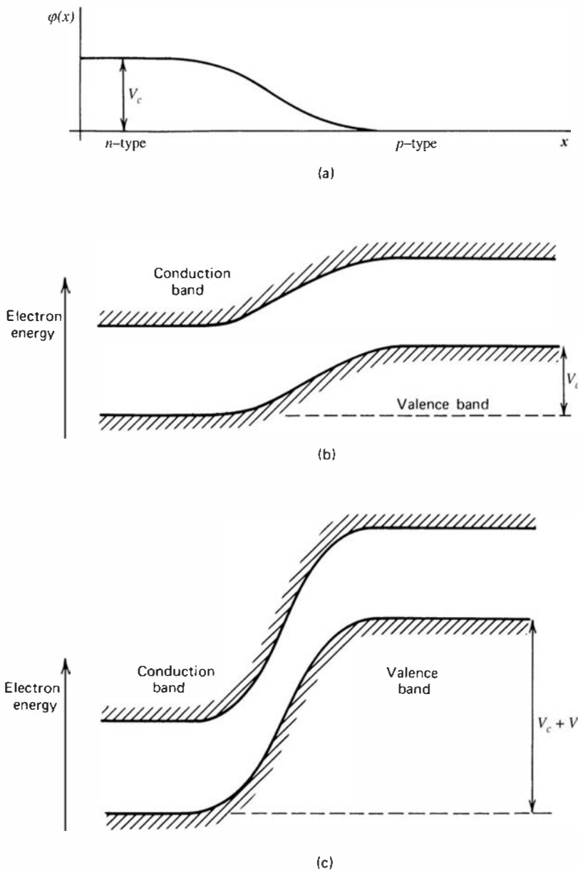
Figure 11.9 (a) The variation of electric potential across an n-p junction from Fig. 11.8. (b) The resulting variation in electron energy bands across the junction. The curvature is reversed because an increase in electron energy corresponds to a decrease in conventional electric potential \phi(x) defined for a positive charge. (c) The added displacement of the bands caused by application of a reverse bias V across the junction.
