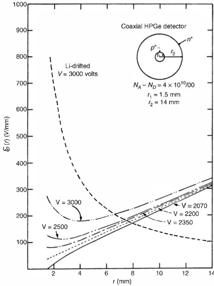
Figure 12.6 The variation of the electric field strength with radius in a HPGe coaxial detector. For the example shown, a minimum value of the reverse bias voltage V of 2070 V is required to fully deplete the detector. The 1/r field variation in a coaxial Ge(Li) detector is shown for comparison. (From Llacer. 3 )
