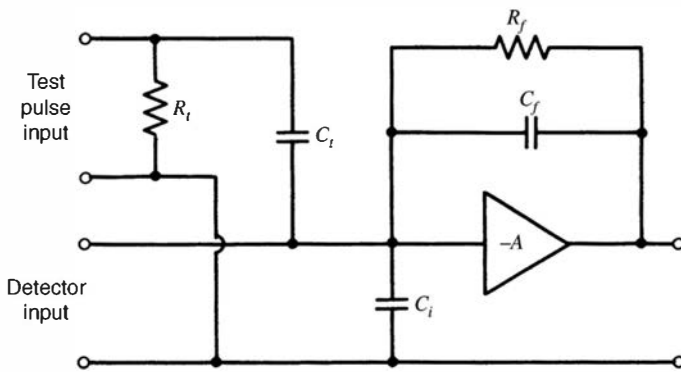
Figure 16.17 A charge-sensitive pre-amplifier that has been provided with a test pulse input. If a step voltage pulse of amplitude V_t is applied to this input, a charge equal to V_t C_t is supplied to the preamplifier input stage. R_t is a small-value termination resistance.
