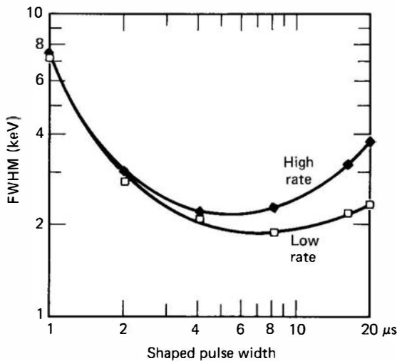
Figure 17.35 Variation of the energy resolution of a typical germanium detector system as the amplifier shaping time is changed. The horizontal axis is the width of the shaped pulse at half maximum. The upper curve is for a relatively high rate (62,000/s) and the lower curve is for a low rate (2000/s). (Data from Fairstein. 48 )
