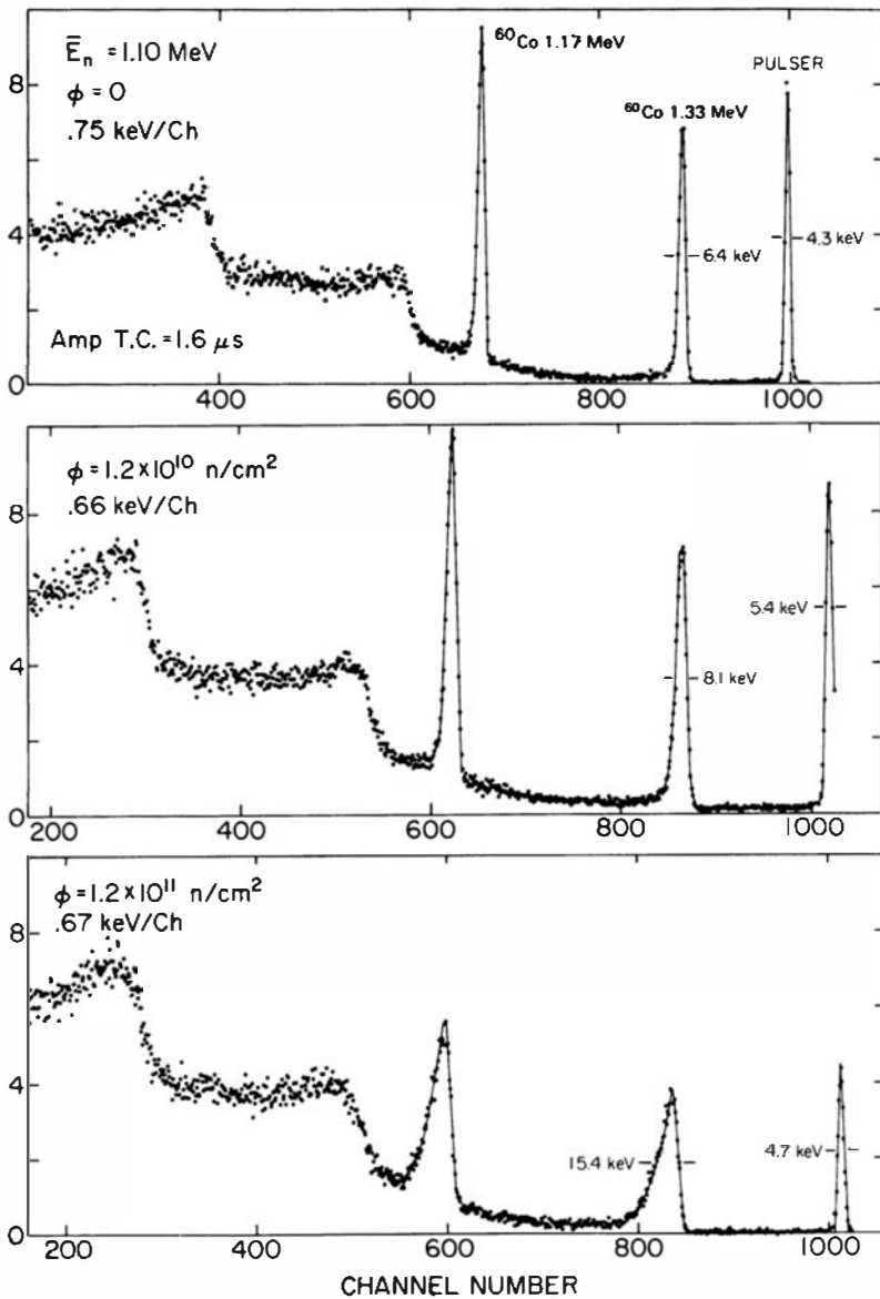
Figure 12.35 The deterioration of a Ge(Li) \gamma -spectrum with increasing neutron fluence. Only the upper part of the spectrum is shown. (From Kraner et al. 118 )
