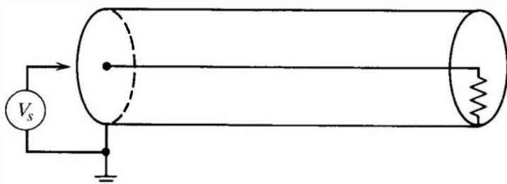
Figure 16.6 Application of a step voltage V_S to a coaxial cable terminated in R_T .
