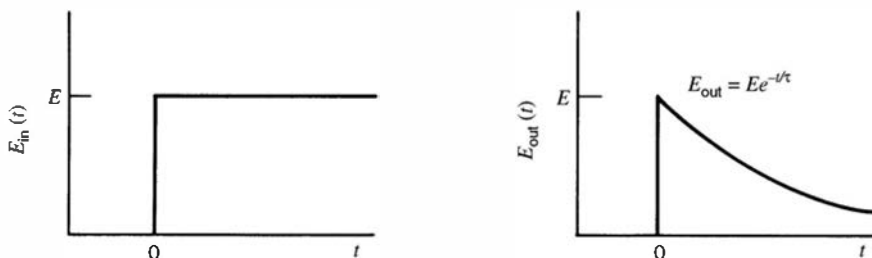
Figure 17.2 A high-pass CR filter or differentiator network. The response to a step function input is illustrated.
