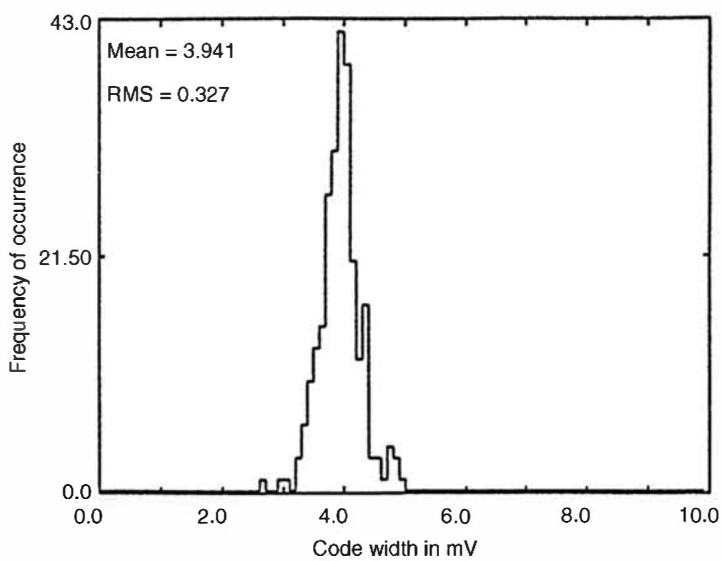
Figure 17.40 Histogram of the frequency of occurrence of measured code widths for a representative flash ADC. (From Crawley et al. 54 )
