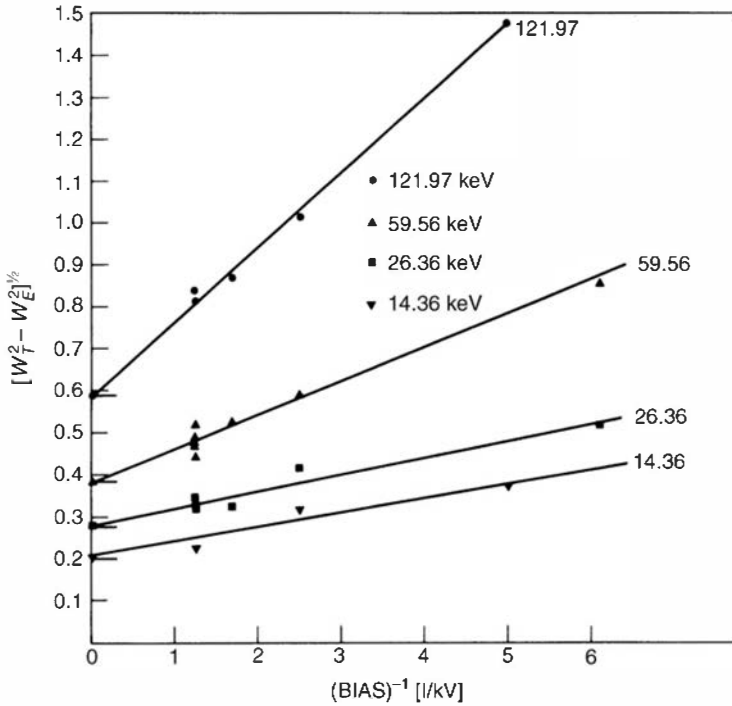
Figure 12.10 Extrapolation of peak width data from an Si(Li) detector to infinite field conditions. The electronic broadening ( W_E ) has already been subtracted quadratically from the measured FWHM, so that the remaining contribution given by the extrapolation should only be due to statistical effects. (From Zulliger et al. 15 )
