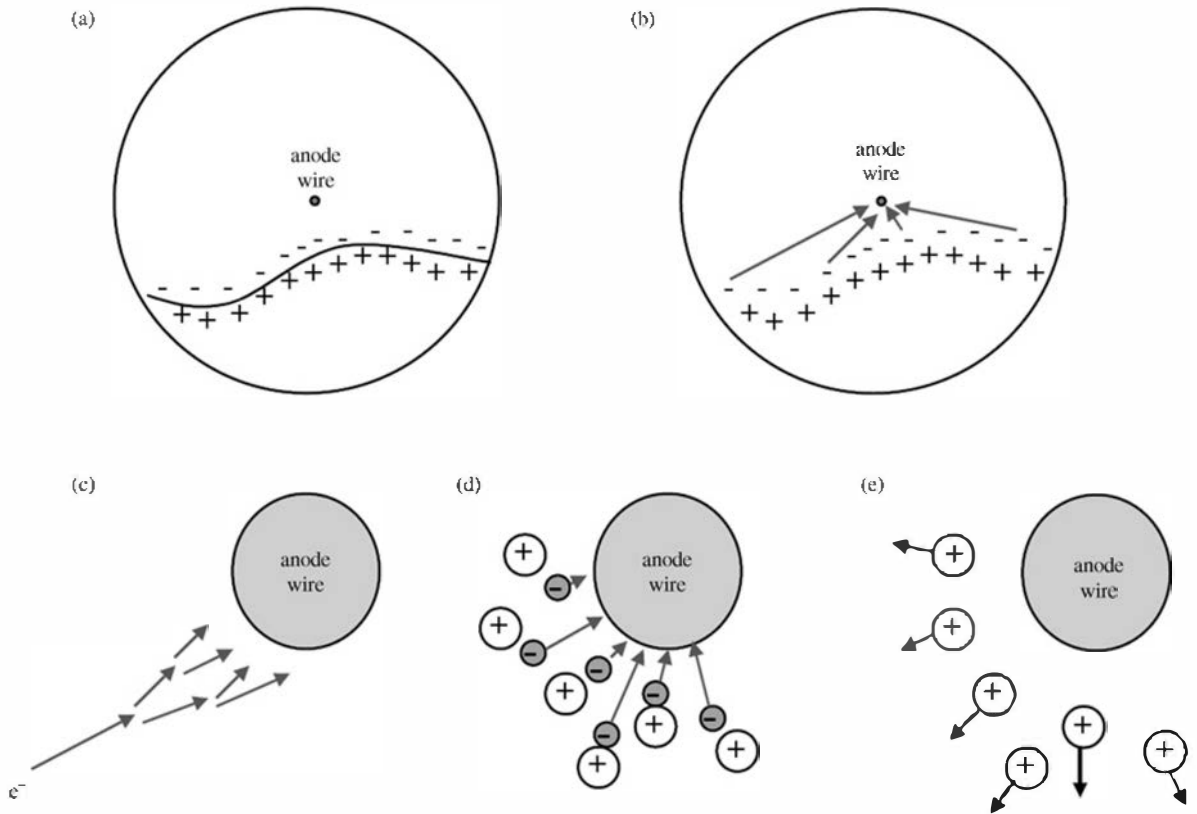
Figure 6.14 The sequence of events in producing a pulse in a proportional counter. (a) An energetic electron or charged particle produces ion pairs in its passage through the counter gas (nanosecond time scale). (b) The ionization electrons drift inward along a radius toward the anode wire (few microsecond time scale). (c) Each electron arriving at the multiplication region triggers its own avalanche (submicrosecond time scale). (d) The hundreds or thousands of electrons formed in each avalanche are quickly drawn to the wire surface (submicrosecond time scale). (e) The much slower positive ions from the avalanche move outward through the high field region near the wire, producing most of the output pulse amplitude (few microsecond time scale).
