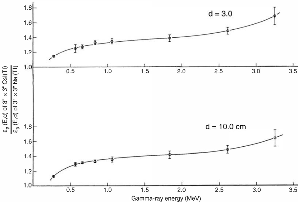
Figure 10.28 Relative intrinsic peak efficiencies of 7.62 cm \times 7.62 cm cylindrical crystals of CsI(Tl) and NaI(Tl); d is the crystal-source distance. (From Irfan and Prasad. 49 )
