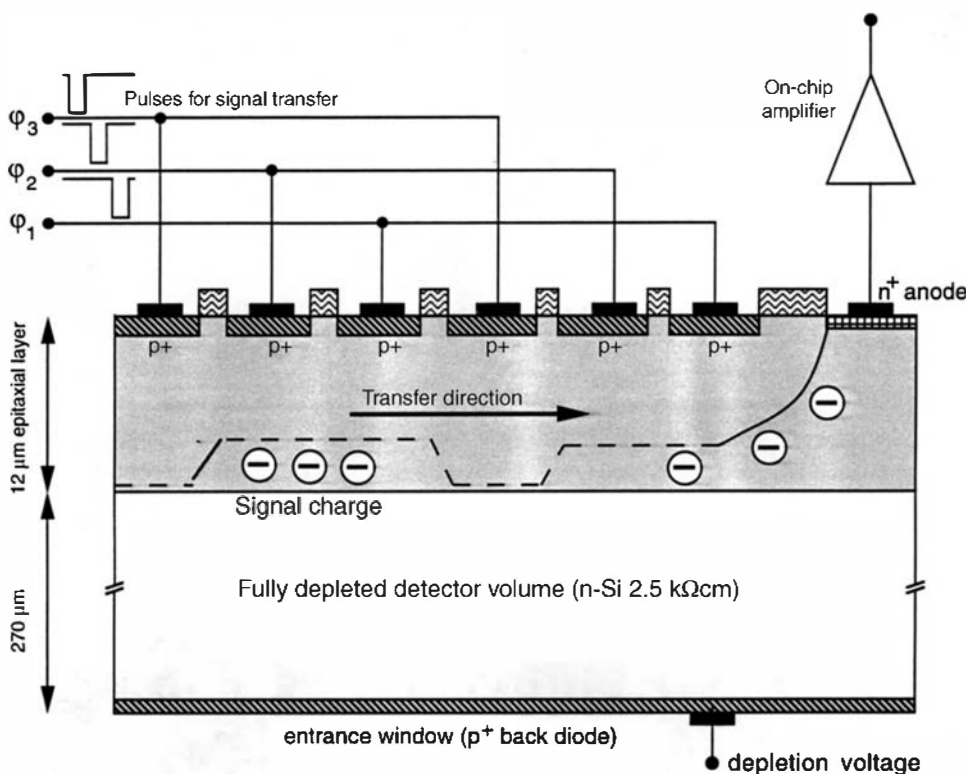
Figure 13.40 Cross section through a transfer channel of pn -CCD. (From Soltau et al. 198 )
