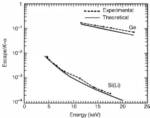
Figure 13.8 Ratio of the X-ray escape peak intensity to the full energy peak intensity for Si(Li) and germanium planar detectors. (From Rossington et al. 15 ).
