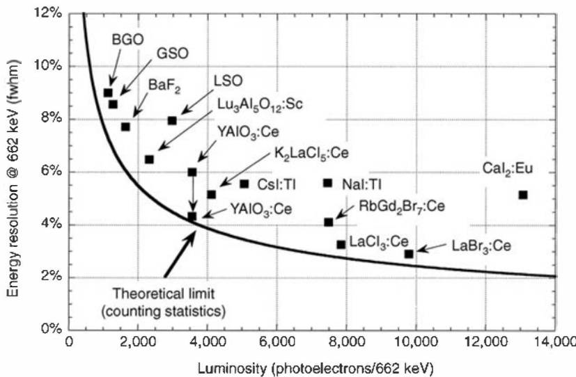
Figure 10.22 The energy resolution (at 662 keV) observed for a variety of scintillators plotted against their luminosity. (Original plot from Ref. 22, with revisions courtesy of William Moses, Lawrence Berkeley National Laboratory.)
