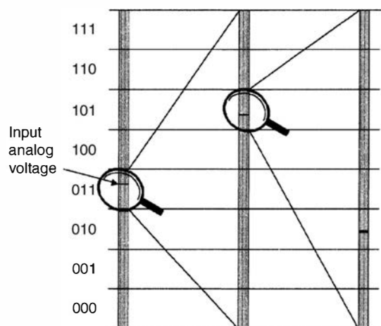
Figure 17.43 Analogy to the operation of a subranging ADC in which magnifiers are used in sequence to expand the analog voltage scale. For the example shown, a sequence of three 3-bit analog-to-digital conversions produces the 9-bit binary code of 011101010, or 234 on a decimal scale of 0–511. (Courtesy of V. Jordanov, Yantel LLC.)
