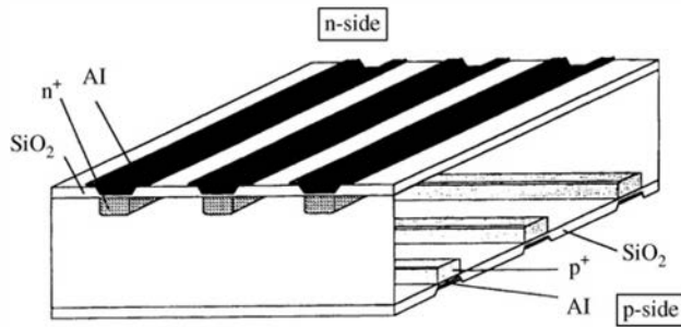
Figure 13.35 Double-sided silicon strip detector. (From Hubbeling et al. 171 )
