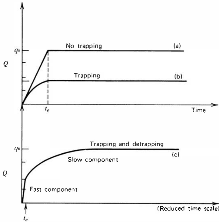
Figure 12.14 Sketches illustrating the pulse leading edge for interactions in a planar detector at one extreme of the active volume: (a) no trapping, (b) permanent trapping, and (c) trapping with slow detrapping. (From Martini and McMath. 46 )
