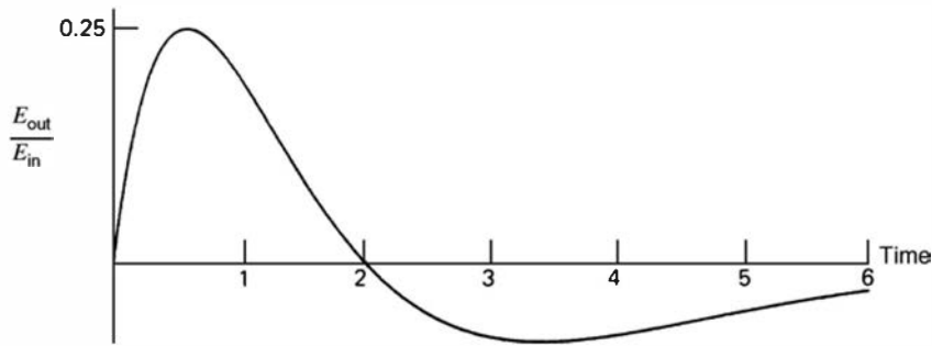
Figure 17.12 The CR-RC-CR network and its output waveform for a step input when all three time constants are equal. Units of the time scale are in values of this time constant.
