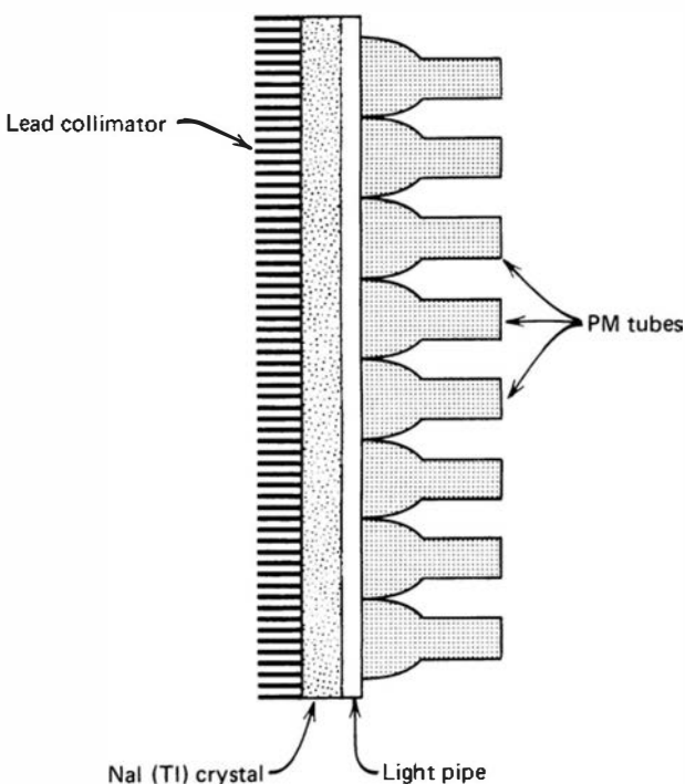
Figure 10.34 Elements of a two-dimensional position-sensitive scintillation detector, commonly called a gamma camera .
