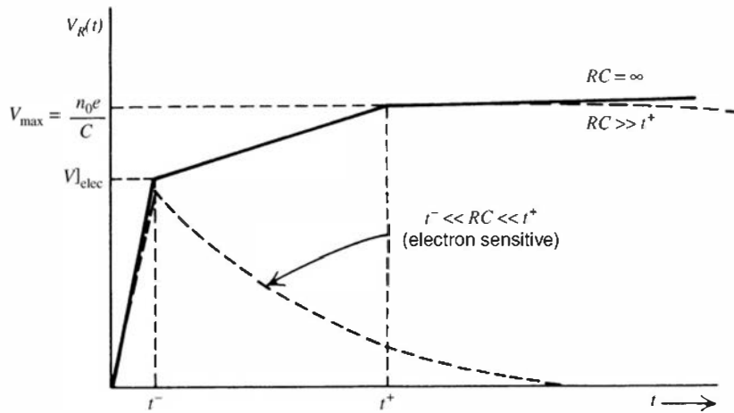
Figure 5.16 Output pulse shape V_R(t) for various time constants RC in the schematic diagram of Fig. 5.15.
