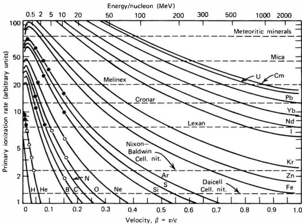
Figure 19.18 The relative ionization rate as a function of energy per nucleon or velocity is shown for various heavy ions. Horizontal dashed lines indicate the minimum damage rate required for 100% registration of tracks on some popular track-recording materials. The solid dots are experiments using accelerated ions on Lexan, which gave 100% registration, and the open circles gave zero registration. (From R. L. Fleischer, P. B. Price, and R. M. Walker, Nuclear Tracks in Solids . Copyright 1975 by The Regents of the University of California; reprinted by permission of the University of California Press.)
