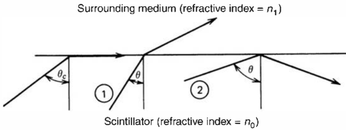
Figure 8.16 Conditions at the interface of dissimilar optical media ( n_0 > n_1 ). Ray ① may escape, but ray ② will be internally reflected at the surface.
