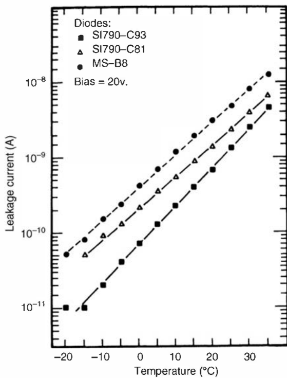
Figure 9.17 The temperature dependence of the leakage current for some typical silicon photodiodes. (From Bian et al. 75 )
