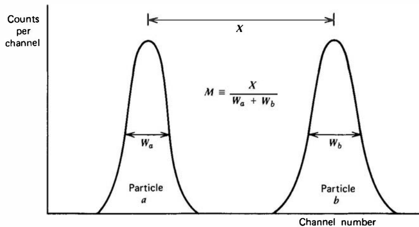
Figure 17.64 Definition of the figure of merit M for pulse shape discrimination applications. In the most common analog PSD method, the abscissa corresponds to the crossover time of a doubly differentiated input pulse.
