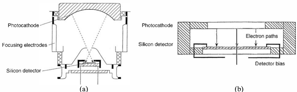
Figure 9.23 Elements of hybrid photomultiplier tubes. Part (a) shows the electrostatic focusing arrangement, while part (b) shows a proximity-focused configuration. (From Basa et al. 103 )
