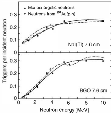
Figure 10.32 The prompt pulse response to fast neutrons in 7.6 cm \times 7.6 cm scintillation detectors of NaI(Tl) and BGO. (From Hausser et al. 56 )
