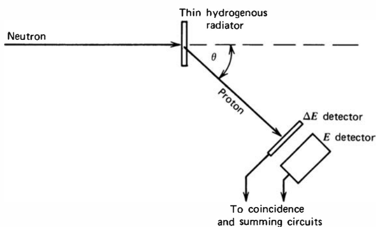
Figure 15.25 A proton recoil telescope.
