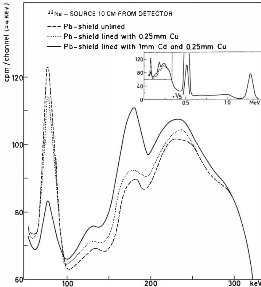
Figure 20.6 A plot of the low-energy portion of the ^{22}\text{Na} gamma-ray spectrum (indicated on the insert) as recorded by a 7.62\text{ cm} \times 7.62\text{ cm} NaI(Tl) scintillator. The effects of different shield liners on the fluorescent X-ray and backscatter peaks are illustrated. (From Stenberg and Olsson. 15 )
