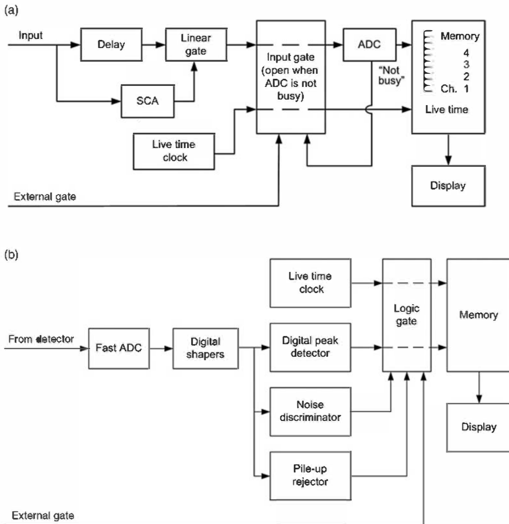
Figure 18.7 Functional block diagram of a typical MCA: (a) based on analog pulse processing, and (b) based on digital pulse processing. (Courtesy of V. Jordanov, Yantel LLC.)
