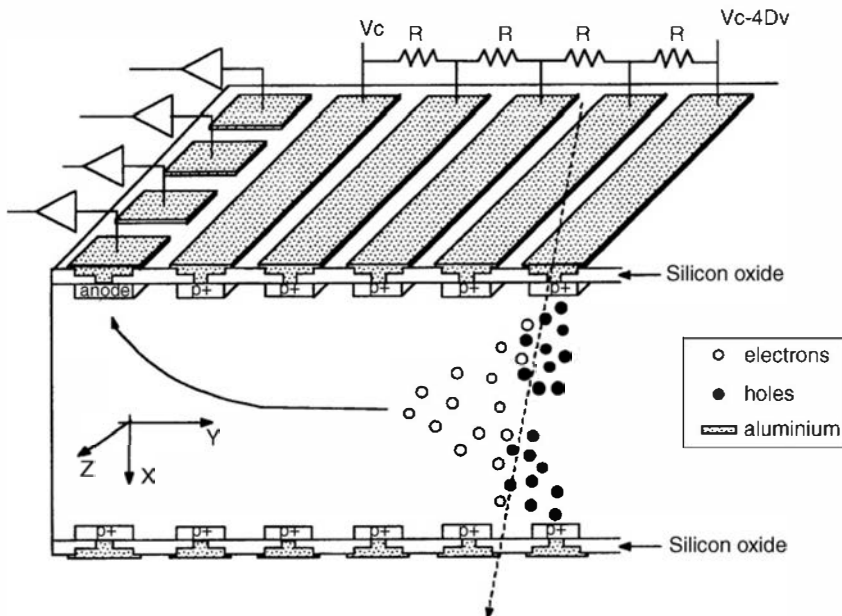
Figure 13.37 Structure of a linear silicon drift detector. Electrons formed by the ionizing radiation are initially drawn to a potential minimum near the center of the wafer. They are then transported parallel to the surfaces by a potential gradient between the surface strips and collected at an anode near the edge of the wafer. (From Gramegna et al. 189 )
