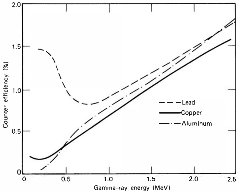
Figure 7.9 The efficiency of G-M tubes for gamma rays normally incident on the cathode. [From W. K. Sinclair, Chap. 5 in Radiation Dosimetry , G. J. Hine and G. L. Brownell, (eds.). Copyright 1956 by Academic Press. Used with permission.]
