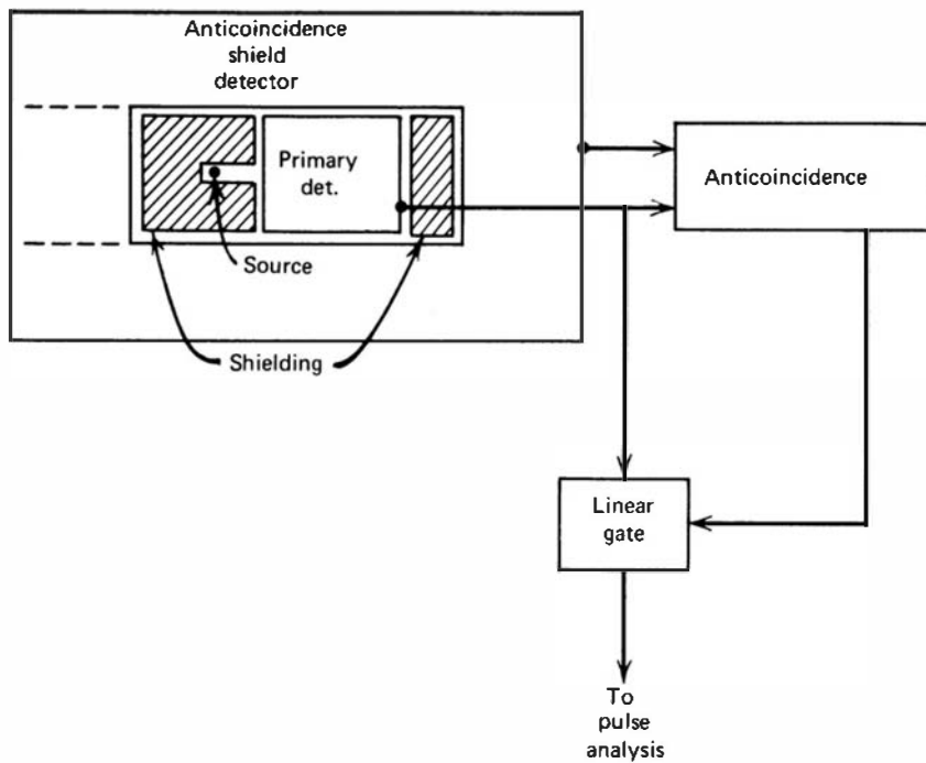
Figure 20.10 The general arrangement of an anticoincidence shield for cosmic background reduction.
