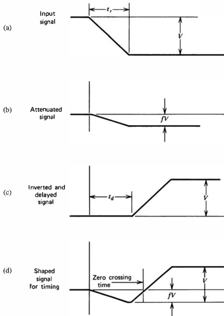
Figure 17.52 Waveforms in the constant fraction time pick-off method. For clarity, only the leading edge of the pulse is shown.
