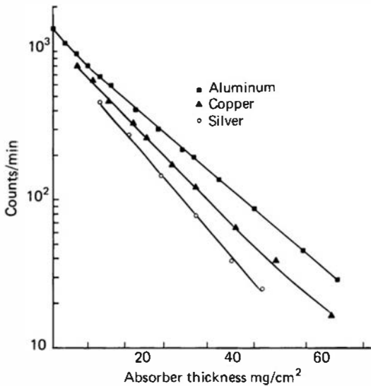
Figure 2.15 Transmission curves for beta particles from 185 W (endpoint energy of 0.43 MeV). (From Baltakmens. 26 )
