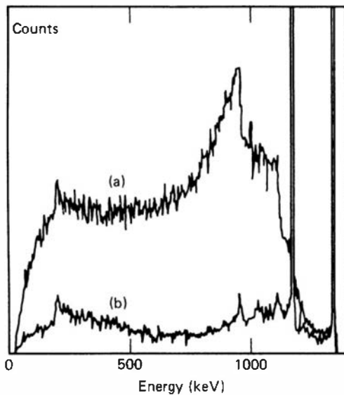
Figure 12.27 Pulse height spectra from a ^{60}\text{Co} gamma-ray source using the system shown in Fig. 12.26. A collimator shielded the scintillators from direct irradiation. (a) Normal spectrum recorded from the central germanium detector. (b) Spectrum recorded in anticoincidence with the scintillation detectors, showing the suppression of the Compton continuum. The full-energy peak areas were unaffected to within 1%. (From Nolan et al. 70 )
