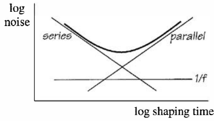
Figure 17.26 Variation of the contributions of series and parallel noise sources as a function of the shaping time in the pulse processing electronics. The minimum in the total occurs at the shaping time that results in equal contributions from series and parallel noise. The 1/f noise contribution is unaffected by the shaping time.
