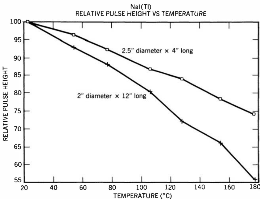
Figure 8.9 The temperature dependence of the light yield measured from two NaI(Tl) crystals. The measurements were made using an oven equipped with a light pipe, and the temperature of the photomultiplier tube was held constant. The difference in behavior between the two crystals is probably due to changes in surface reflectivity. (Data courtesy R. Dayton, Bicon Corporation, Newbury, Ohio.)
