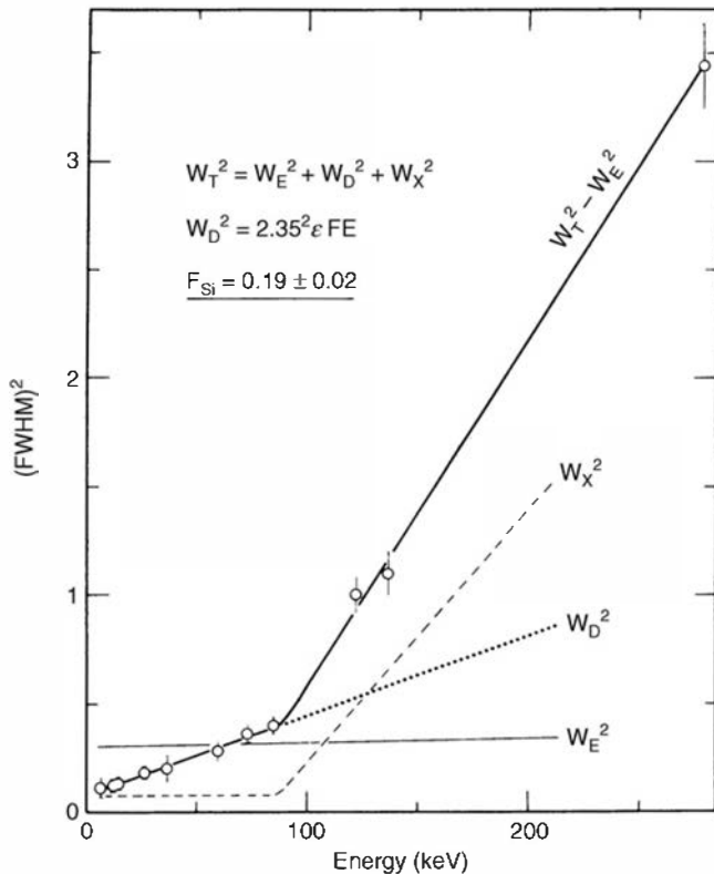
Figure 13.11 Contribution of various noise sources to the total width of the full energy peak from a Si(Li) photon spectrometer. For definitions of the various terms, see the text. (From Hollstein. 26 )
