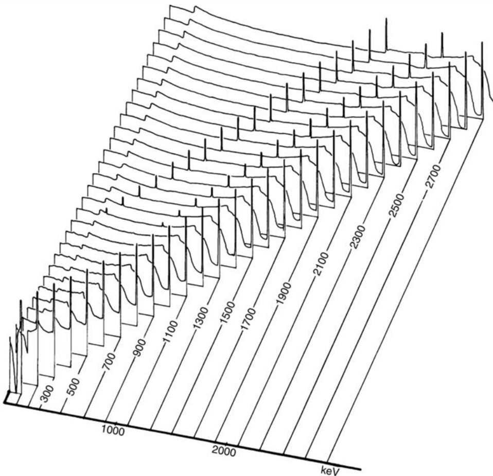
Figure 12.24 Perspective diagram of calculated Ge(Li) spectra for energies up to 3 MeV. (From Meixner. 66 )
