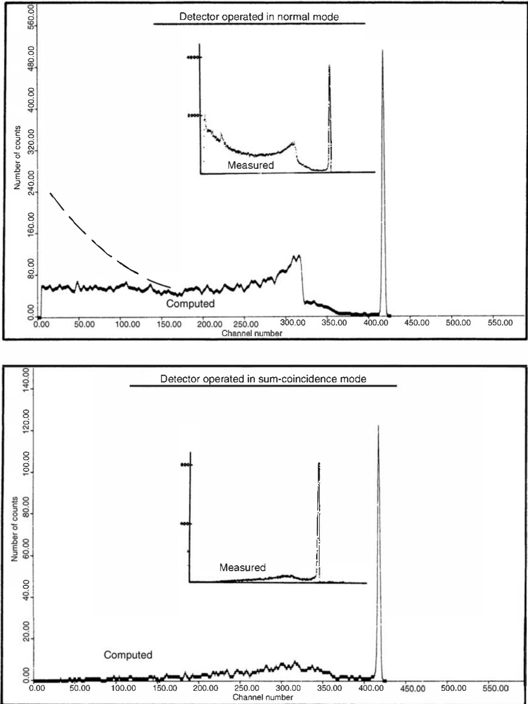
Figure 12.28 Pulse height spectra for 835 keV gamma rays from a Ge(Li) detector in normal operation (top) compared with spectra from the same detector operated in sum-coincidence mode. (From Walker and Palms. 77 )
