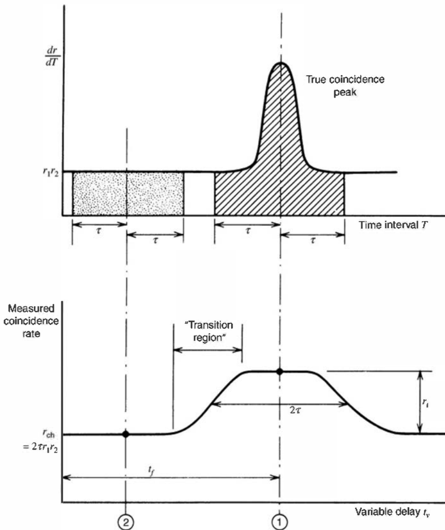
Figure 17.59 Relation between the differential time spectrum (upper plot) and the coincidence-delay curve recorded with the system of Fig. 17.58 (lower plot). The recorded coincidence rate at any specific delay value t_v is equal to the area under the differential spectrum between the limits t_v - \tau and t_v + \tau . In the lower plot, r_{ch} represents the chance coincidence rate, and r_t is the true coincidence rate.
