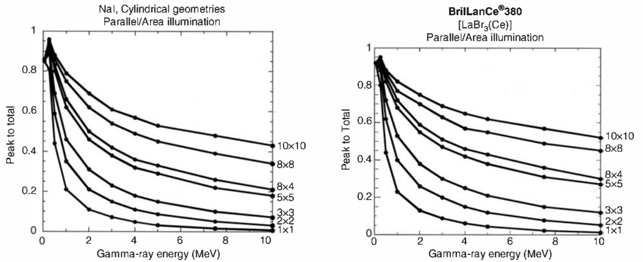
Figure 10.27 Plots of the peak-to-total ratio (or photofraction) for sodium iodide and lanthanum bromide scintillators. The size of the cylindrical detector (diameter and height in inches) is indicated for each curve. In the Monte Carlo code that generated these data, the gamma rays were assumed to be incident on the full circular area of the cylinder and parallel to the axis. (From “Efficiency Calculations for Selected Scintillators,” Saint-Gobain Ceramics and Plastics, Inc.)
