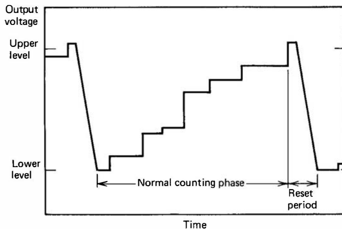
Figure 16.15 The output voltage of an active reset preamplifier. The reset phase is triggered when the voltage crosses the upper-level limit during the normal counting phase. Each upward step is a separate signal pulse.
