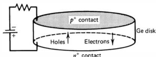
Figure 12.2 Configuration of a planar HPGe detector. The Ge semiconductor may be \nu type ( p^+ contact is rectifying), \pi type ( n^+ contact is rectifying), or lithium drifted. See Fig. 11.13 for sketches of the electric field shape for these three cases.
