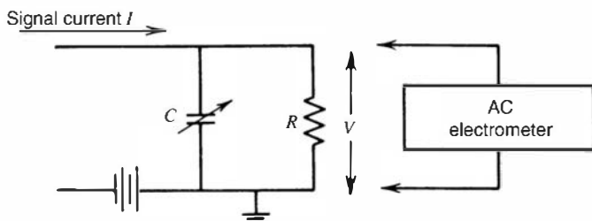
Figure 5.7 Principle of the vibrating reed electrometer. Oscillations of the capacitance induce an ac voltage that is proportional to the steady-state signal current I [see Eq. (5.7)].
