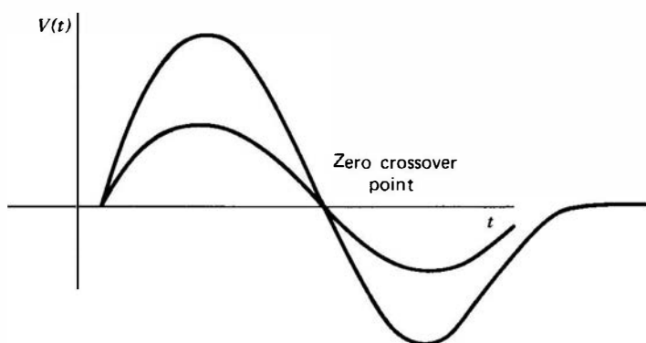
Figure 17.51 Bipolar pulses of different amplitude showing the same time of zero crossover.
