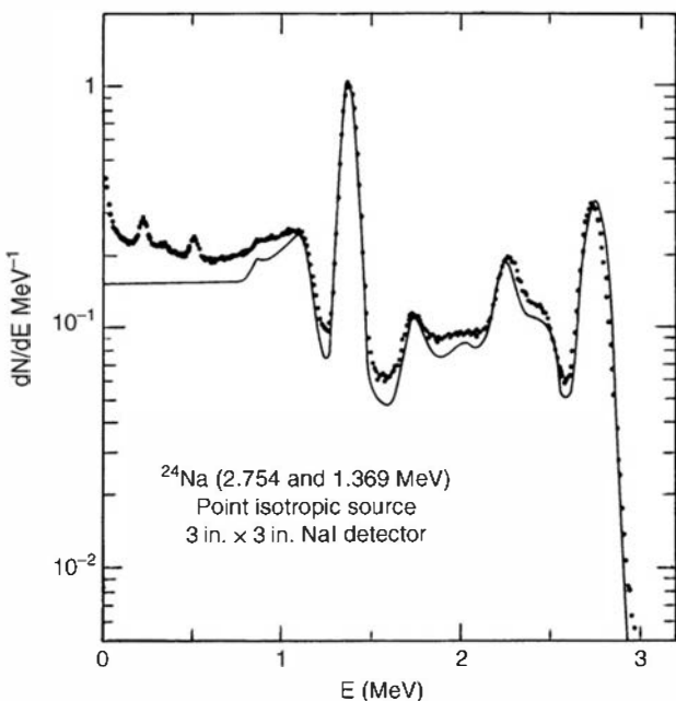
Figure 10.16 A comparison of a measured pulse height spectrum (points) with a theoretical spectrum calculated by Monte Carlo methods. (From Berger and Seltzer. 17 )
