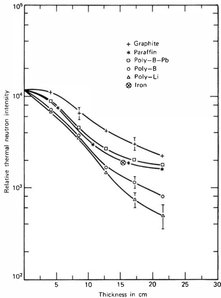
Figure 20.9 The relative effectiveness of different shielding materials for 2.6 MeV neutrons as indicated by the thermal neutron flux for various thicknesses. (From Gujrathi and D'Auria. 40 )
