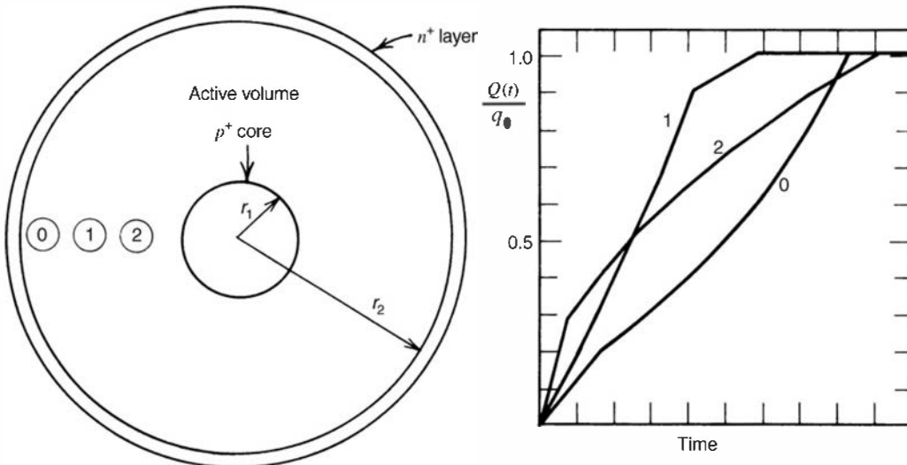
Figure 12.13 Leading edge of the output pulse for a coaxial drifted detector. Three different interaction points are indicated as 0, 1, and 2. (From Gadeken and Robertson. 21 )
