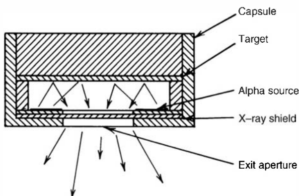
Figure 1.9 Cross-sectional view of a compact source of characteristic X-rays that utilizes alpha particle excitation of a target. (From Amlauer and Tuohy. 17 )
