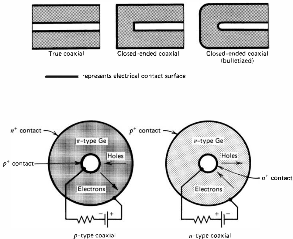
Figure 12.4 At the top are shown the three common shapes of large-volume coaxial detectors. Each represents a cross-sectional view through the axis of a cylindrical crystal. The outer electrode is extended over the flat front (left) surface in both closed-ended cases. Cross sections perpendicular to the cylindrical axis of the crystal are shown at the bottom. The HPGe material may be either high-purity p or n type. The corresponding electrode configurations are shown for each type.
