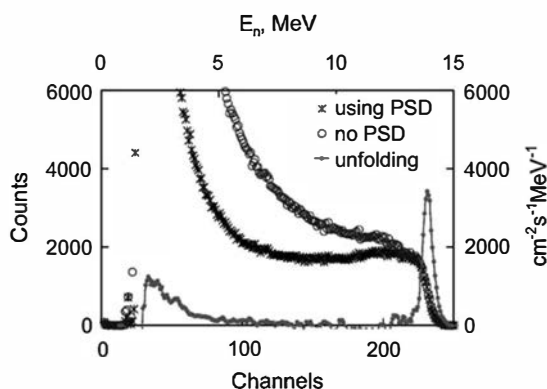
Figure 15.17 The continuous spectrum shown at the top is the pulse height spectrum measured from a liquid scintillator for a source of 14 MeV neutrons. The next lower spectrum was taken using pulse shape discrimination (PSD) to suppress pulses generated by gamma ray interactions. The spectrum at the bottom is the result of applying an unfolding code to the gamma-suppressed spectrum, and shows the peak expected at 14 MeV. (From Kaschuck et al. 112 )
