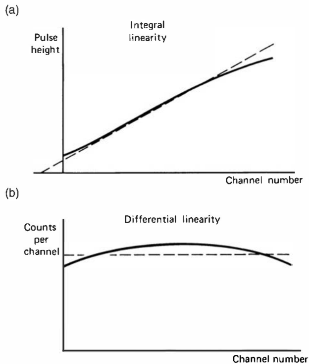
Figure 18.6 Examples of integral and differential linearity measurements for an MCA.
