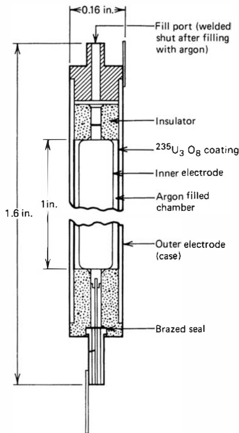
Figure 14.13 A typical in-core fission chamber used in BWR neutron monitoring systems.
