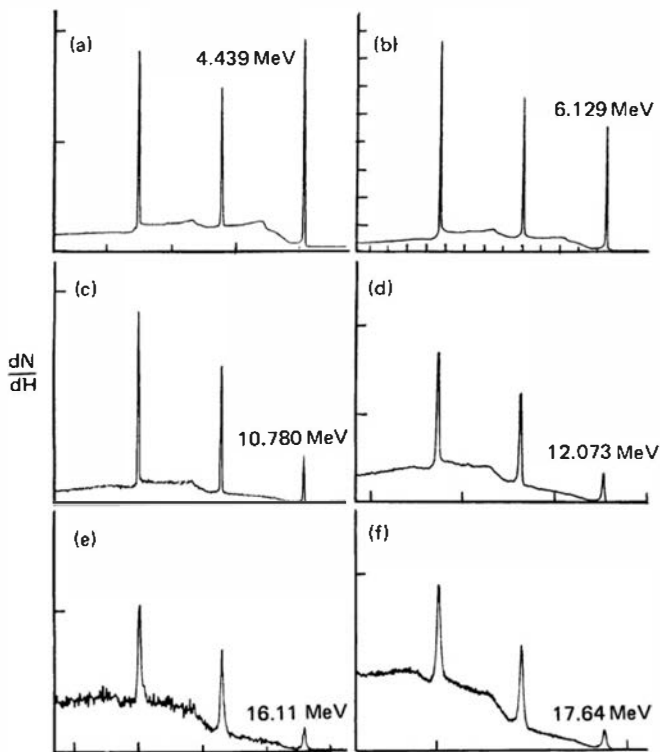
Figure 12.18 The relative intensity of the full-energy, single escape, and double escape peaks for a 100 \text{ cm}^3 Ge(Li) detector for gamma-ray energies from 4.439 to 17.64 MeV. (From Berg et al. 57 )
