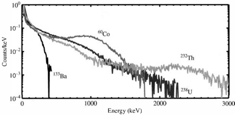
Figure 10.19 Gamma-ray spectra recorded from a plastic scintillation detector for four examples of gamma-emitting radioisotopes. (Plots courtesy of Robert Runkle, Pacific Northwest National Laboratory.)
