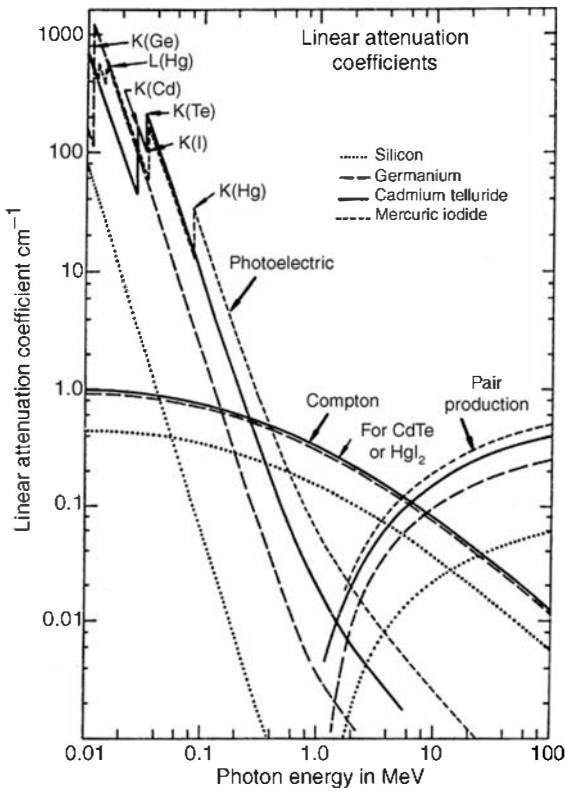
Figure 13.22 Photoelectric, Compton, and pair production linear attenuation coefficients for Si, Ge, CdTe, and HgI 2 . K-shell absorption edges are shown. (From Malm. 49 )
