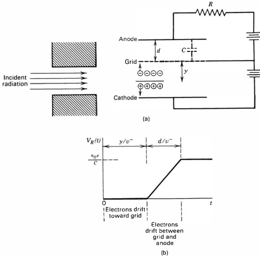
Figure 5.17 (a) Operational principle of the gridded ion chamber. All ion pairs must be formed in the lower region of the chamber between the cathode and grid. (b) The pulse shape that results from the formation of n_0 ion pairs at a distance y from the grid, where d is the grid–anode spacing [see part (a)]. The rise of the pulse results from the drift of the electrons across the grid–anode region. The pulse will decay back to zero with a time constant given by RC .
