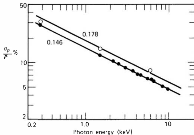
Figure 6.13 Fractional standard deviation of the peak (FWHM energy resolution/2.35) for a proportional counter filled with P-10 gas at 1 atm. Two sets of measurements are shown, one for a “standard” tungsten anode wire of 0.05 mm diameter ( \circ ) and the other for a similar wire of improved uniformity ( \bullet ). The corresponding values for \sqrt{C} (in \text{keV}^{1/2} ) in Eq. (6.25) are indicated. (From Charles and Cooke. 61 )
