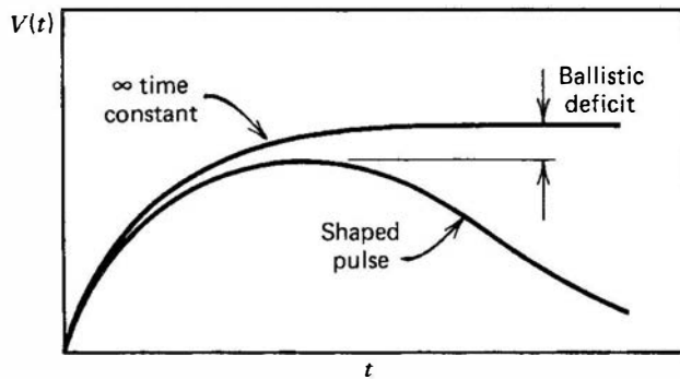
Figure 17.22 Definition of the ballistic deficit. If the shaping times are fixed, the ratio of the deficit to the amplitude of the shaped pulse will be constant for pulses of the same leading edge shape but will vary if this shape changes.
