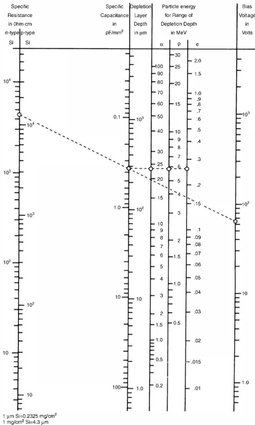
Figure 11.10 Nomogram illustrating interrelation between parameters for silicon junction detectors. (Similar to nomogram originally published by Blankenship and Borkowski. 29) )
