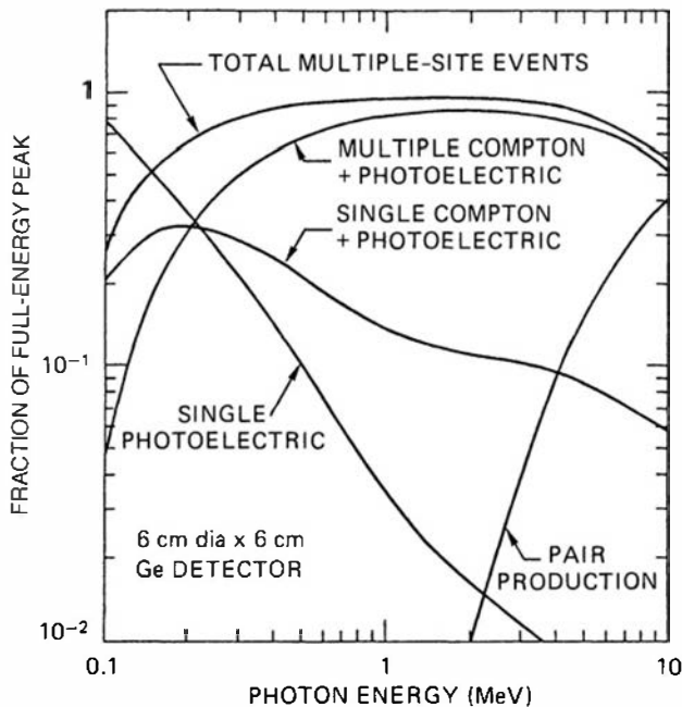
Figure 12.17 Fractions of the full-energy peak contributed by different energy loss mechanisms in a 6 cm \times 6 cm coaxial HPGe detector, as predicted by Monte Carlo simulation. Absorption of the gamma-ray photon in a single photoelectric interaction predominates only for energies below about 140 keV. (From Roth et al. 55 )
