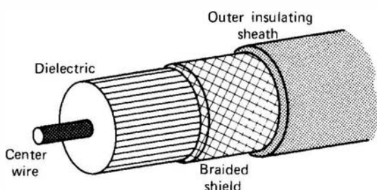
Figure 16.4 Construction of a standard coaxial cable.
