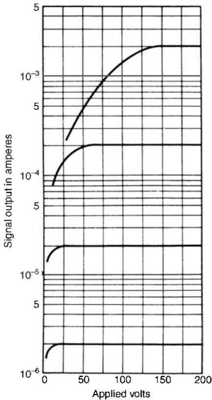
Figure 14.15 Typical current-voltage characteristics of an in-core fission chamber at different neutron irradiation levels. (Courtesy of Westinghouse Electric Corporation, Electronic Tube Division, Horseheads, NY).
