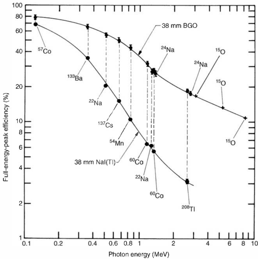
Figure 10.30 Intrinsic peak efficiencies for BGO and NaI(Tl) scintillators of equal 38 mm × 38 mm size. Radioisotope sources used for various photon energies are indicated. (From Evans and Orndoff. 50 )
