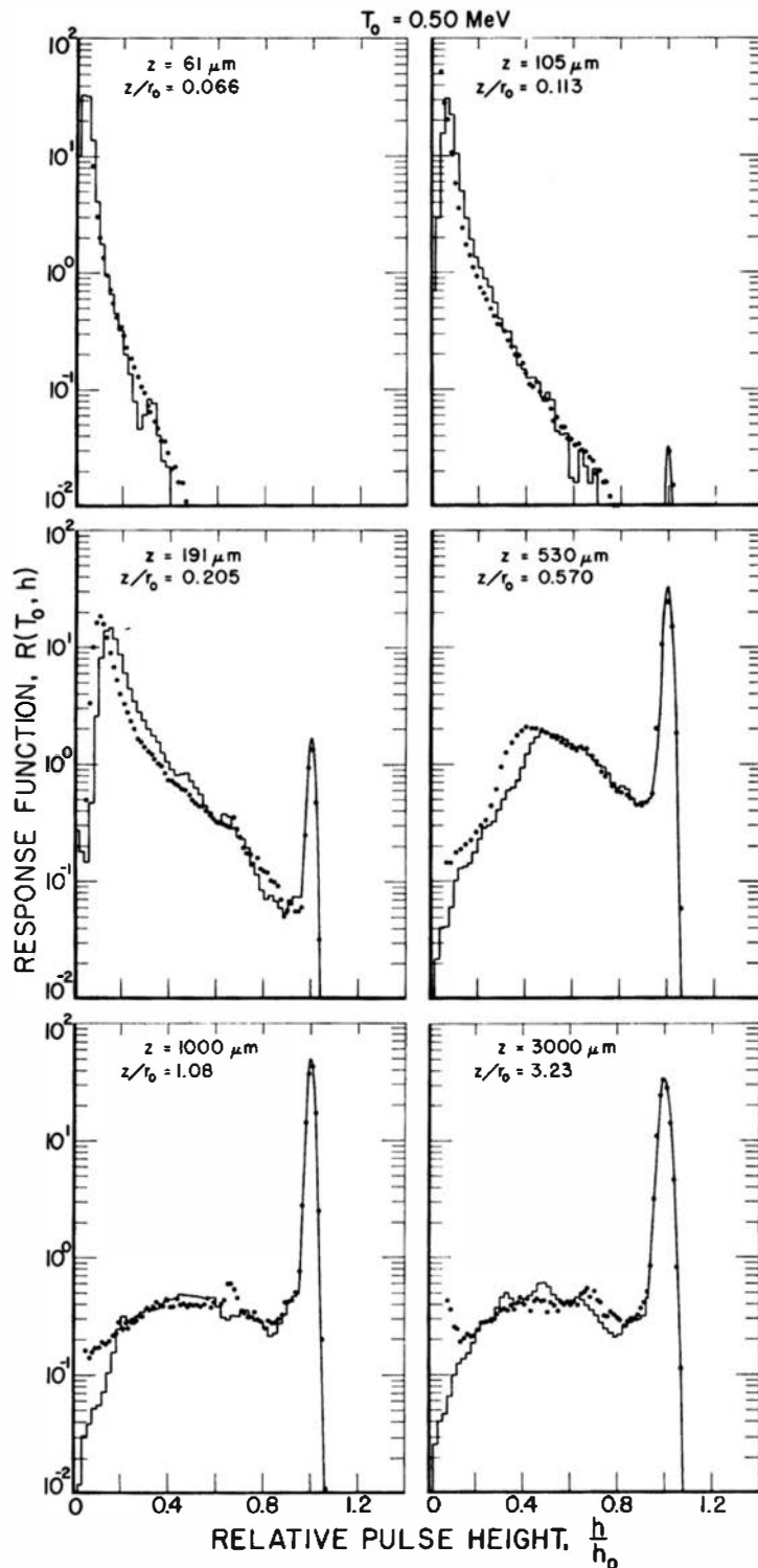
Figure 13.18 Experimental and calculated response functions for silicon detectors for 0.50-MeV electrons. The experimental data are shown as points, whereas the continuous plot is the result of a Monte Carlo calculation. z is the detector thickness, and z/r_0 is the ratio of this thickness to the mean range of the electrons. (From Berger et al. 42 )
