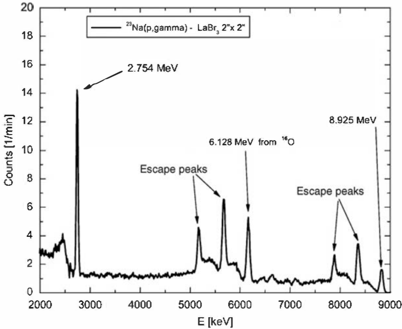
Figure 10.18 Upper portion of the pulse height spectrum from a 5.08 cm × 5.08 cm crystal of LaBr 3 (Ce). The source was a proton-induced nuclear reaction with prominent gamma ray energies emitted at 6.128 and 8.925 MeV. The full-energy, single escape, and double escape peaks for each are clearly seen. (From Ciemala et al. 18 )
