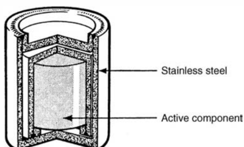
Figure 1.13 Typical double-walled construction for \text{Be}(\alpha, n) sources. (From Lorch. 20 )
