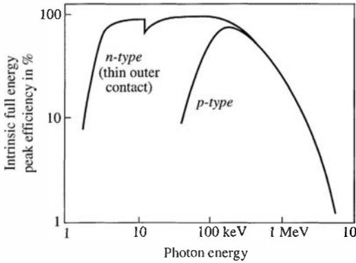
Figure 12.31 General character of the variation of intrinsic peak efficiency for coaxial germanium detectors with incident photon energy. The difference between n - and p -type detector behavior at low energies is caused by the attenuation due to different contact thicknesses.
