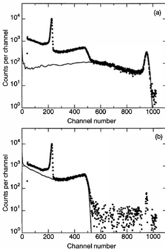
Figure 15.12 (a) The dots show a measured pulse height spectrum from a ^3\text{He} tube for monoenergetic 2.41 MeV neutrons. The predicted spectrum using a Monte Carlo model for only the ^3\text{He}(n, p) reaction is the solid line. (b) The dots now show the residual spectrum after subtraction of the ^3\text{He}(n, p) model results shown in part (a). The solid line is the model prediction for the contribution of elastic scattering. The prominent peak is from the capture of thermal and epithermal neutrons that deposit 0.764 MeV. (From Takeda et al. 75 )
