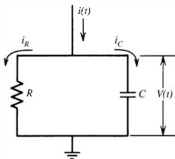
Figure 9.20 Simple parallel RC circuit representing a PM tube anode circuit.
