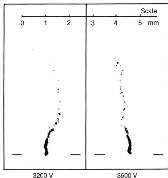
Figure 19.3 Photographs of individual SQSs for two different applied voltages. The anode position is indicated by the line segments at the bottom. (From Atac et al. 10 )
