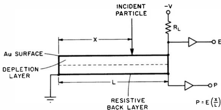
Figure 13.33 Basic configuration of a position-sensitive semiconductor detector. The position signal (labeled P ) is obtained by resistive charge division from the back layer. The E signal is proportional to the energy deposited by the particle in the detector active volume. (From Kaufman et al. 162 )
