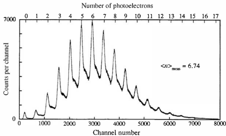
Figure 9.24 Pulse height spectrum taken from a hybrid photomultiplier tube when illuminated by light pulses of low intensity. Separate peaks can be distinguished for events that originate from the discrete number of photoelectrons shown along the top of the plot. (From D'Ambrosio et al. 106 )
