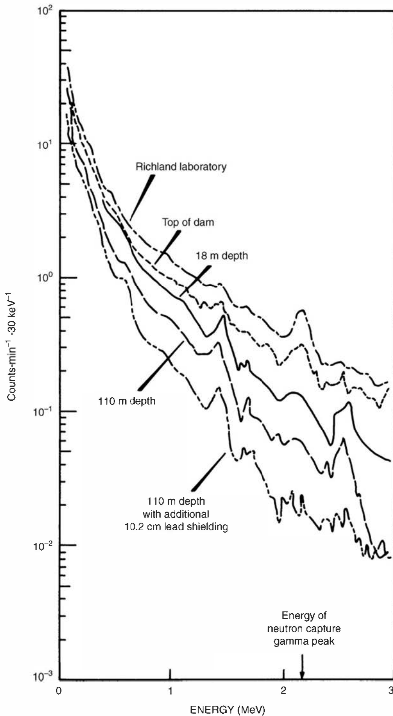
Figure 20.8 The background spectra from a 7.62 cm \times 7.62 cm NaI(Tl) scintillator within a paraffin and 10.2-cm-thick lead shield. The indicated locations are at different depths within the massive concrete structure of Grand Coulee Dam. The purpose of the paraffin was to indicate the importance of the neutron component by the relative prominence of the hydrogen capture gamma-ray peak at 2.22 MeV. (From Kaye et al. 31 )
