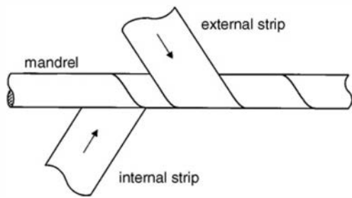
Figure 6.7 The fabrication of a straw tube from two foil strips. Adhesive is used to bind the strips together into a rigid tube. (From Marzec et al. 9 )
