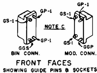
Figure A.1 Pin assignments for the NIM standard connector between bin and module. (Adapted from National Bureau of Standards Photo 74-08-4044.)
