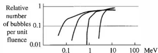
Figure 19.22 Response curves of a set of bubble detectors with differing degrees of superheat. The differences in these curves can be used as the basis of an unfolding process to estimate the important components of the neutron energy spectrum.
