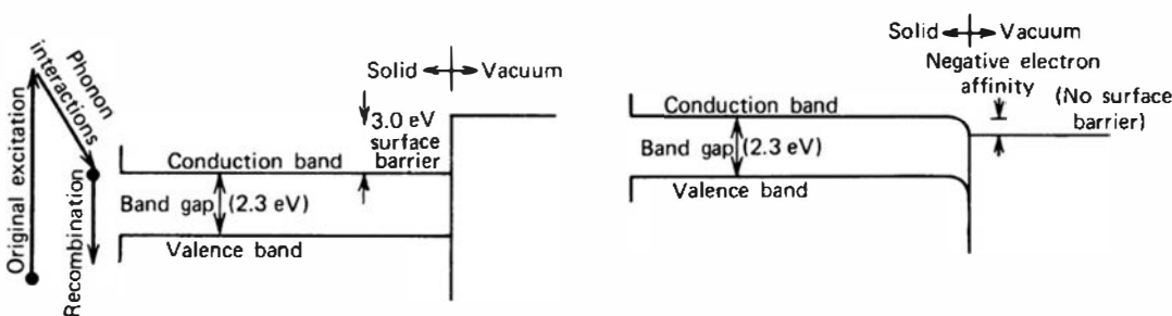
Figure 9.4 Band structure near the surface for conventional semiconductors (left) and NEA materials (right). (Adapted from Krall et al. 10 )
