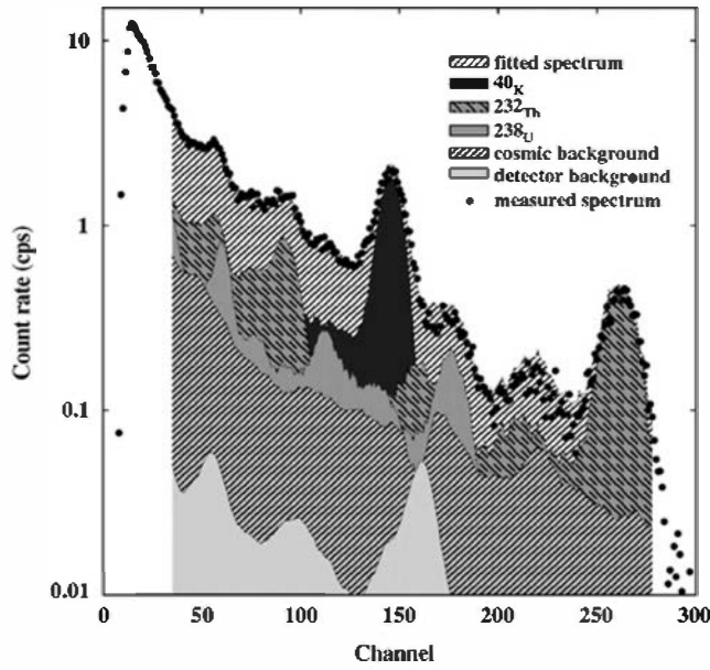
Figure 20.3 Background spectrum measured from a 12.7 cm diameter by 15 cm cylindrical BGO scintillator located over an asphalt surface. The separate contributions of naturally occurring gamma rays, cosmic rays, and radioactivity of the detector itself are shown. (From van der Graaf et al. 21 )
