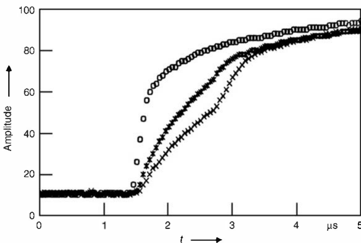
Figure 14.7 Variation in the digitized pulse leading edge from a ^3\text{He} tube due to differences in the orientation of the proton-triton tracks with respect to the anode wire. (From Dietz and Sosaat. 50 )
