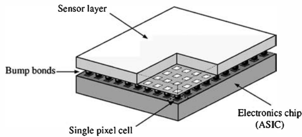
Figure 16.11 Sketch of the readout of a pixel detector using the Medipix ASIC. Each pixel from the sensor is coupled to a corresponding readout channel of the ASIC using individual conducting bump bonds. (From Michel et al. 11 )
