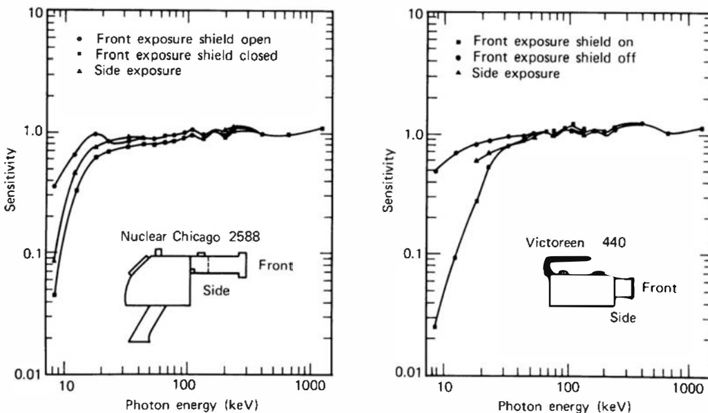
Figure 5.12 Energy calibration of two different gamma-ray survey meters. (From Storm et al. 17 )
