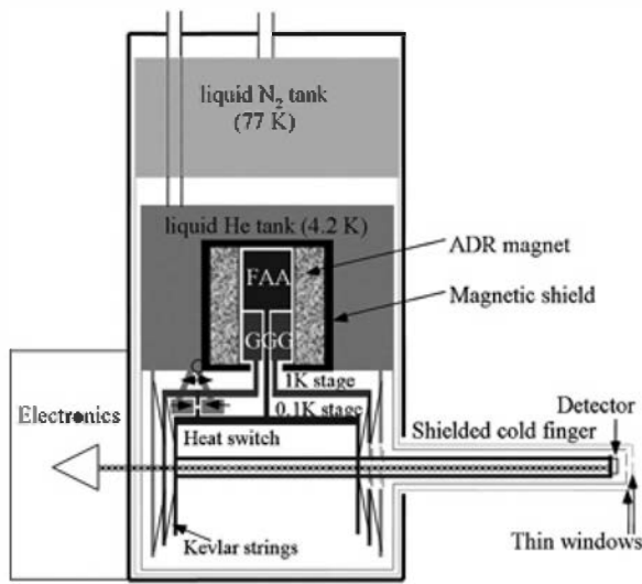
Figure 19.6 Schematic of a two-stage adiabatic demagnetization refrigerator (ADR) with liquid nitrogen and liquid helium precooling. The detector is held at \sim 0.1 K at the end of a shielded cold finger behind several thin windows that block thermal radiation while transmitting the radiation of interest. (From Friedrich et al. 61 )
