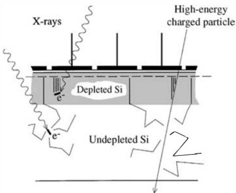
Figure 13.41 Schematic representation of the diffusion of electrons following their interaction in a partially depleted CCD. Electrons created in the depleted region are less likely to be spread among multiple pixels than those that are formed in the undepleted region because of their rapid collection caused by the strong electric field in the depleted region.
