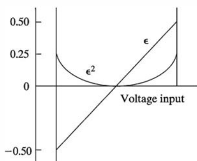
Figure 17.41 The top plot shows the ideal conversion between analog voltage input and the output code of an ADC. The bottom plot shows the quantization error \epsilon (in units of code width), together with the square of its value \epsilon^2 .
