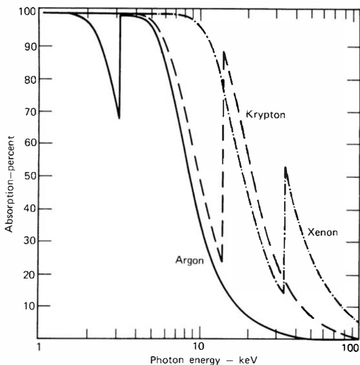
Figure 6.18 Fraction of incident photons absorbed in a 5.08-cm layer of several proportional gases at 1 atm pressure.
