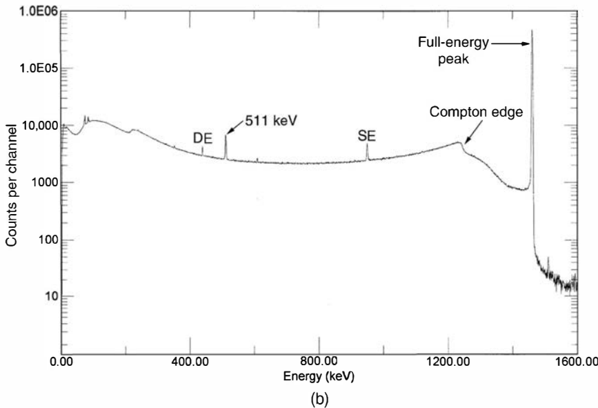
(b) Spectrum from 1460 keV gamma rays emitted by ^{40}\text{K} that now shows the additional effects of pair production taking place in the detector and surrounding materials. Both single escape (SE) and double escape (DE) peaks can be seen, along with the peak at 511 keV due to annihilation radiation produced by pair production interactions in surrounding materials.
