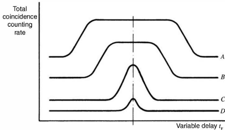
Figure 17.60 Coincidence-delay curves for different values of the coincidence resolving time \tau . Curve A corresponds to the largest value of \tau , curve D to the smallest. Values of \tau larger than half the width (at its base) of the prompt coincidence peak in the differential time spectrum of Fig. 17.59 lead to the flat-topped plateau shape of curves A and B . In curve C , \tau is just equal to this value and the full true coincidence rate is obtained only at one specific delay value. In curve D , \tau is too small to obtain all the true coincidences at any delay value.
