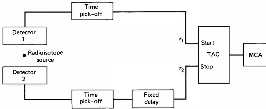
Figure 17.56 A simplified system to record multichannel time spectra from a radioisotope source emitting coincident radiation.
