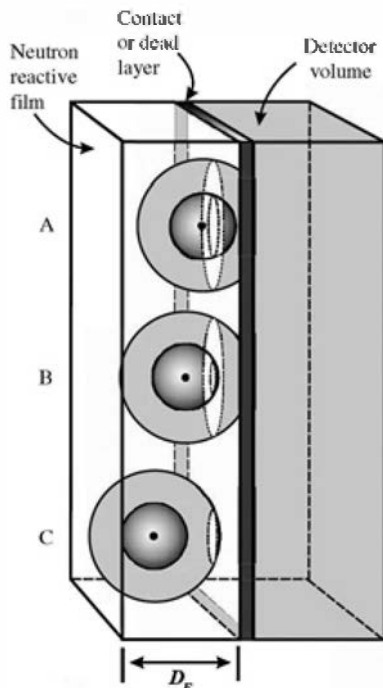
Figure 14.5 Sketch of a converter layer of thickness D_F in contact with a semiconductor detector. A thin electrical contact or dead layer that is normally present on the surface of the detector is also shown. The three cases labeled A, B, and C represent neutron interaction points at varying depths in the converter layer. The spheres sketched around each interaction point represent the maximum range of the two reaction products (the alpha particle and recoil lithium nucleus for the ^{10}\text{B} reaction). For case A, the interaction is near the interface, and either reaction product has a reasonable probability of reaching the detector active volume. In case B, the short-range particle (the lithium recoil) has only a low probability of reaching the detector. For case C, the short-range particle can no longer reach the detector, and the probability that the longer-range particle (the alpha particle) is detected is now much lower than in the previous cases. (From McGregor et al. 33 )
