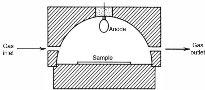
Figure 6.8 Diagram of a 2\pi gas flow proportional counter with a loop anode wire and hemispherical volume. The sample can often be inserted into the chamber by sliding a tray to minimize the amount of air introduced.
