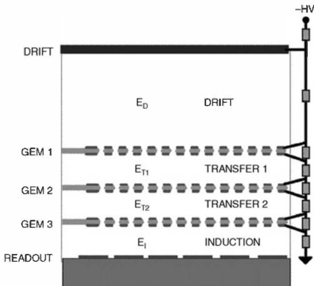
Figure 6.30 Arrangement of three GEM foils in cascade. The original ionization occurs in the region labeled DRIFT, and the ionization electrons are drawn downward to the first GEM foil. The amplified electrons emerging from GEM 1 are drifted to GEM 2 where they again multiply. One more GEM stage provides further amplification, and its output is collected at the readout plane that can be a gas microstrip structure or other readout pattern. The resistor chain at the right provides appropriate voltage differences between elements from a single high-voltage supply. (From F. Sauli. 150 )
