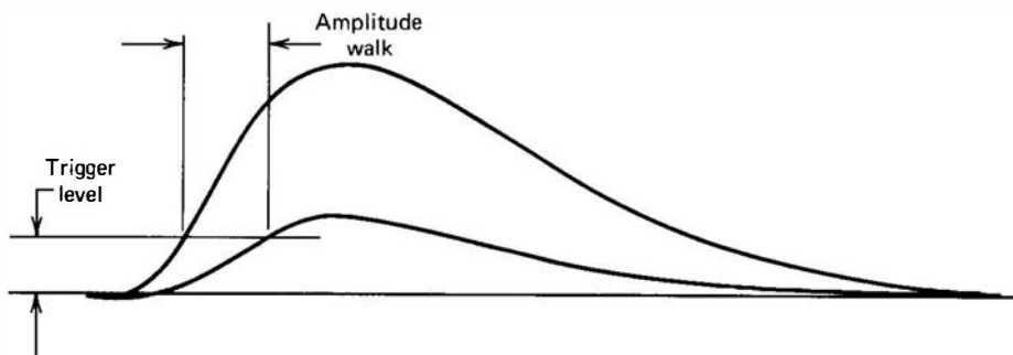
Figure 17.49 Amplitude walk in leading edge triggering. Two pulses with identical shape and time of occurrence but different amplitude are seen to cross the trigger level at different times.
