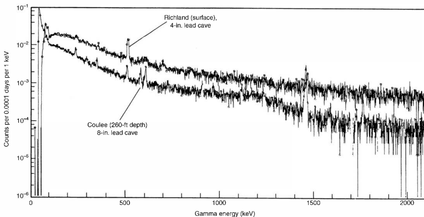
Figure 20.5 The top curve shows the background spectrum recorded for an 85-cm 3 germanium detector in a normal laboratory using the shielding shown on Fig. 20.4. The bottom curve shows the gains achieved by relocating the counter deep inside the massive concrete structure of a dam and increasing the thickness of the lead shielding. (From Kaye et al. 16 )
