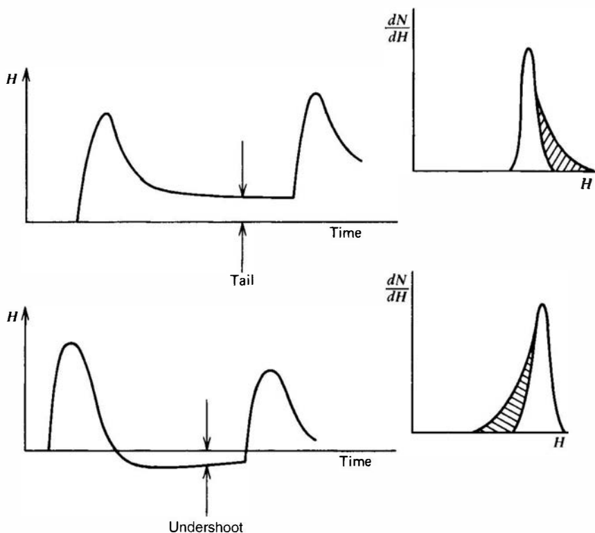
Figure 17.28 Pile-up from the tail or undershoot of a preceding pulse. Both are usually categorized as tail pile-up. The effect on the differential pulse height spectrum for constant-amplitude pulses is shown as the cross-hatched area at the right.
