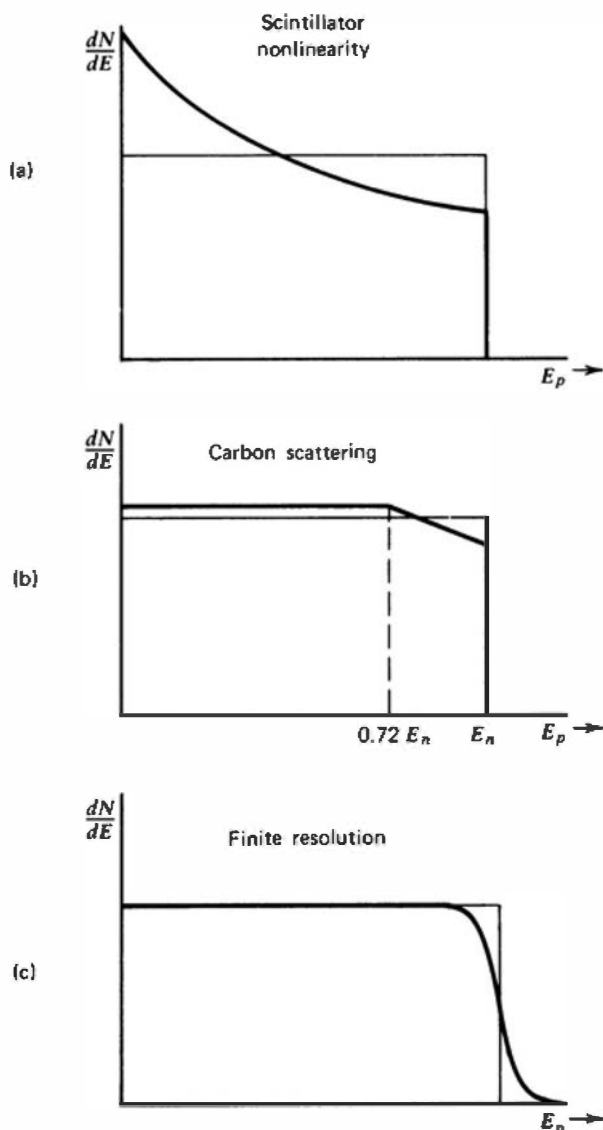
Figure 15.19 Distortions to the rectangular recoil proton energy spectrum due to three separate factors.
