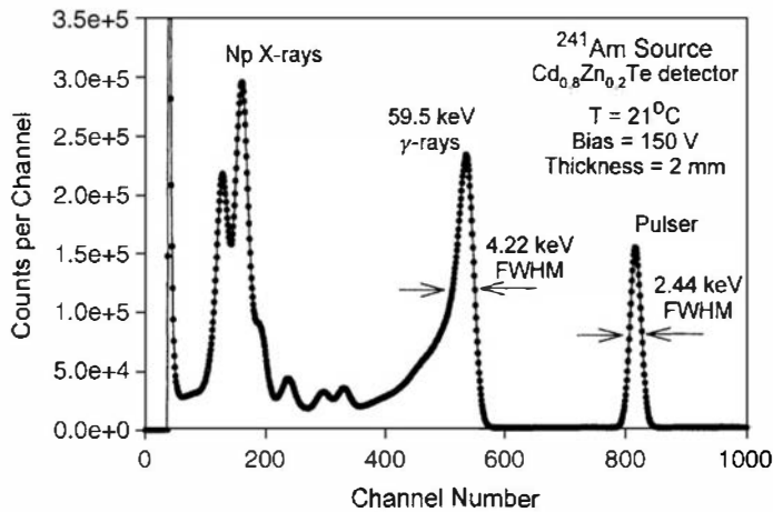
Figure 13.29 Pulse height spectrum from a 5 mm × 5 mm × 2 mm thick planar CdZnTe detector. (From McGregor and Hermon. 50 )
