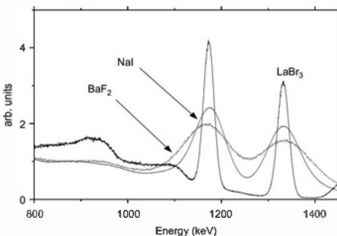
Figure 8.14 Comparison of the ^{60}\text{Co} pulse height spectrum measured with 1-inch \times 1-inch \text{LaBr}_3 , NaI, and \text{BaF}_2 (From Nicolini et al. 215 ).
