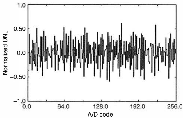
Figure 17.39 The differential nonlinearity (as defined in the text) plotted versus ADC code for an 8-bit flash ADC. (From Crawley et al. 53 )
