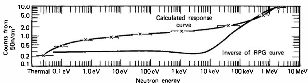
Figure 15.4 Calculated sensitivity of a 10-in. (25.4 cm) diameter moderating sphere, together with the relative dose per neutron (inverse of RPG curve). (From Hankins. 17 )
