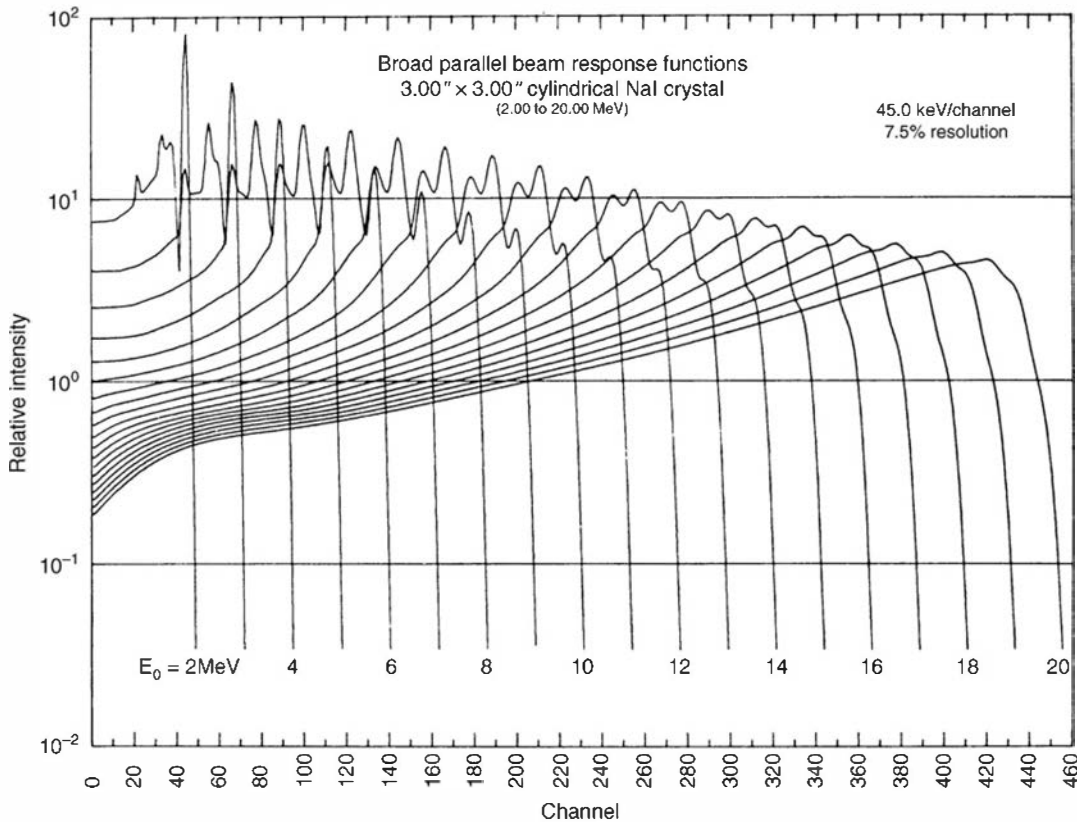
Figure 10.17 Calculated response functions for a NaI(Tl) scintillation detector extending to 20 MeV. (From Berger and Seltzer. 17 )
