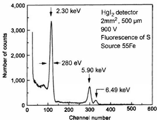
Figure 13.28 Example of a measured pulse height spectrum from a \text{HgI}_2 detector. (From Ponpon and Sieskind. 76 )
