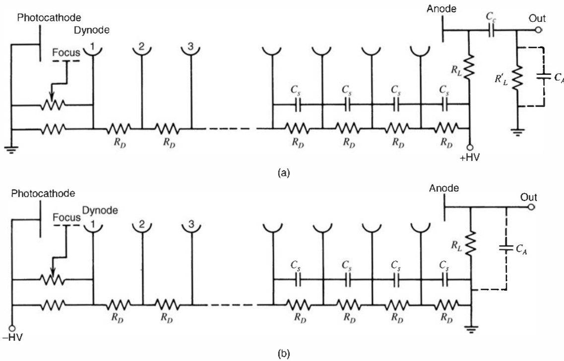
Figure 9.14 Typical wiring diagrams for the base of a PM tube. Scheme (a) utilizes positive high voltage and a grounded photocathode. Scheme (b) uses negative high voltage, and the photocathode must be isolated from ground. Values of the divider string resistors R_D are chosen using criteria given in the text. The equivalent anode load resistance is R_L in (b), and the parallel combination of R_L and R'_L in (a). Other identifications are given in the text.
