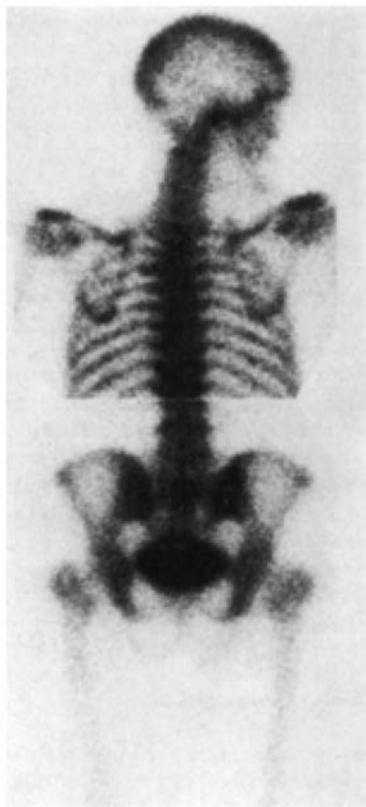
Figure 10.35 Example of a human bone scan produced by using a gamma camera to image the distribution of methylene diphosphonate labeled with ^{99m}\text{Tc} . The upper and lower halves of the image each were produced by recording approximately 10^6 counts over a 3-min period. (Courtesy of W. L. Rogers, University of Michigan Medical Center.)
