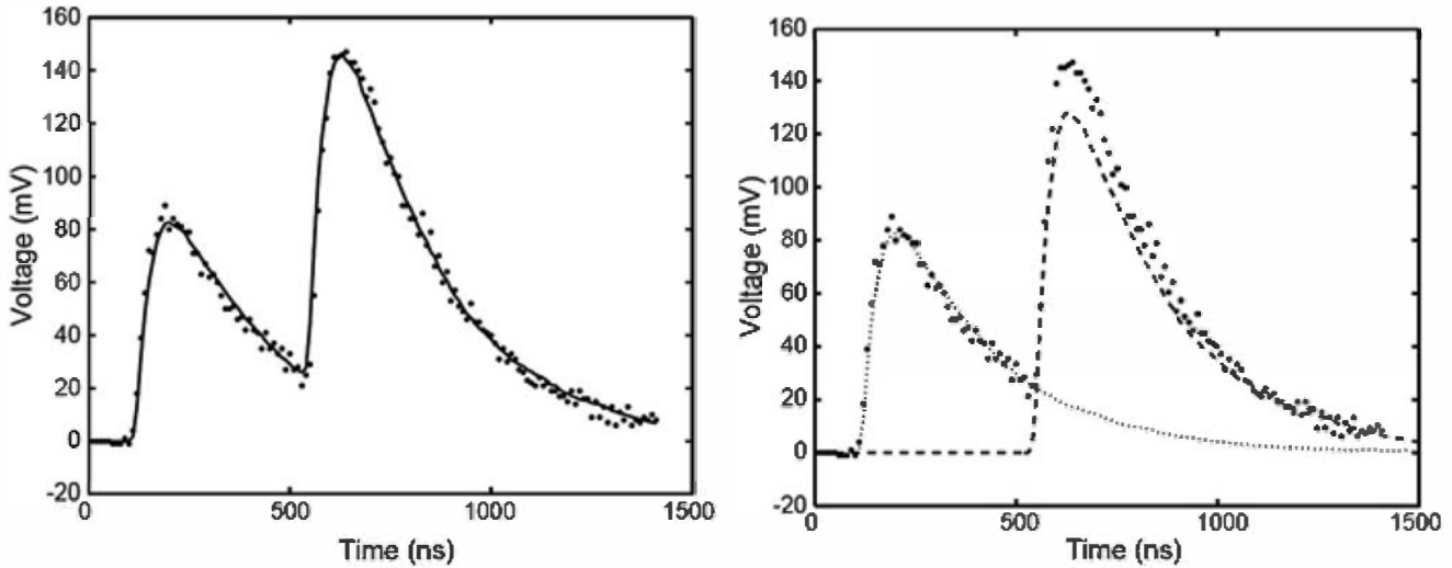
Figure 17.47 Pulses digitized directly from a photomultiplier tube viewing a NaI(Tl) scintillator. Two events have occurred in the scintillator, the second before the light from the first has completely decayed. Recovery of the information carried by both events is possible by deconvolving the individual components of the pile-up that has occurred. (From Scott et al. 66 )
