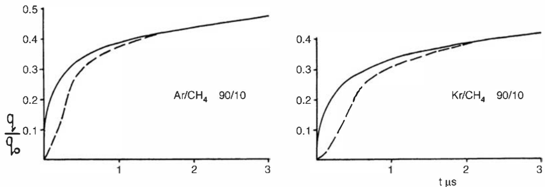
Figure 6.16 Shape of the output pulse leading edge calculated for a typical tube for two different proportional counter gases. In each case, the solid curve represents initial ionization formed at a single radius (constant drift time), whereas the dashed line assumes uniform ionization along a diameter. (From Gott and Charles. 73 )
