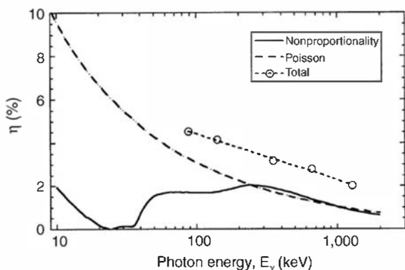
Figure 10.23 A comparison of the predicted contributions of scintillator nonproportionality and Poisson photoelectron statistics to the energy resolution of a 2.54 cm × 2.54 cm NaI(Tl) scintillator. The points labeled “Total” are measured resolution values. (From Valentine et al. 25 )
