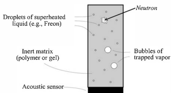
Figure 19.21 Principle of the bubble detector for neutrons. The acoustic sensor converts the device into an active detector.
