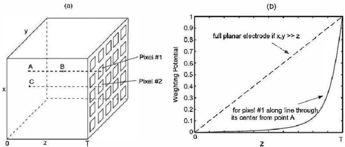
Figure D.1 (a) A planar detector configuration with a continuous cathode electrode on the x - y surface at the left and a pixelated anode surface on the right. (b) Plot of the weighting potential for a continuous anode (dashed line) and for a single pixel anode (solid line), for the case in which the pixel size is 20% of the detector thickness T .
