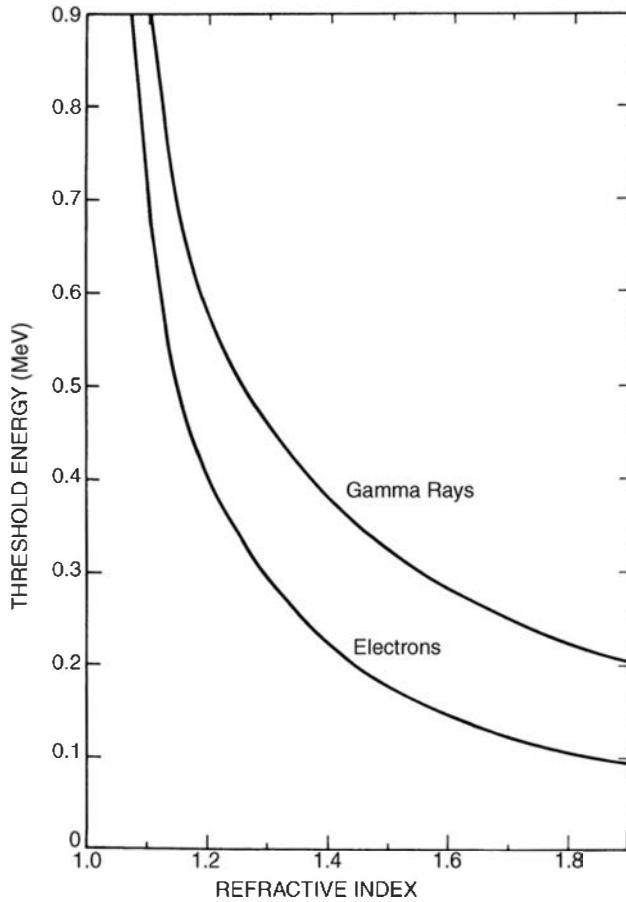
Figure 19.1 The threshold energy for Cherenkov radiation as a function of the index of refraction of the detection medium. Curves are shown both for electrons and for gamma rays that can yield, by 180^\circ Compton scattering, an electron of the threshold energy. (From Sowerby. 2 )
