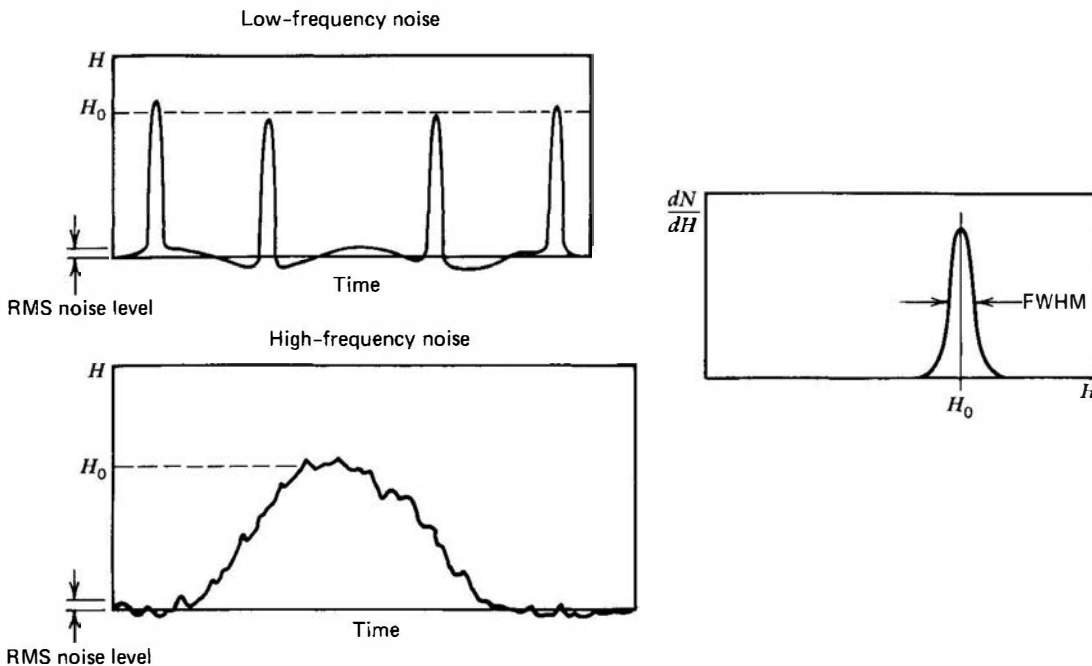
Figure 17.23 Sketches of the effect of low-frequency and high-frequency noise on signal pulses of constant amplitude. The effect is to broaden the peak recorded in the differential pulse height spectrum for these pulses. The FWHM of the peak of Gaussian-distributed noise will be equal to the RMS noise level multiplied by a shape factor of 2.35, provided noise is the only factor in broadening the peak.
