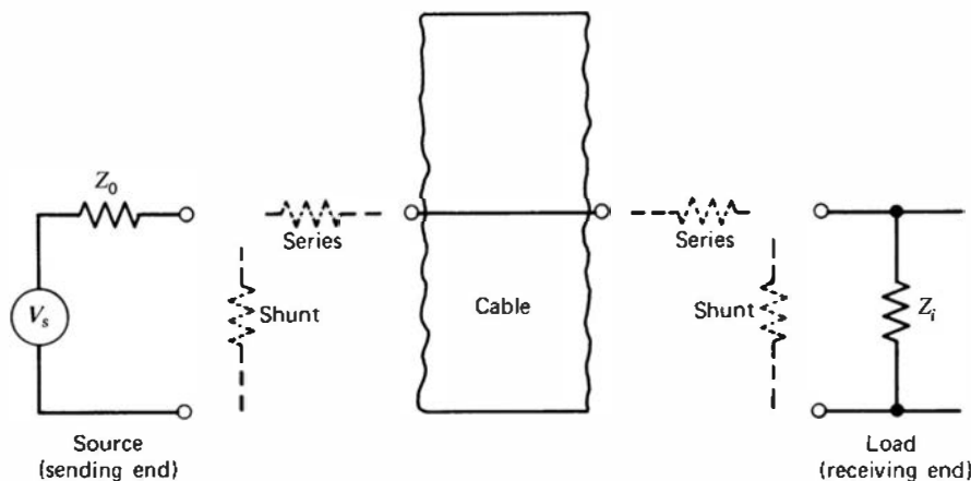
Figure 16.7 Methods of inserting terminators at either end of a coaxial cable.
