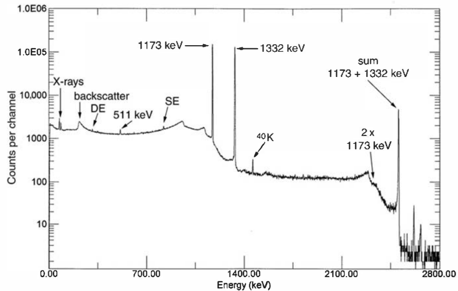
Figure 12.20 Pulse height spectrum from 1173 keV and 1332 keV gamma rays emitted by ^{60}\text{Co} measured using a p -type HPGe detector with 110% relative efficiency. Evident in the spectrum are characteristic X-rays from photoelectric absorptions in the lead shield, the backscatter peak, barely perceptible single escape (SE) and double escape (DE) peaks from pair production interactions of the 1332 keV gamma ray (the escape peaks are weak because the 1332 keV gamma ray energy is only slightly above the threshold for pair production), a peak at 511 keV from annihilation radiation produced in the shield, the Compton edges and full-energy peaks from the two primary gamma rays, a small peak at 1460 keV from ^{40}\text{K} in the background, a small “shoulder” from the summing of two 1173 keV events through pile-up, a pronounced sum peak at 2506 keV due to the full absorption of both primary gamma ray photons that are emitted in coincidence, a small peak at 2614 keV from ^{228}\text{Th} in the background, and a very small sum peak at 2665 keV from the pile-up of two 1332 keV pulses. (Spectrum courtesy R. Keyser, EG&G ORTEC, Oak Ridge, Tennessee.)
