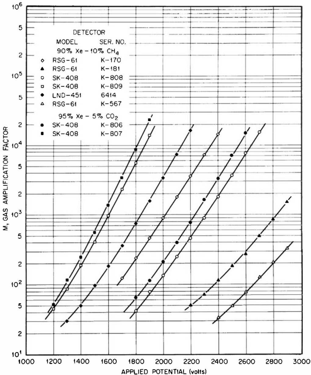
Figure 6.11 Variation of the gas multiplication factor M with voltage applied to various proportional counters. The tubes differ in their physical characteristics, but only the two indicated gases were used. (From Hendricks. 51 )
