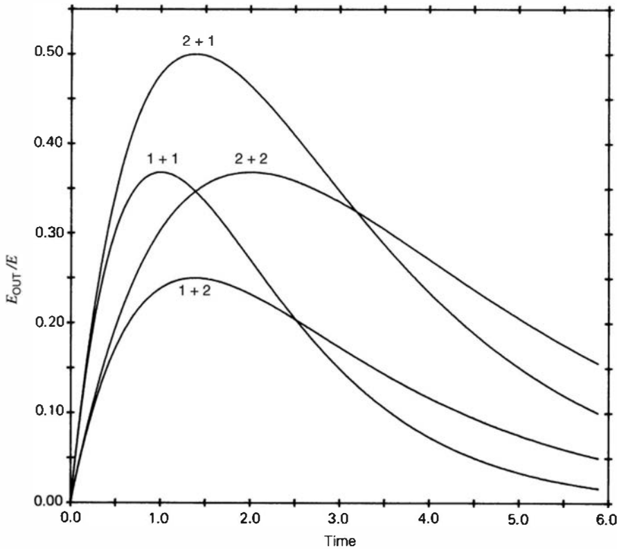
Figure 17.5 The response of a CR - RC network to a step voltage input of amplitude E at time zero. Curves are shown for four pairs of differentiator + integrator time constants. Units of the time constants and time scale are identical.
