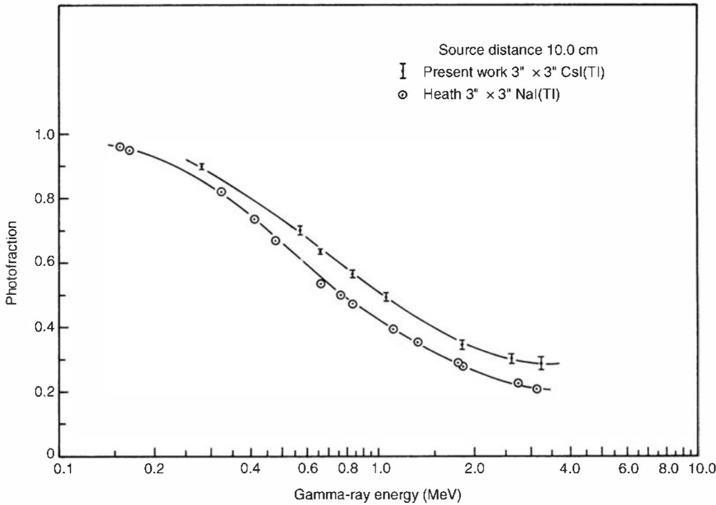
Figure 10.29 Experimental photofractions of 7.62 cm × 7.62 cm cylindrical crystals of CsI(Tl) and NaI(Tl). (From Irfan and Prasad. 49 )
