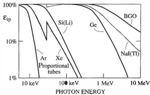
Figure 12.34 The general dependence of intrinsic full-energy peak efficiency on incident photon energy for a number of common detectors used for X- and gamma-ray spectroscopy. The curves are to be interpreted as showing broad trends only, and there will be large differences between specific detectors within each of the categories shown.
