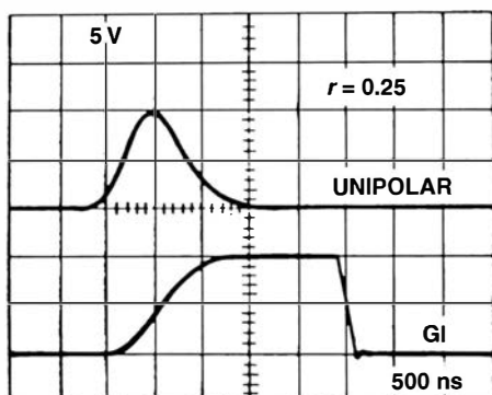
Figure 17.36 Waveforms in the operation of a gated integrator. The unipolar output of a standard Gaussian shaping network is integrated in an active circuit to give the waveform shown in the lower plot. (From Britton et al., IEEE Trans. Nucl. Sci. NS-31(1) , 455 (1984).)
