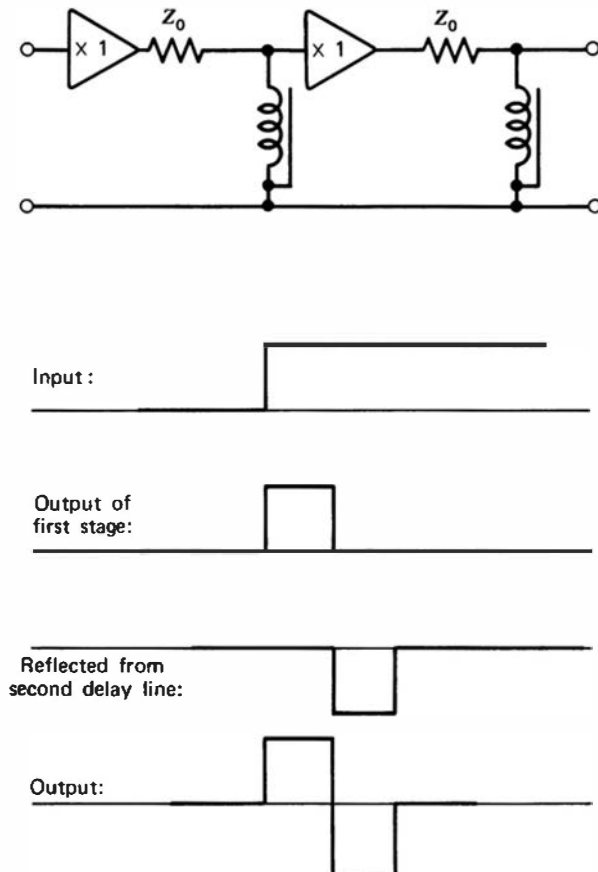
Figure 17.15 A double delay line (DDL) shaping network with equal delay times applied to a step input waveform.
