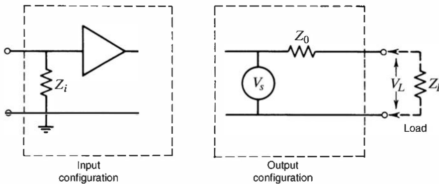
Figure 16.3 Idealized input and output configurations. For the input configuration, the triangle represents an ideal operational amplifier with infinite input impedance. Therefore, the effective device input impedance is Z_i . For the output configuration, Z_0 represents the output impedance in series with an ideal voltage generator V_S .
