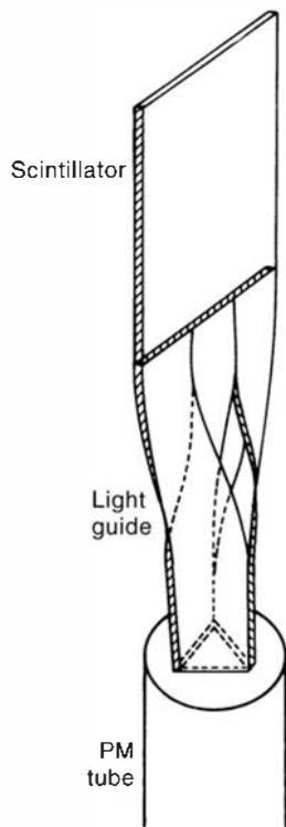
Figure 8.18 A strip light guide can be used to couple the edge of a large, flat scintillator to a PM tube.
