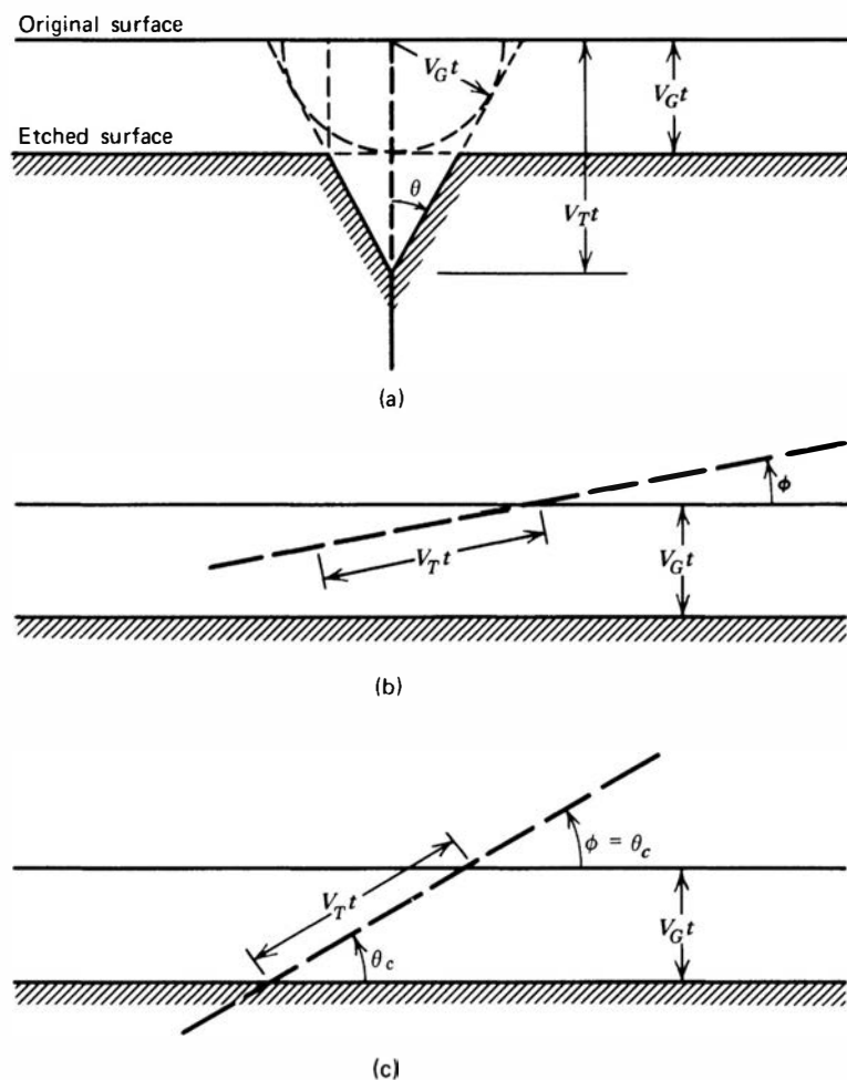
Figure 19.20 (a) Model of track etching in which the normal surface is removed at a velocity V_G and the damaged track at a velocity V_T , leading to a cone-shaped pit. (b) Tracks formed at an angle \phi less than the critical angle \theta_c are not revealed because the normal surface advances faster than the etch rate along the track. (c) The case in which the particle enters at the critical angle \theta_c . Tracks entering the surface at an angle greater than the critical angle will be visible after etching. (From R. L. Fleischer, P. B. Price, and R. M. Walker, Nuclear Tracks in Solids . Copyright 1975 by The Regents of the University of California; reprinted by permission of the University of California Press.)
