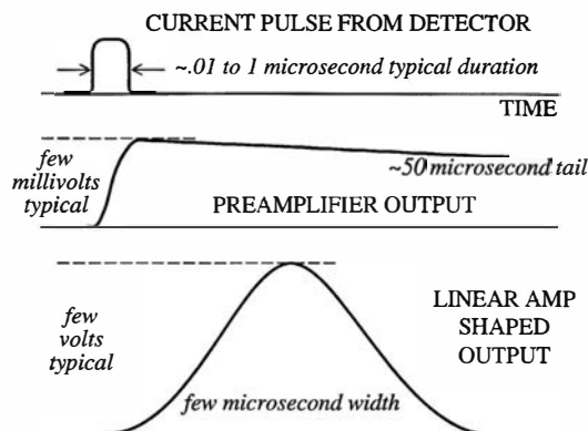
Figure 17.17 Intercomparison of typical pulses at sequential points along the signal processing chain.
