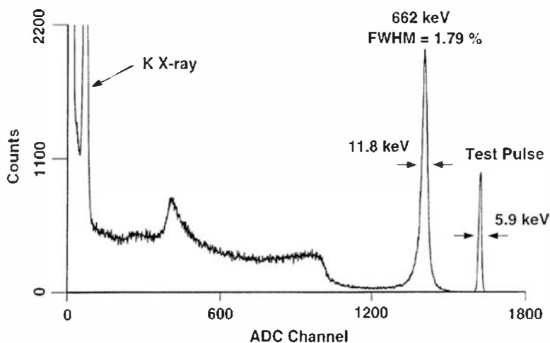
Figure 13.30 Pulse height spectrum for 662-keV gamma rays taken with a 1-cm 3 CdZnTe spectrometer operated with coplanar grid electrodes. (From He et al. 89 )
