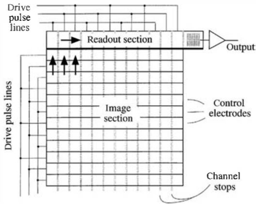
Figure 13.39 Layout of the surface of a CCD.
