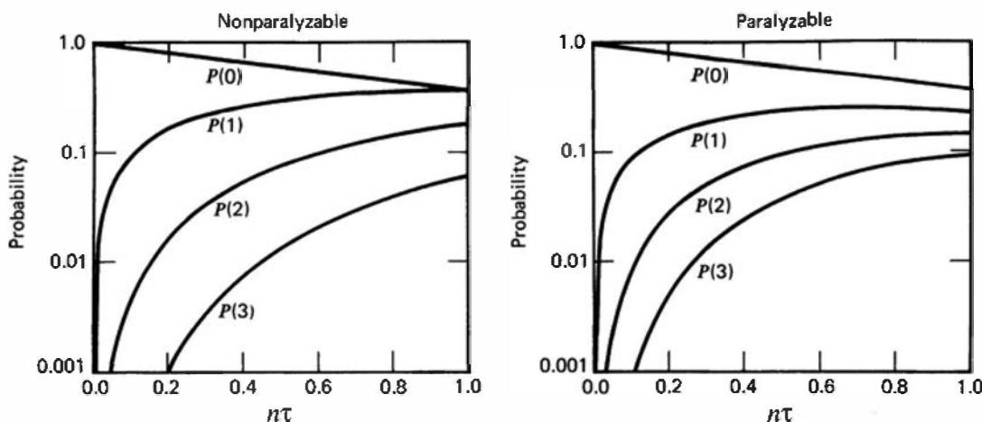
Figure 17.32 Plots of the probabilities that a recorded count is free of pile-up [ P(0) ] or due to i th-order pile-up [ P(i) ]. The abscissa is the product of true event rate n and the pile-up resolution time \tau . The left plot is from Eq. (17.34) for nonparalyzable systems, and the right plot is from Eq. (17.37) for paralyzable systems.
