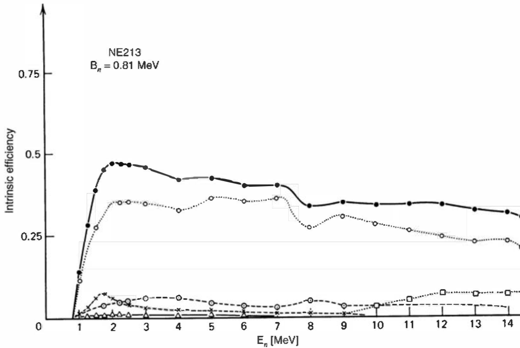
Figure 15.21 The calculated efficiency of a NE213 liquid scintillator (1.9-cm radius, 10-cm length) for a discrimination level of 0.81 MeV. Identification of the symbols is as follows: (●) combined efficiency from all processes; (○) single hydrogen scattering; (×) n-H, n-H double scattering; (⊙) n-C, n-H double scattering; (△) n-C, n-H, n-H triple scattering; (□) (n, α) and (n, n')3α reactions. (From Hermsdorf et al. 123 )
