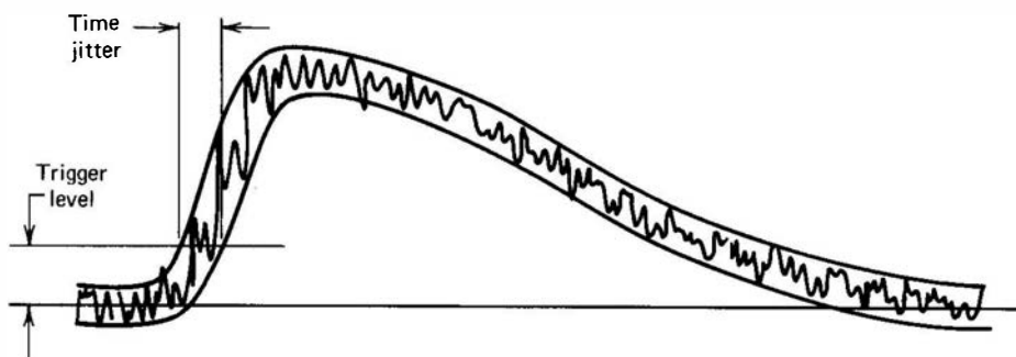
Figure 17.48 The time jitter in leading edge triggering arising from random noise. An envelope is shown of many repeated signal pulses of the same amplitude and shape, but with a random contribution of noise.
