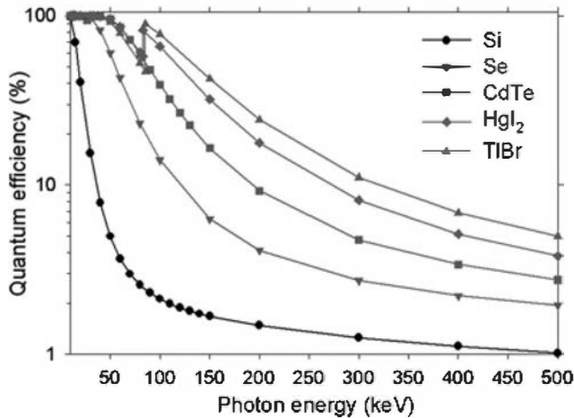
Figure 13.44 Calculated X-ray quantum efficiency values for 500 \mu\text{m} thick semiconductor materials.
