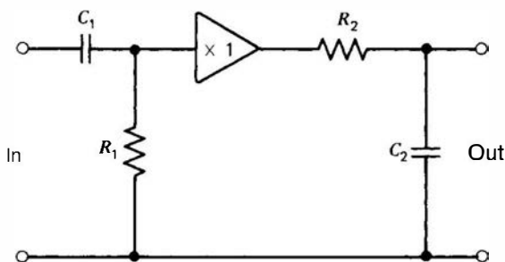
Figure 17.4 A shaping network consisting of sequential differentiating and integrating stages, sometimes denoted a CR-RC network.
