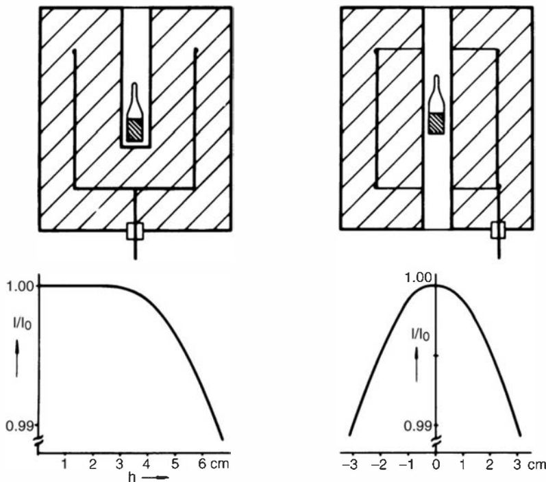
Figure 5.13 Ionization chambers used for calibration of gamma-ray sources. The curve below each configuration shows the behavior of the ionization current for small displacements of the source position. (From Weiss. 19 )
