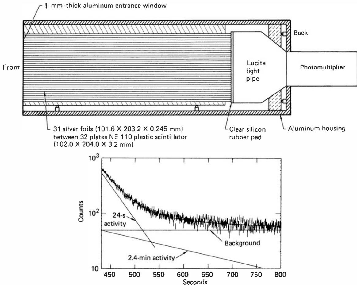
Figure 19.24 Example of a specific design for a silver activation counter. When used with fast neutrons, the counter is normally placed within a polyethylene moderator. The plot shows the counting rate observed for a period from 450 to 800 s following exposure to a fast neutron flux. (From Slaughter and Pickles. 173 )
