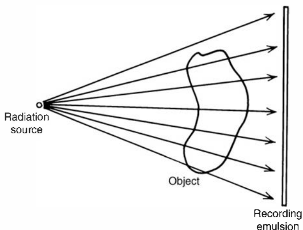
Figure 19.12 The elements in the formation of a radiographic image.
