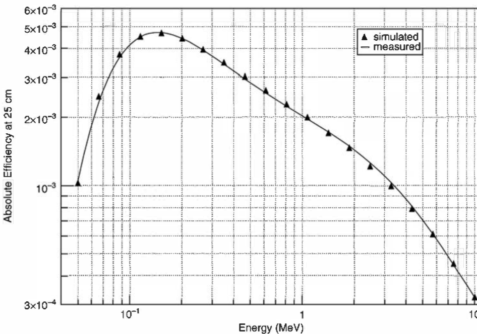
Figure 12.32 Plot of the absolute full-energy peak efficiency for a point source 25 cm in front of a p -type HPGe coaxial detector with 139% relative efficiency as defined later in this chapter. The germanium crystal has a diameter of 8.81 cm and a length of 9.97 cm. The curve is a polynomial best fit to measured data, and the points are the results from the Monte Carlo modeling code. (From Hoover. 96 )
