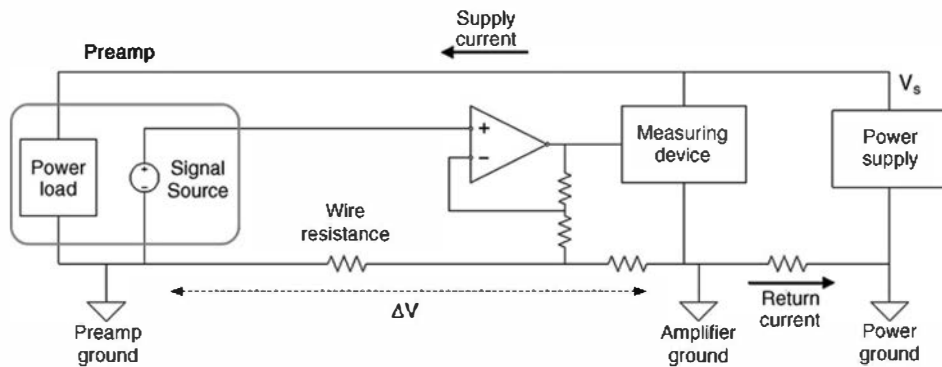
Figure 16.5 Sketch illustrating ground connections in a simple system. (Courtesy of R. Redus, Amptek, Inc.)
