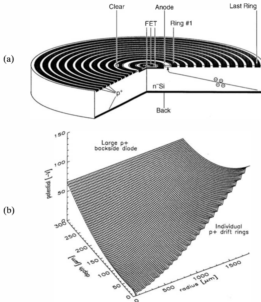
Figure 13.38 (a) Cross section through a cylindrical drift detector with an integrated JFET connected to the collecting anode. The nonstructured back surface of the detectors can provide a thin entrance window for weakly penetrating radiation. (b) Potential surface for electrons for the device of part (a). The central collecting anode is shown at the near corner of the surface. (From Lechner et al. 192 )
