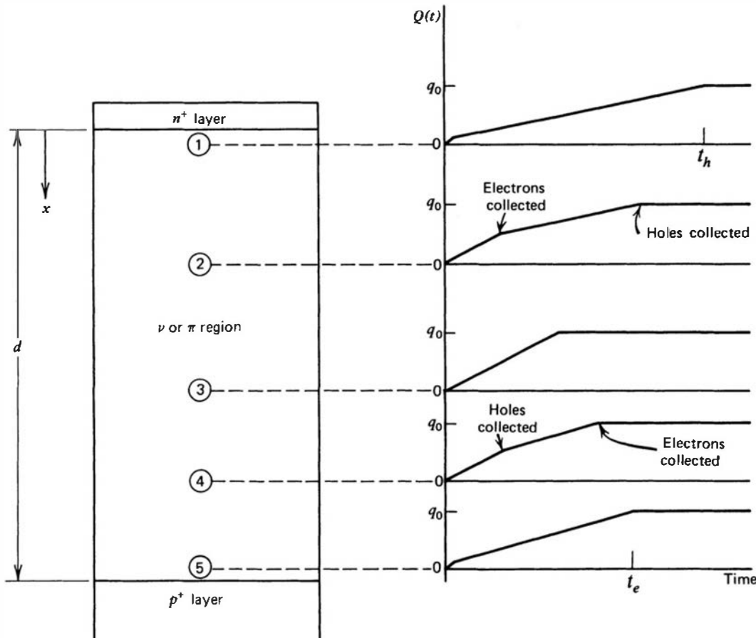
Figure 12.12 Shape of the leading edge of the output pulse Q(t) for various interaction points within the detector [from Eq. (12.20a)]. The initial slope of all pulses is the same, corresponding to the period when both electrons and holes are drifting. For point ①, electrons are collected very quickly and most of the rise corresponds to the drift of holes to the p^+ layer. The opposite is true for point ⑤. t_h and t_e are the assumed drift times for holes and electrons, respectively, across the entire thickness d .
