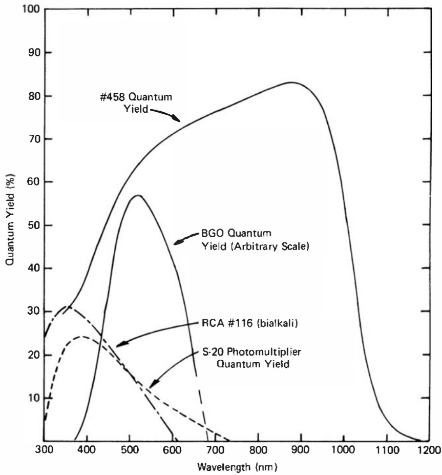
Figure 9.16 A comparison of the quantum efficiency of a silicon photodiode (labeled #458) with representative bialkali and S-20 photocathode quantum efficiencies. The emission spectrum from a BGO scintillator is shown for reference. (From Groom. 74 )
