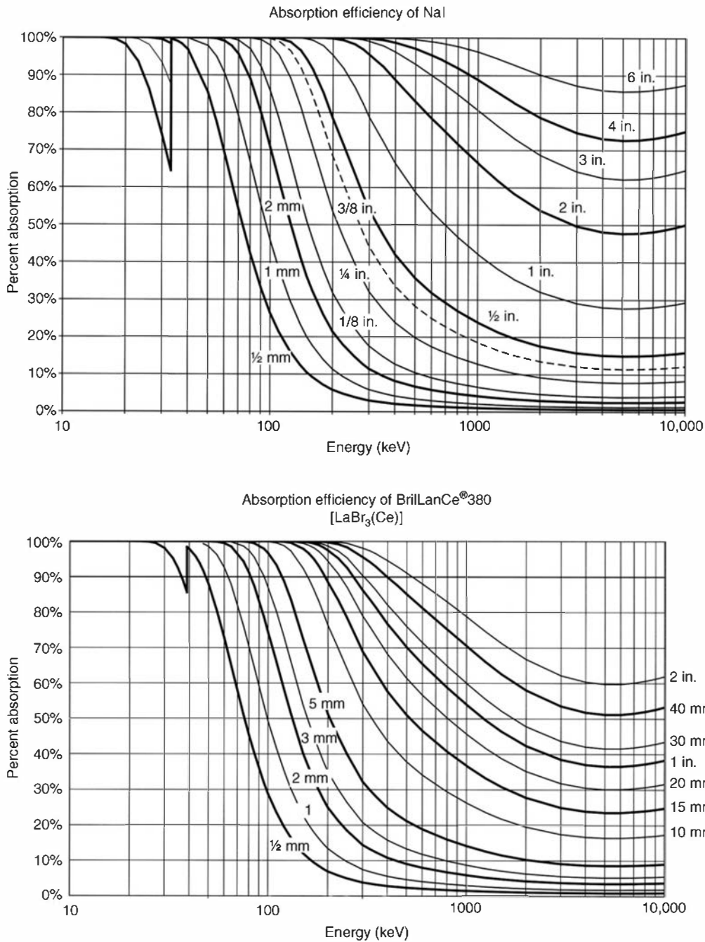
Figure 10.26 Plots of the intrinsic total efficiency for sodium iodide and lanthanum bromide scintillators of assorted thicknesses. The gamma rays are assumed to be normally incident to the surface. (From “Efficiency Calculations for Selected Scintillators,” Saint-Gobain Ceramics and Plastics, Inc.)
