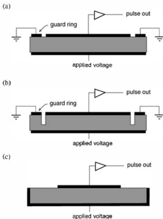
Figure 12.3 Three variants on the configuration of planar detectors. The electrodes are shown with exaggerated thickness as the solid black lines. (a) A narrow guard ring electrode protects the readout electrode from the effects of leakage current conducted across the cylindrical side surface of the semiconductor disk. (b) A groove is provided into the semiconductor volume to increase the surface area separating the guard ring and readout electrode. (c) A “wraparound” electrode is extended from one planar surface to also cover the side surface of the disk, and a small-diameter readout electrode fabricated on the opposite planar surface. The detector is normally oriented so that gamma or X-rays are incident on the surface shown at the bottom in this sketch.
