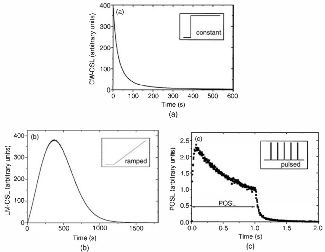
Figure 19.17 (a) CW-OSL obtained with a constant stimulation power (inset). The decay is due to the depopulation of trapped carriers during the readout. (b) LM-OSL in which the stimulation power is increased linearly with time (inset). (c) POSL obtained by monitoring the OSL emission between stimulation pulses in which each pulse width (inset) is shorter than the luminescence lifetime of the emitting center. The train of pulses in this example was 1 s long, and the drop in intensity over this period is again due to the depopulation of trapped carriers. Following the end of the pulses, the signal decays exponentially with the characteristic lifetime of the luminescence centers. (Courtesy of S. McKeever, Oklahoma State Univ.)
