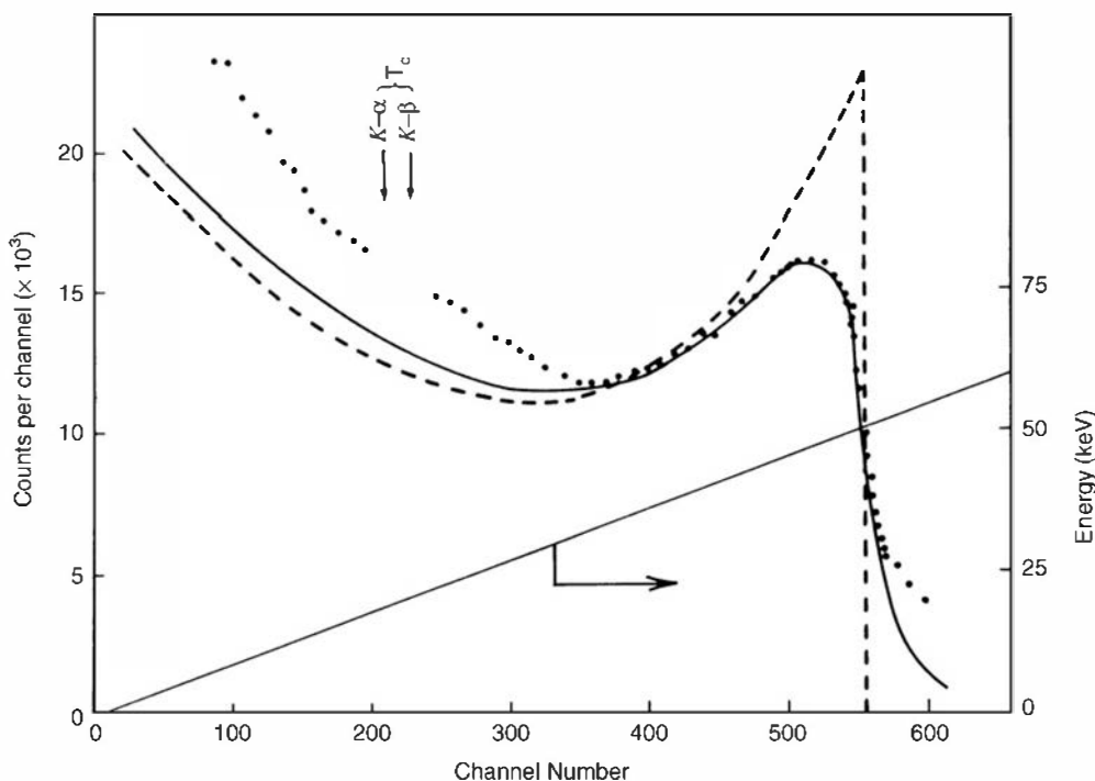
Figure 13.9 Calculated and observed shape of the Compton continuum for a 99m Tc source (140.5 keV). The dashed curve is predicted based on scattering of free electrons, whereas the solid curve is calculated taking into account the finite electron binding energy in silicon. The points are experimental data. (From Felsteiner et al. 24 )
