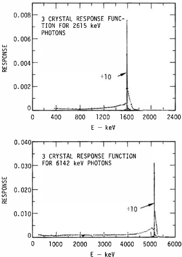
Figure 12.29 Response functions of a Ge(Li) crystal operated as a pair spectrometer in conjunction with two NaI(Tl) detectors. (From Stelts and Browne. 82 )
