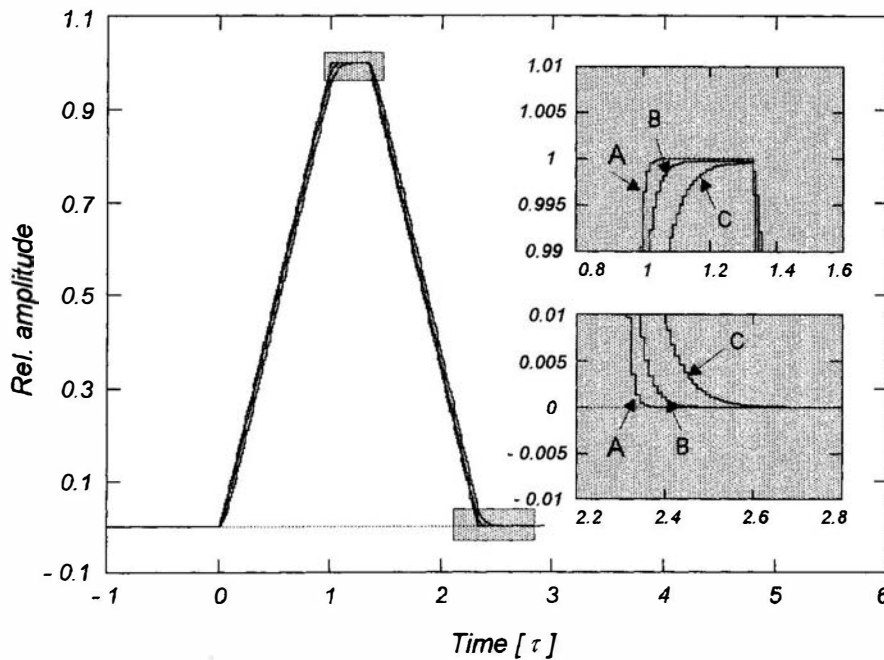
Figure 17.7 Effect of trapezoidal shaping of detector pulses with three different rise times that increase in the sequence A, B, and C. In the case shown, if the trapezoidal flat top is longer than the variation in rise time, the shaped pulses reach the same amplitude and ballistic deficit is avoided. (From Jordanov and Knoll. 3 )
