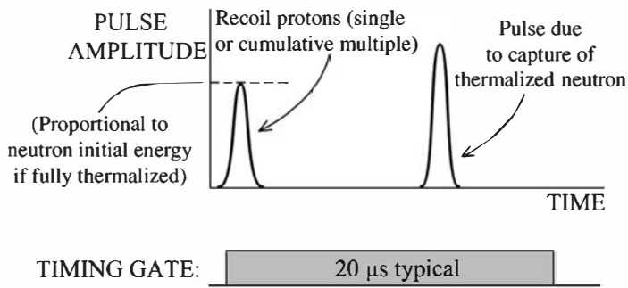
Figure 15.27 Sequence of two pulses expected from a capture-gated neutron spectrometer when the incident fast neutron is thermalized and captured.
