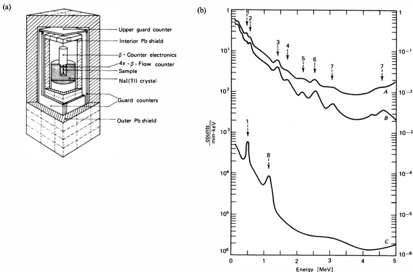
Figure 20.12 (a) A schematic view of a \beta - \gamma coincidence detector assembly, in which beta particles are detected by a split 4\pi flow counter, and the gamma rays by a surrounding well-type NaI(Tl) scintillator. Anticoincidence guard detectors are also employed. (b) Background spectra from the same detector assembly. A: NaI(Tl) spectrum without \beta - \gamma coincidence or anticoincidence shielding. B: Same, but with anticoincidence shielding. C: As in B, but with \beta - \gamma coincidence between the two detectors. Identified peaks probably correspond to 1—annihilation radiation; 2— ^{208}\text{Tl} ; 3— ^{40}\text{K} ; 4— ^{214}\text{Bi} , ^{212}\text{Bi} ; 5— ^{214}\text{Bi} , ^{212}\text{Bi} ; 6— ^{208}\text{Tl} ; 7—alpha particles from detector components; 8—not specifically identified. (From Roedel. 44 )
