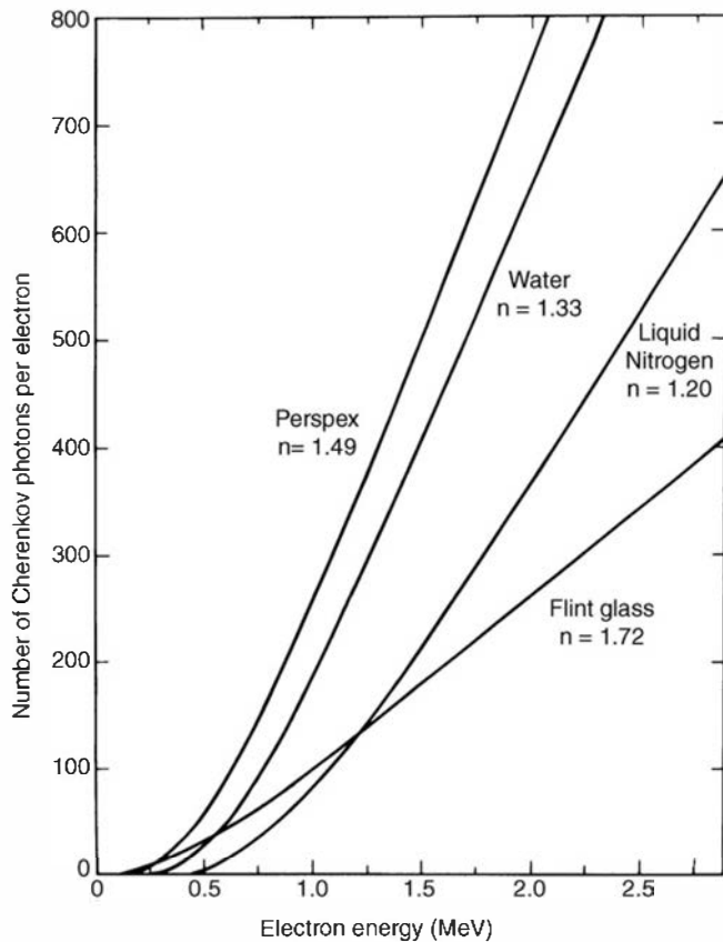
Figure 19.2 Calculated yield of Cherenkov photons in the 300–600 nm wavelength region for several detection media. (From Sowerby. 2 )
