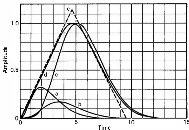
Figure 17.6 Synthesis of a near triangular waveform (curve d , normalized to unity) through the summation of active integrator output waveforms a , b , and c . Curve e is a symmetrical triangle for comparison. Time is in units of the initial differentiation time constant. (From Goulding et al. 1 )
