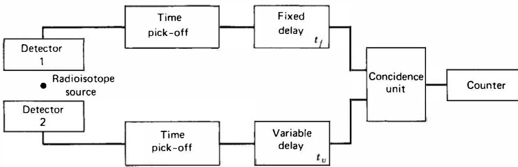
Figure 17.58 A simplified system to record coincidence-delay curves from a radioisotope source emitting coincident radiation.
