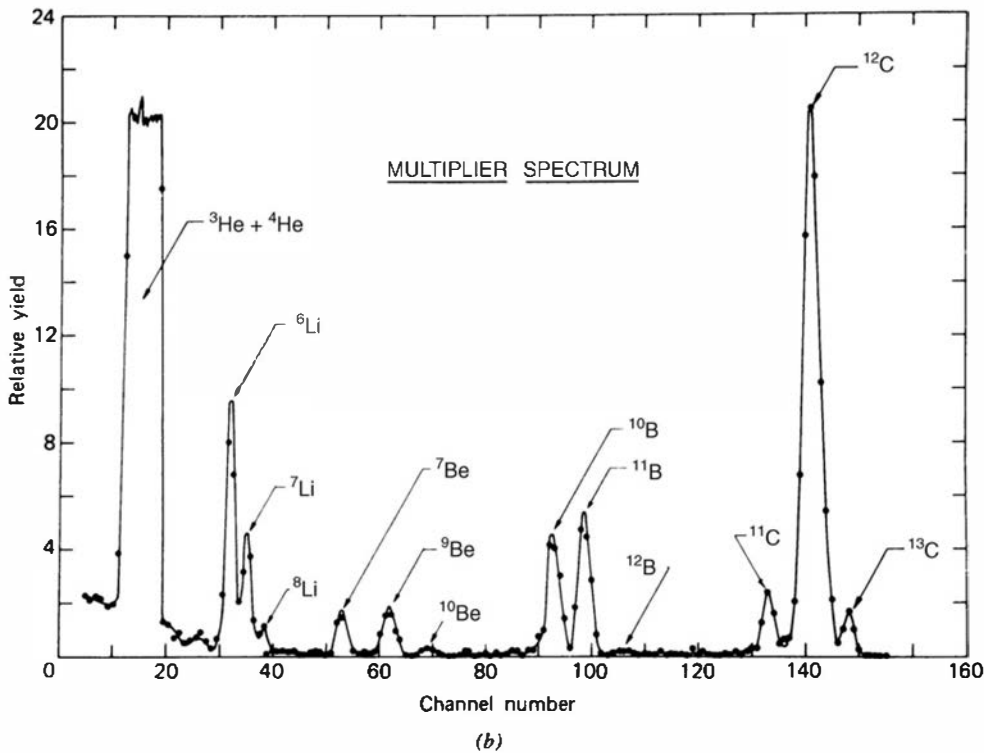
Figure 11.19 (a) A particle identifier arrangement consisting of tandem \Delta E and E detectors operated in coincidence. (b) Experimental spectrum obtained for the \Delta E \cdot E signal product for a mixture of different ions. (From Bromley, 115 )
