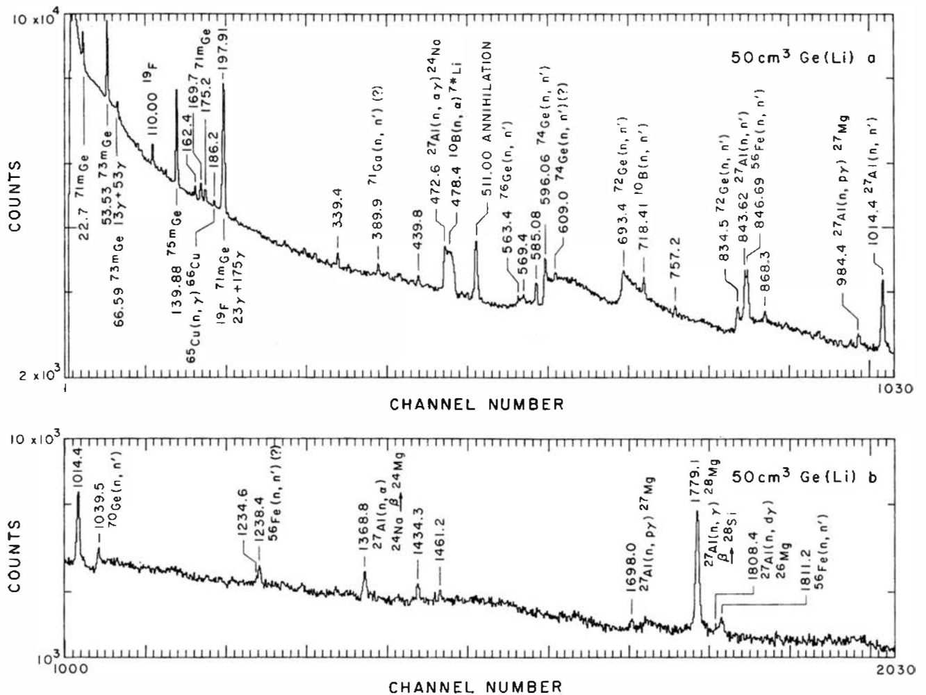
Figure 12.36 Prompt pulse height spectrum produced by fast neutron irradiation of a 50-cm 3 Ge(Li) detector. (From Bunting and Kraushaar. 127 )
