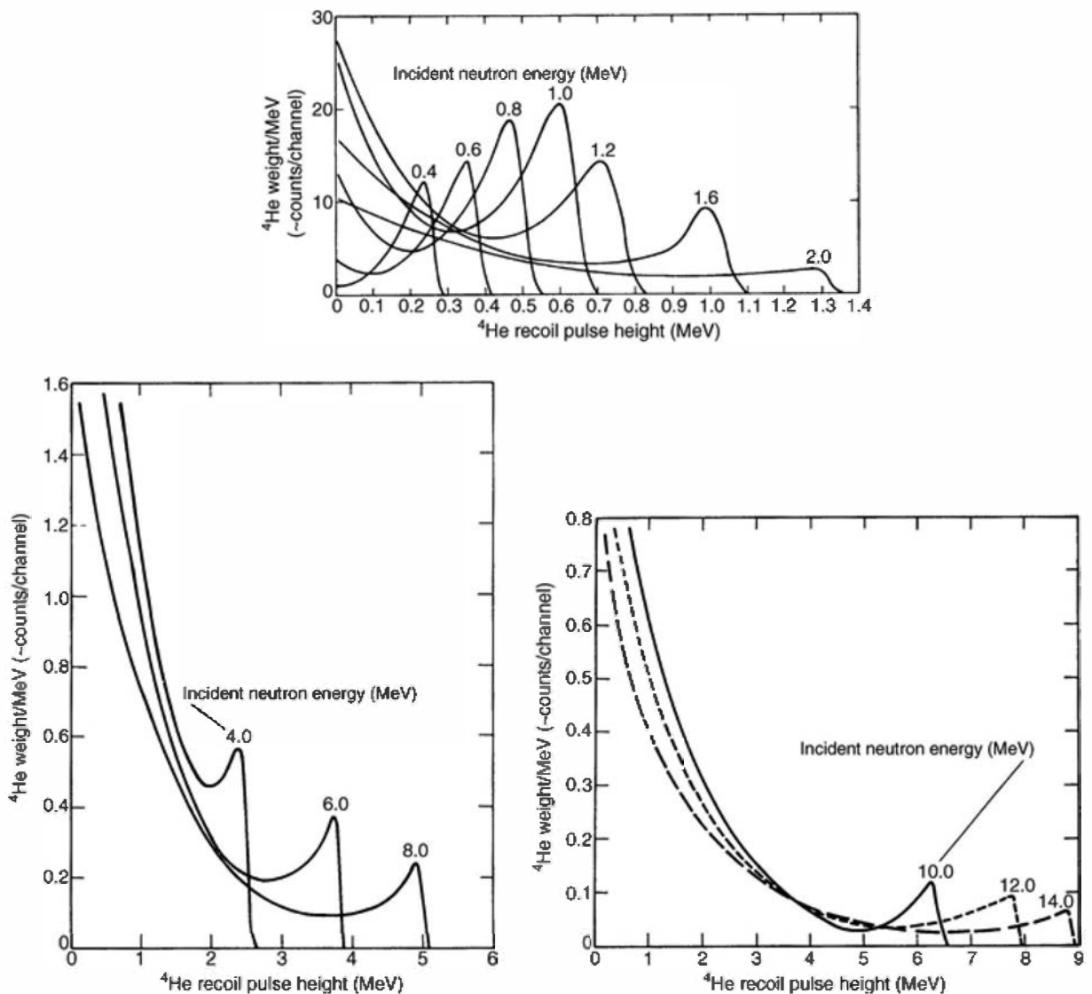
Figure 15.23 Calculated pulse height spectra for a recoil proportional counter filled with ^4\text{He} at 8 atm pressure. (From Atwater. 160 )
