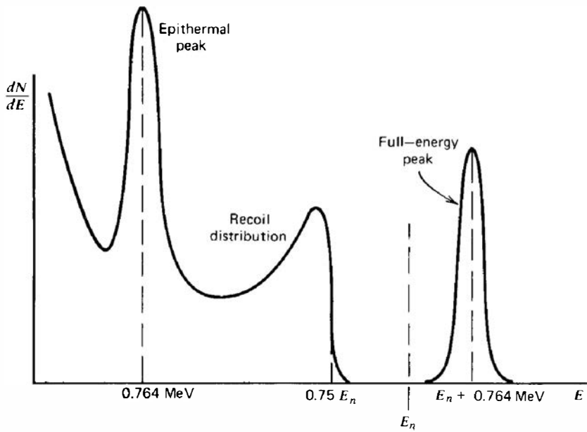
Figure 15.11 Idealized energy spectrum of charged particles expected from fast neutrons incident on a ^3\text{He} detector.
