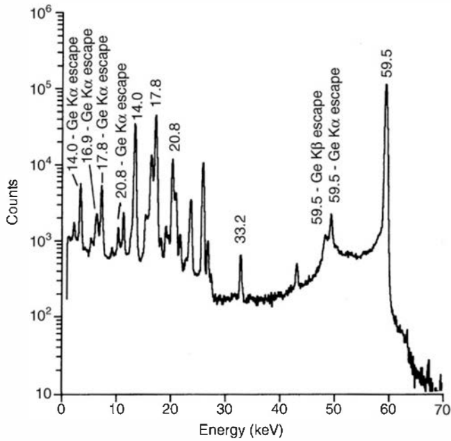
Figure 12.19 Pulse height spectrum taken from a ^{241}\text{Am} source with a 4-mm-thick planar HPGe detector. A number of the X-ray escape peaks are identified on the figure. (From Rossington et al. 59 )
