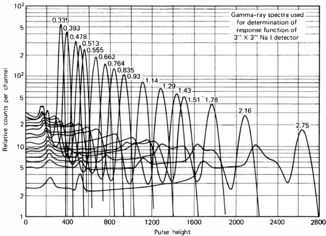
Figure 10.11 Response functions for a 7.62 cm × 7.62 cm cylindrical NaI(Tl) scintillator for gamma rays from 0.335 to 2.75 MeV. (From Heath. 5 )
