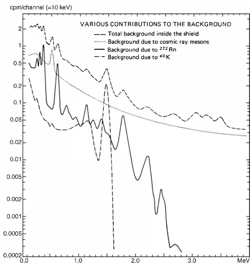
Figure 20.2 Various contributions to the background spectrum from a 7.62 cm × 7.62 cm NaI(Tl) scintillator inside a massive lead and borated paraffin shield. (From Stenberg and Olsson. 15 )
