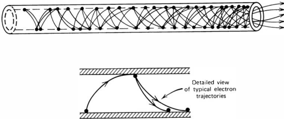
Figure 9.8 Continuous channel electron multiplier.
