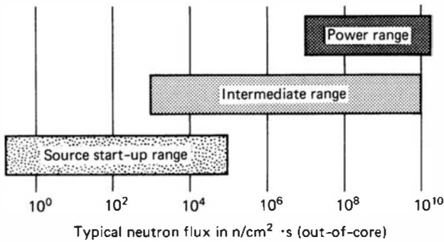
Figure 14.10 Typical ranges covered by out-of-core neutron detectors in a PWR.
