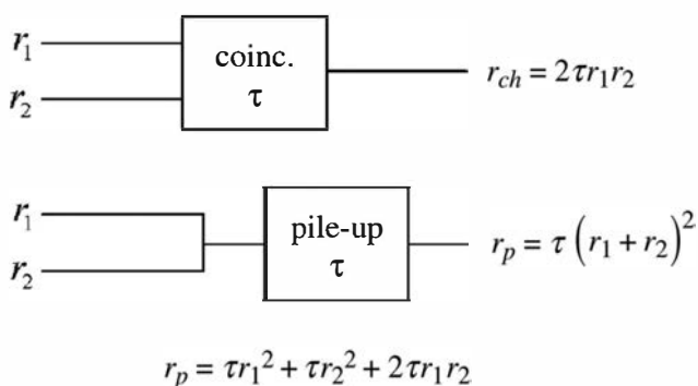
Figure 17.61 At the top, a coincidence unit with resolving time \tau results in a chance coincidence rate of 2\tau r_1 r_2 . In the bottom diagram, two input lines with equivalent singles rates are combined in a system with pile-up resolving time of \tau . Expansion of the resulting pile-up rate shows three components: pile-up of pulses in line 1, pile-up of pulses in line 2, and the pile-up involving pulses from opposite lines.
