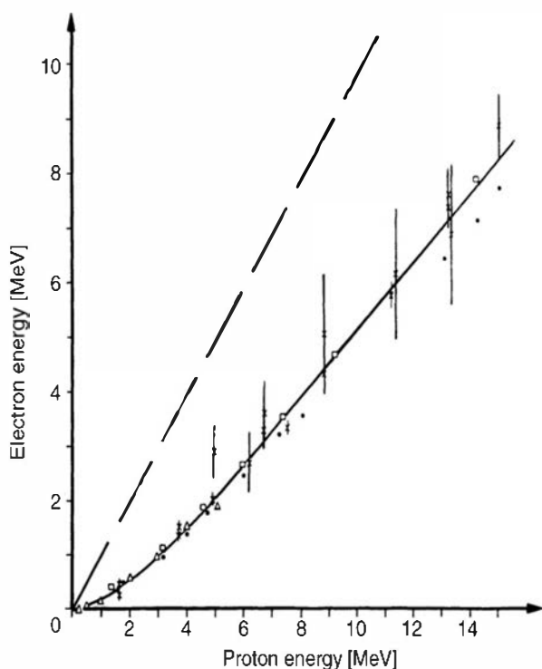
Figure 8.4 The light output (expressed in equivalent electron energy deposition) versus proton energy for liquid scintillator NE 213. The dashed line indicates the response to fast electrons. (Adapted from Maier and Nitschke. 46 )
