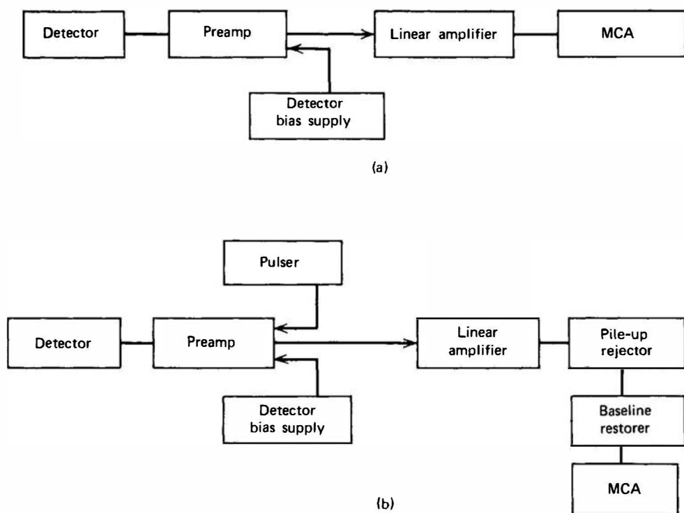
Figure 17.21 Signal chains for pulse height spectrometry. Part (a) shows a rudimentary system for noncritical applications, whereas system (b) includes some added functions that can improve performance for high-resolution detectors when operated at high pulse rates.
