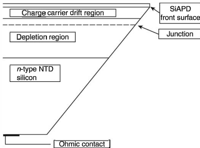
Figure 13.31 Cross section through an avalanche diode showing the beveled edge used to avoid surface breakdown. (From Farrel et al. 145 )
