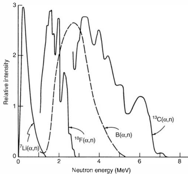
Figure 1.14 Neutron energy spectra from alternative ( \alpha, n ) sources. ( ^7\text{Li} data from Geiger and Van der Zwan, 28 and remainder from Lorch. 20 )
