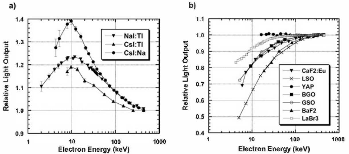
Figure 8.8 The relative scintillation response per unit energy deposited by fast electrons plotted as a function of their energy. The responses are normalized to unity at 445 keV. Perfectly proportional behavior would be a horizontal line passing through 1 on the vertical scale. The alkali halides included in part (a) show a peak in their response around 10 keV, whereas the scintillators plotted in part (b) show monotonically decreasing yield as the energy is lowered. (Plots courtesy of W. Moses of Lawrence Berkeley National Laboratory. Data derived from Ref. 87 and supplemented with prepublication data obtained using the SLYNCI facility at Lawrence Livermore National Laboratory.)
