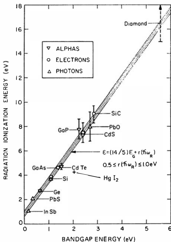
Figure 13.21 The average energy required to form one electron-hole pair ( \epsilon ) versus bandgap energy for a number of semiconductor materials. (From Klein. 48 )
