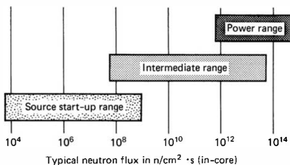
Figure 14.12 Typical ranges covered by in-core neutron detectors in a BWR.
