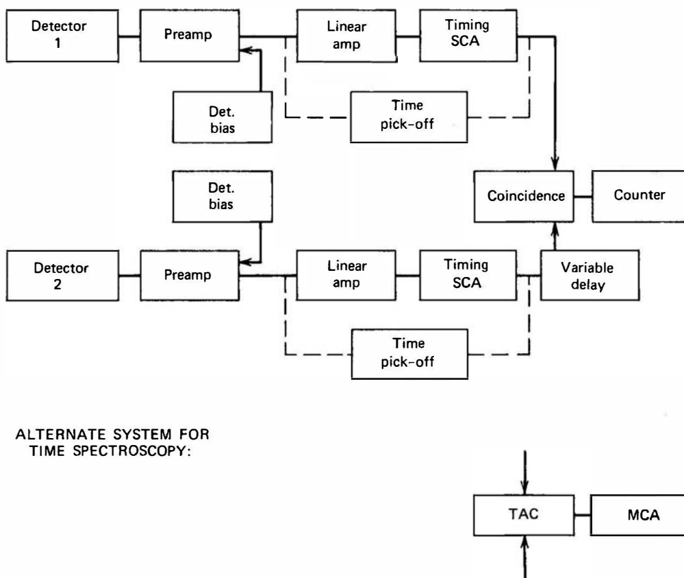
Figure 17.62 Basic modular system for twofold coincidence measurements. The use of a time pick-off in place of the linear amplifier and timing SCA, as indicated by the dashed lines, is warranted if no pulse amplitude selection is desired. An alternative arrangement for multi-channel time spectroscopy is indicated at the bottom, in which the coincidence unit and counter are replaced by a TAC and MCA.
