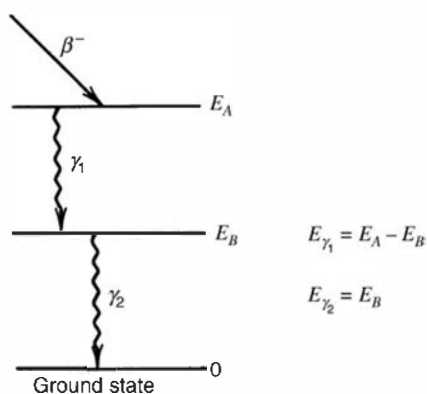
Figure 10.8 Simplified nuclear decay scheme, which can lead to summation effects in gamma spectra. Provided the intermediate state (at E_B ) is shortlived, \gamma_1 and \gamma_2 are emitted in virtual coincidence.
