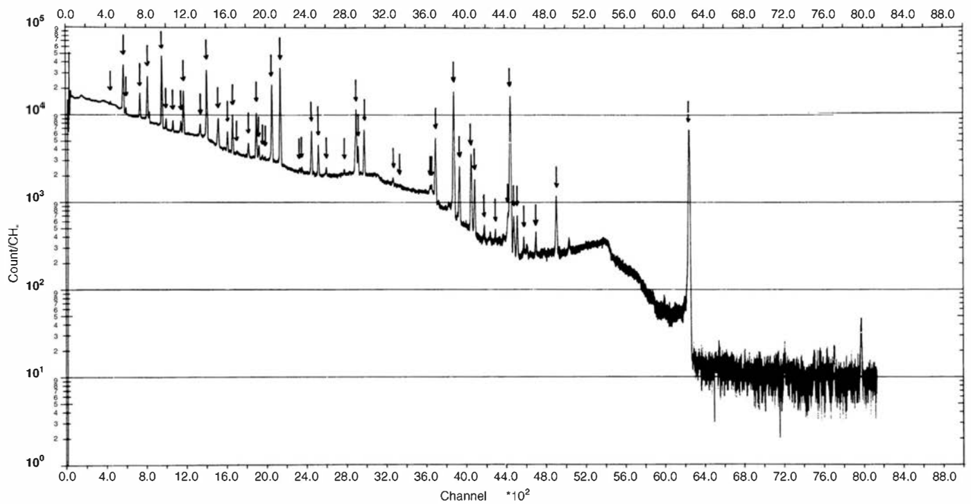
Figure 18.14 Results of a computerized peak search routine applied to a pulse height spectrum from a germanium gamma-ray spectrometer. Arrows indicate the locations of peaks found by the program. (From Sasamoto et al. 40 )
