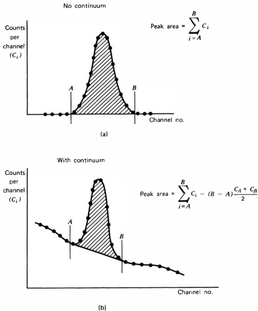
Figure 10.31 Methods of obtaining peak areas from multi-channel spectra. In part (a) the continuum under the peak present in part (b) is negligible.
