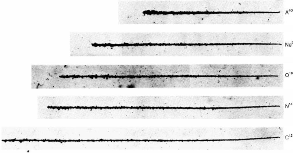
Figure 19.13 Tracks of fast heavy ions in Ilford K.5 nuclear emulsion. The ions are all incident from the left with initial energy of 10 MeV per nucleon. The track density is seen to decrease as the ion slows down and loses charge by electron pickup. (Photomicrographs courtesy of Prof. E. V. Benton, University of San Francisco.)
