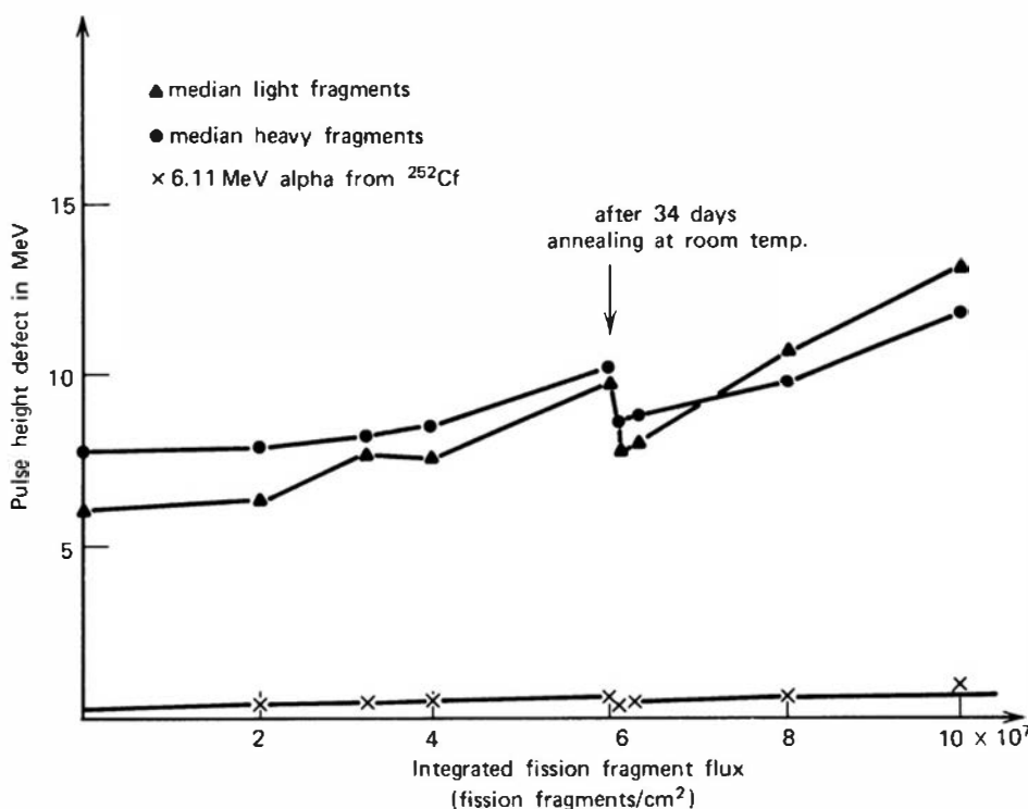
Figure 11.17 Dependence of measured pulse height defect versus fission fragment exposure for a heavy ion silicon detector. (From Bozorgmanesh. 93 )
