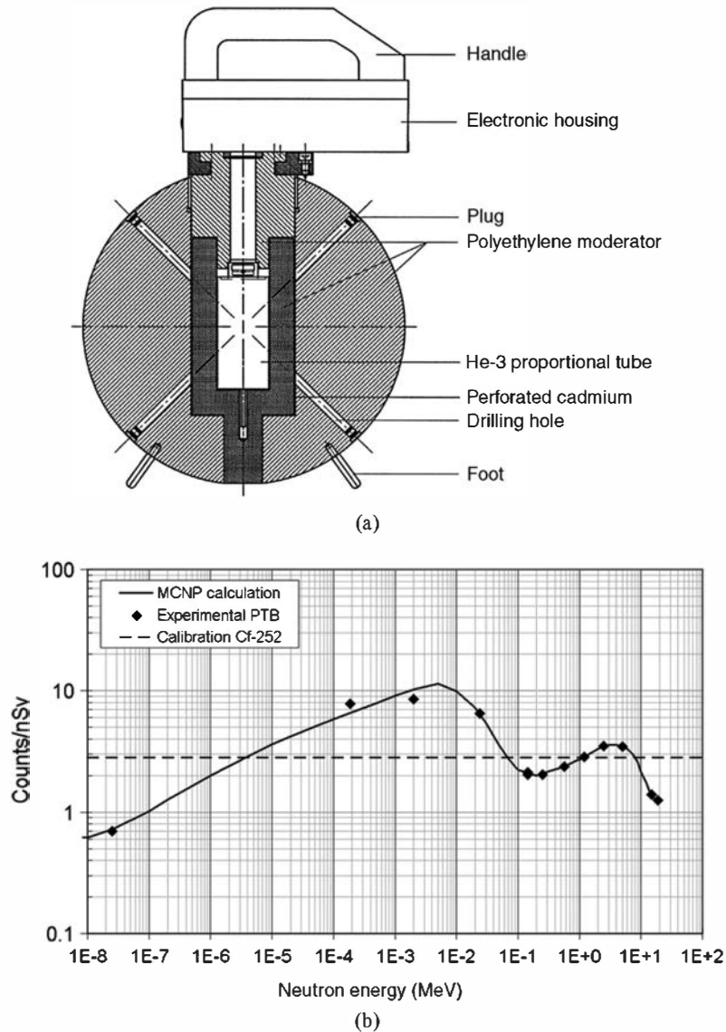
Figure 15.5 (a) Cross-sectional diagram of the Berthold LB 6411 spherical neutron dosimeter. The moderator has an external diameter of 25 cm and is 9.2 kg in weight. (b) The number of counts produced per unit ambient dose equivalent as a function of incident neutron energy for the instrument shown in part (a). The departure from a uniform response is quoted as plus or minus 30% from 50 keV to 10 MeV. Much larger departures are observed for lower and higher neutron energies. (From Klett and Burgkhardt. 23 )
