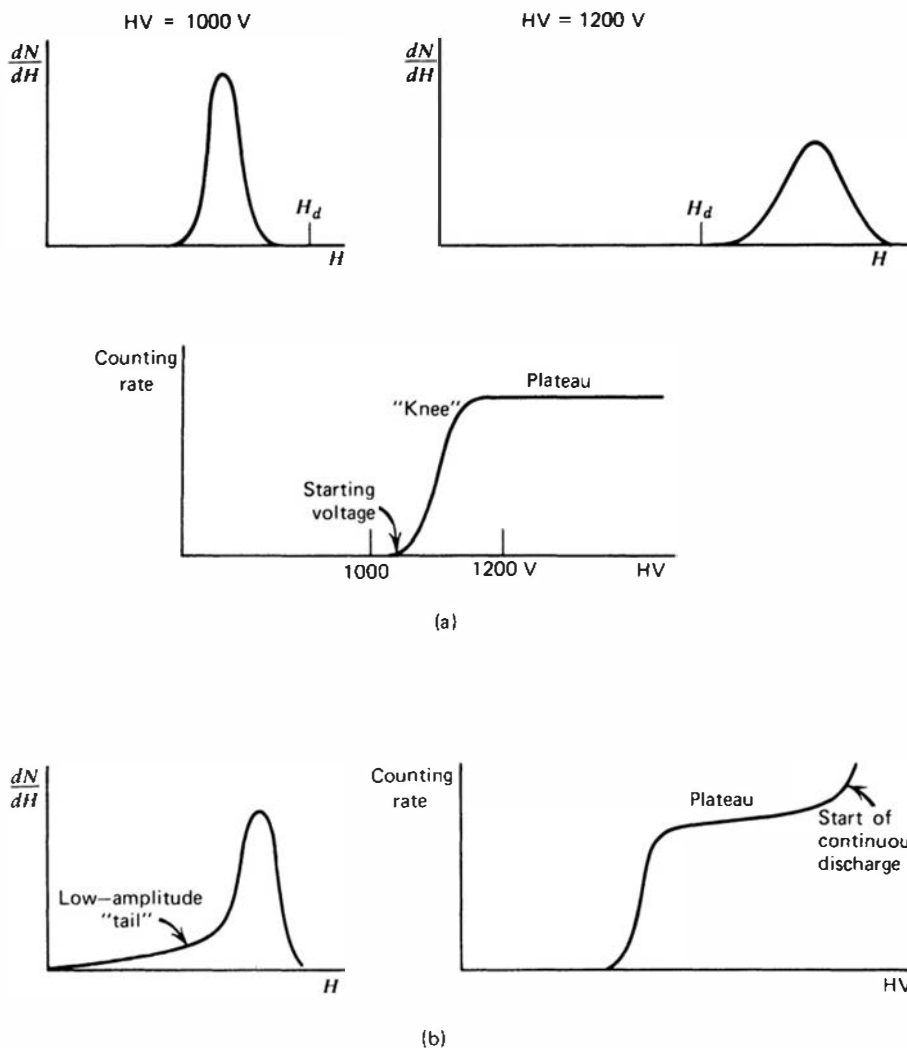
Figure 7.5 (a) The establishment of the counting plateau for a G-M tube. As the high voltage is varied in this example from 1000 to 1200 V, the output pulses change from falling below the counter threshold H_d to a situation in which all pulses are larger than H_d . (b) The low-amplitude tail on the pulse height spectrum at the left causes a finite slope of the plateau in the counting curve.
