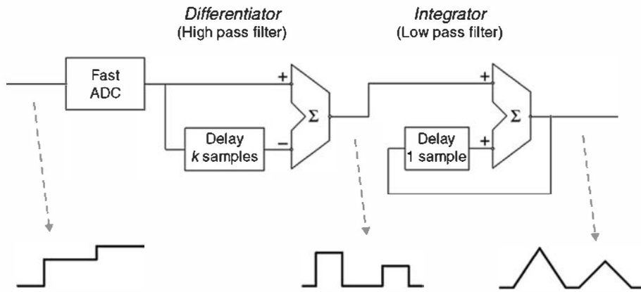
Figure 17.46 Example of a simple digital filter that produces a triangular-shaped pulse from a step input. (Courtesy of R. Redus, Amptek, Inc.)
