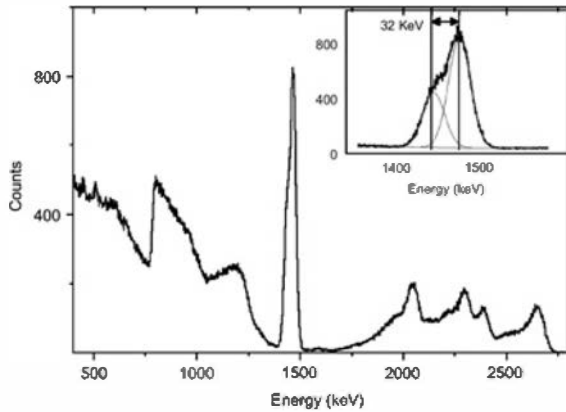
Figure 8.15 Intrinsic activity of \text{LaBr}_3 . The structure below 1.5 MeV is primarily associated with the decay of ^{138}\text{La} , while the structure above 1.5 MeV is produced by the decay chain of ^{227}\text{Ac} . The inset shows the peak structure around 1450 keV consisting of both intrinsic emissions and the natural external background from ^{40}\text{K} at 1461 keV. The intrinsic structure is associated with the cascade emission of a 1436 keV gamma ray and ^{138}\text{Ba} x-rays (about 32 keV); the presence of the 1436 keV peak indicates that a significant fraction of the X-rays are escaping without detection. With larger \text{LaBr}_3 crystals this feature will be suppressed and the sum peak at about 1468 keV will be more dominant. (From Nicolini et al. 215 )
