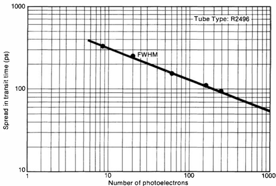
Figure 9.12 Measurements of the transit time spread observed from the PM tube shown in Fig. 9.11 as a function of the average number of photoelectrons generated per pulse. (From Kume et al. 33 )
