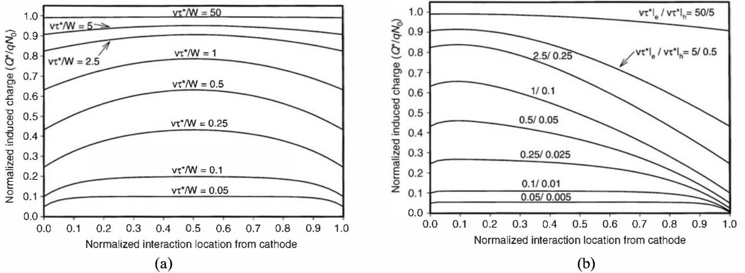
Figure 13.24 (a) Relative position-dependent charge collection for cases in which hole and electron transport properties are identical. Various values of v\tau^*/W are assumed to show the dependence. (b) Same plot as above, but for cases in which the electron carrier extraction factor is always 10 times greater than that for holes.
