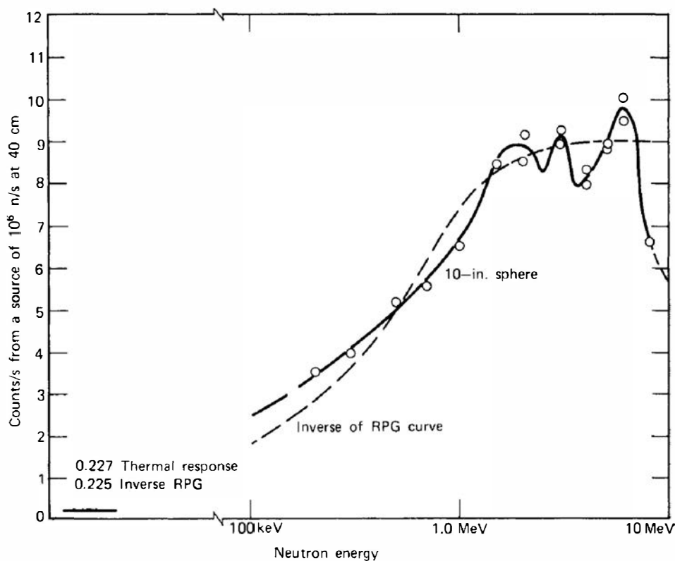
Figure 15.3 Sensitivity of a 10-in. (25.4 cm) diameter moderating sphere surrounding a 4 mm × 4 mm LiI scintillator. Also shown is the relative dose per neutron labeled “inverse of RPG curve.” (From Hankins. 17 )
