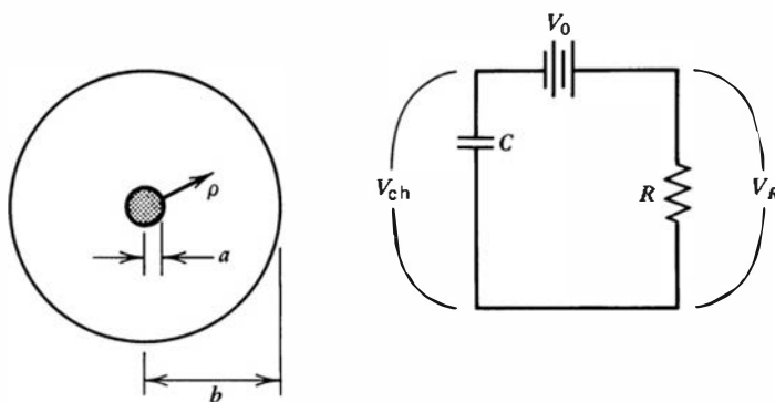
Figure 6.15 On the left is shown a cross-section of the cylindrical geometry used in deriving the pulse shape induced by a single avalanche. The equivalent circuit across which the signal is developed is at the right. There C represents the capacitance of the detector and associated wiring, V_R is the signal voltage developed across the load resistance R , and V_{ch} is the voltage remaining across the detector.
