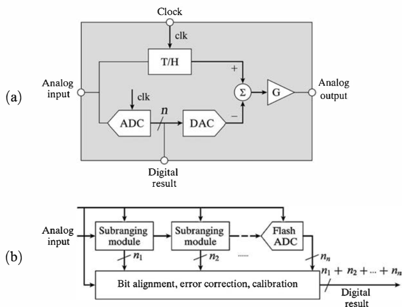
Figure 17.44 (a) The elements of a single subranging stage or module. T/H is a track-hold circuit, ADC is a flash ADC, DAC is a digital-to-analog converter, \Sigma is an analog summing unit, and G represents the gain of an analog amplifier. (b) The combination of multiple subranging modules in a fast pipelined ADC. (Courtesy of V. Jordanov, Yantel LLC.)
