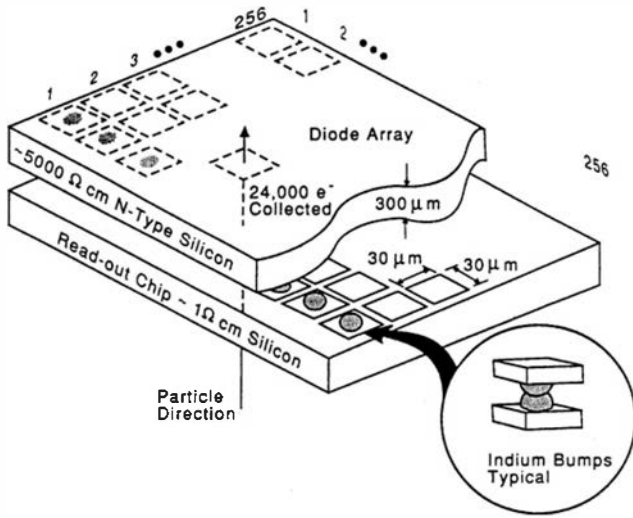
Figure 13.36 A “hybrid” pixel detector consisting of separate detector and electronics chips connected through indium bump bonds. (From Hallewell. 180 )
