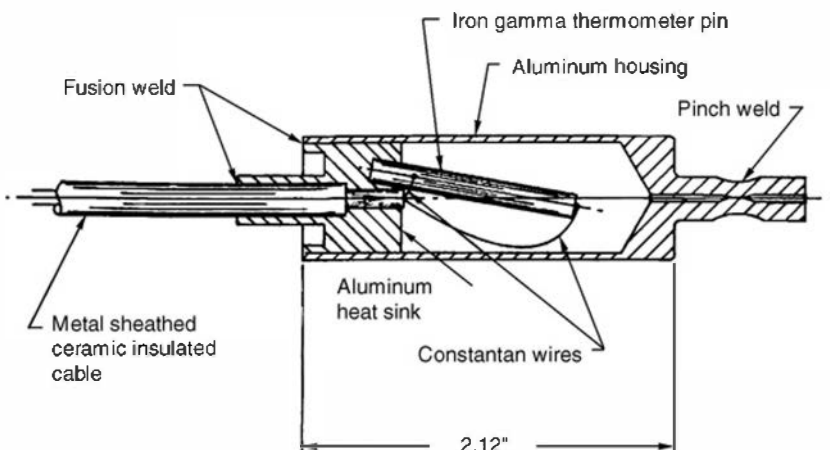
Figure 14.19 Single pin gamma thermometer. (From Stutheit. 115 )
