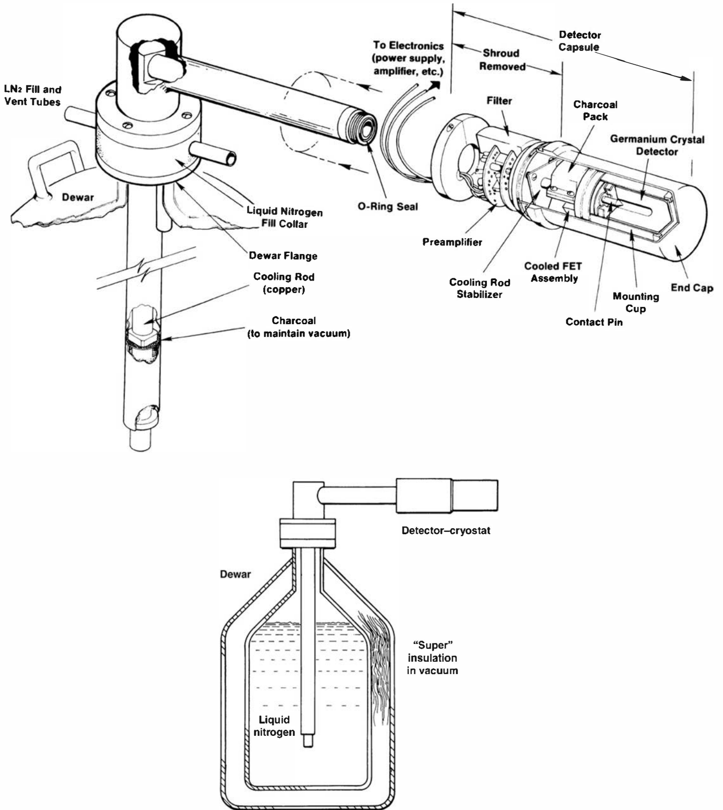
Figure 12.7 Diagram showing the location of a HPGe detector within its vacuum capsule. In this design, the capsule can be connected, without using vacuum pumps, to a variety of cryostats or cryostat-dewar assemblies. The example shown is the common horizontal configuration of the cryostat above the liquid nitrogen dewar (see inset). (Courtesy of M. Martini, EG & G ORTEC, Oak Ridge, TN.)
