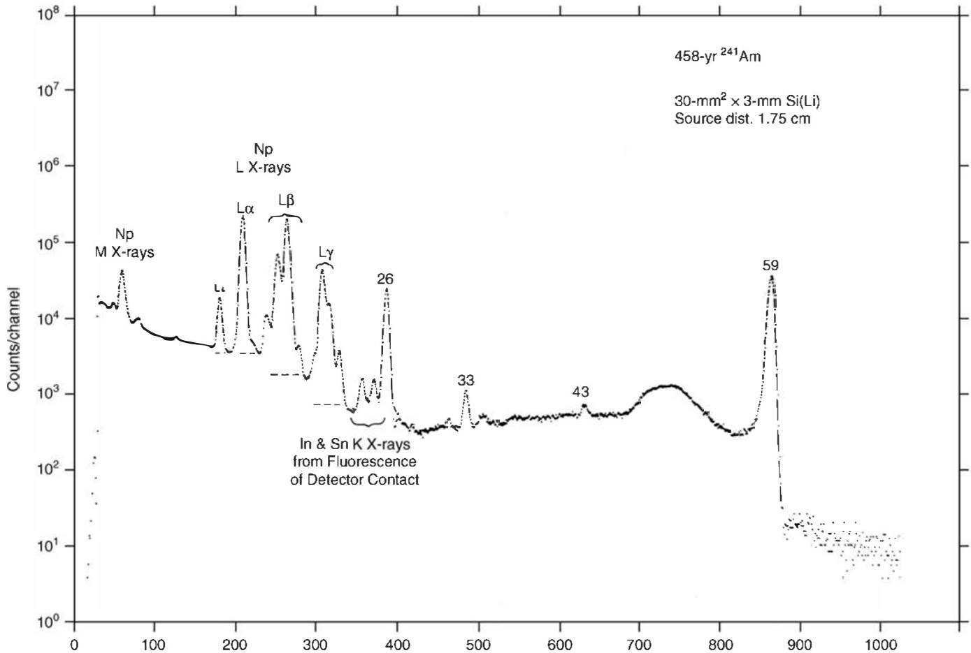
Figure 13.13 Photon spectrum from ^{241}\text{Am} obtained using a 30\text{ mm}^2 \times 3\text{ mm} Si(Li) detector. (From Gehrke and Lokken. 32 )
