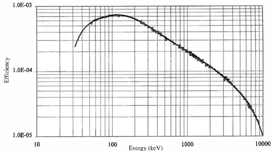
Figure 12.33 The points shown are measured full-energy peak efficiency values for a 25% relative efficiency n -type germanium detector. The cryostat had a 0.5-mm-thick aluminum entrance window. The points at lower energies were obtained using standard radioisotope calibration sources, whereas neutron-induced capture gamma rays provided the upper energy values. The solid line is a 9-parameter analytical fit to all the points using a function of the form given in Eq. (12.32). (From Kis et al. 107 )
