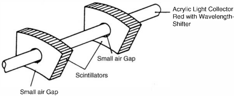
Figure 8.25 Sections of two slab scintillators are shown coupled to a common light pipe loaded with wavelength shifter. Light passing across the air gap and entering the pipe can be absorbed, re-radiated, and guided to the ends of the rod. (From Eckardt et al. 317 )
