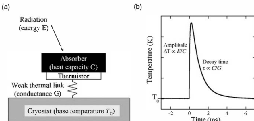
Figure 19.7 Schematic of a microcalorimeter (a), and typical gamma-ray pulse in response to a single 60 keV photon (b). (Courtesy of S. Friedrich, Lawrence Livermore National Laboratory.)
