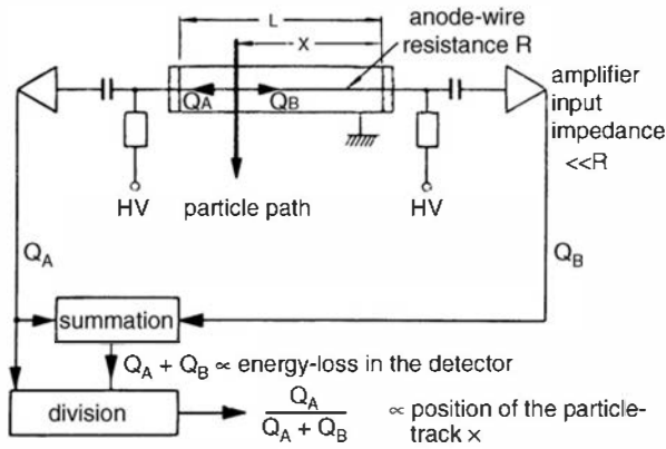
Figure 6.20 Position localization in proportional counters using the charge-division method. (From Fischer. 102 )
