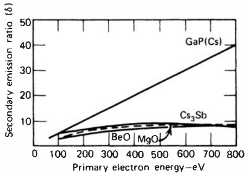
Figure 9.3 Variation of the secondary emission yield with primary electron energy for standard dynode materials (lower three curves) and an NEA material [GaP(Cs)]. (From Krall et al. 10 )
