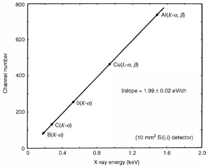
Figure 13.10 Experimentally determined linearity between pulse height and X-ray energy for a Si(Li) detector. (From Musket. 25 )
