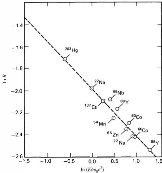
Figure 10.21 Experimentally measured resolution R from a NaI(Tl) scintillation detector for various gamma-ray energies E . (From Beattie and Byrne. 21 )
