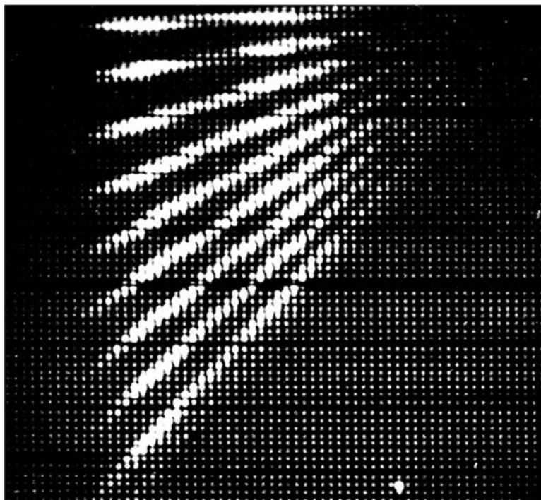
Figure 13.34 A two-parameter display of events recorded from a position-sensitive detector of the type shown in Fig. 13.33. The E signal amplitude is displayed along the horizontal axis and the P signal along the vertical axis. A collimator with nine equidistant slits was placed in front of the detector. Incident particles were fission fragments from ^{252}\text{Cf} . (From Kaufman et al. 162 )
