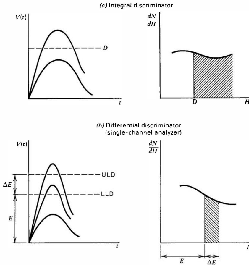
Figure 17.18 (a) The function of an integral discriminator. Of the two input pulses shown, only the larger clears the discrimination level D and produces a logic pulse output. The effect is to select only the area to the right of the amplitude D in the differential pulse height spectrum. (b) The function of a differential discriminator or single-channel analyzer. For the three input pulses shown, only the intermediate amplitude lies within the acceptance window and leads to an output logic pulse. In the pulse height spectrum, only the pulses falling within the cross-hatched area are accepted.
