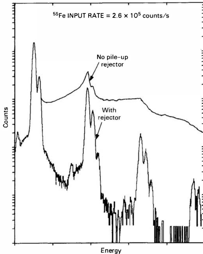
Figure 17.31 Pulse height spectra recorded with and without a pile-up rejector. The true event rate n was 2.6 \times 10^5/\text{s} and the rejector resolution time \tau was 300 ns. Note that the contributions to the spectrum from pile-up are greatly reduced by the rejector, while the numbers of counts in the primary peaks (free of pile-up) are unaffected. (From Goulding and Landis. 35 )
